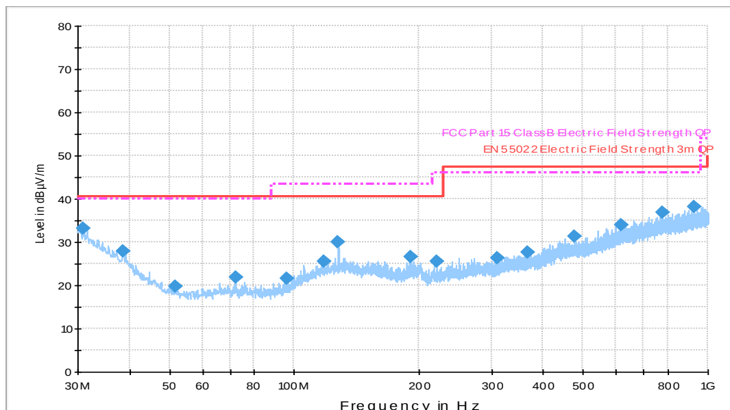
Plot 1: Unintentional Radiated Emissions, IC/FCC Class B, Receive Mode -3m
