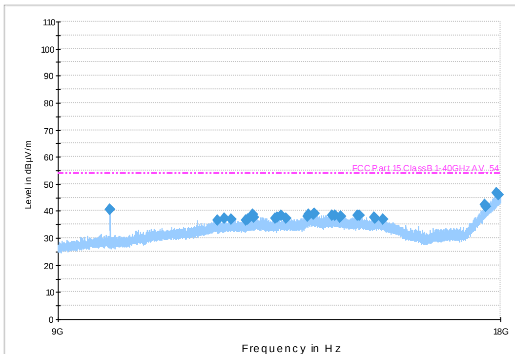
Plot 6: Intentional Radiated Emissions, 9GHz-18GHz, Tx Mode, Mid Channel -3m
