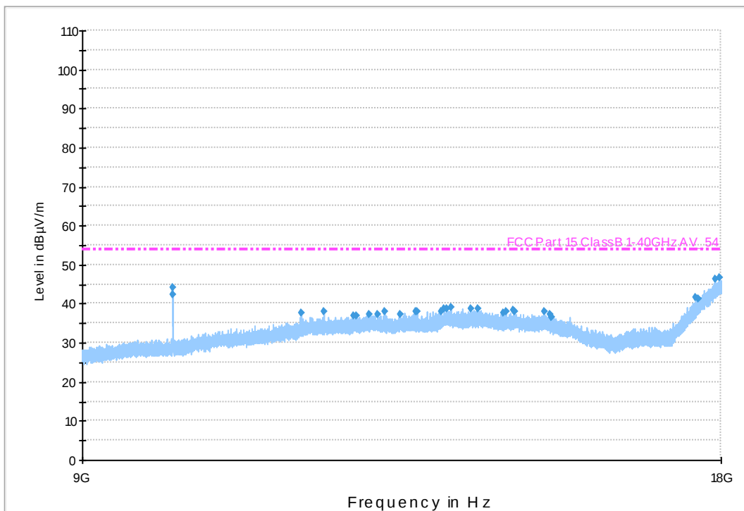
Plot 8: Intentional Radiated Emissions, 9GHz-18GHz, TX Mode, High Channel -3m
