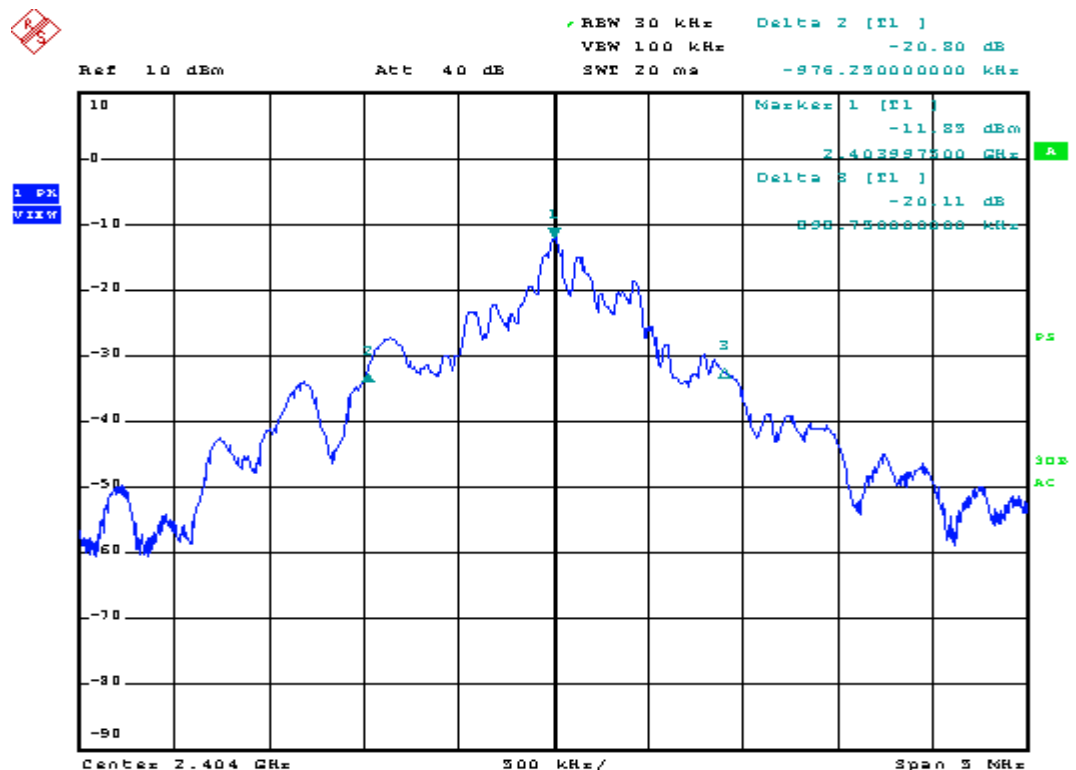
Plot 10: 20dB Bandwidth at LOW Frequency – 1875 kHz
