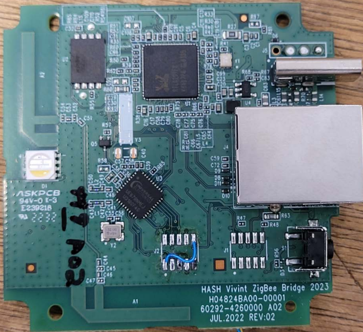
Bottom View of the PCB - View #1
