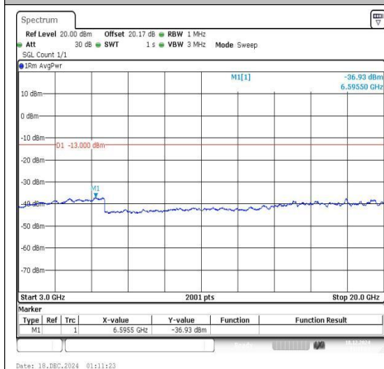
Band4_5MHz_QPSK_20375_1RB#0_3000~2000_0_3000~20000
