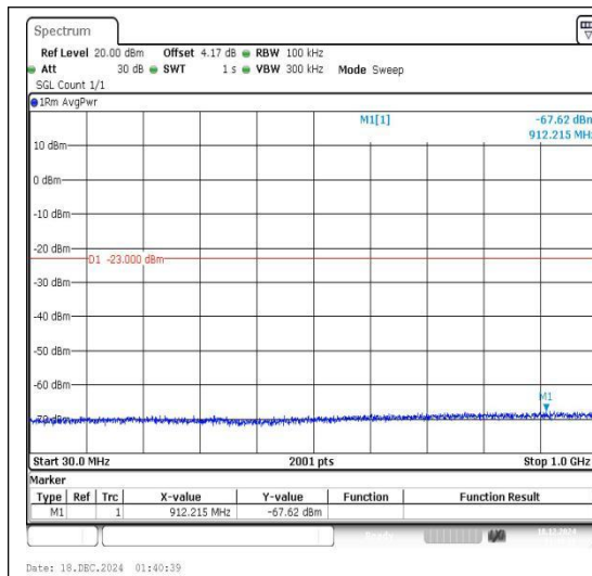
Band4_10MHz_QPSK_20175_1RB#0_30~1000_30~1000
