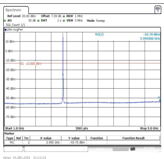
Band4_5MHz_QPSK_20375_1RB#0_1000~3000_1000~3000
