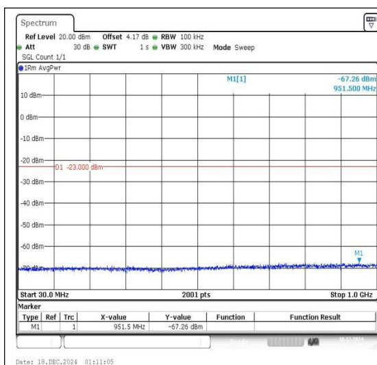
Band4_5MHz_QPSK_20375_1RB#0_30~1000_3 0~1000
