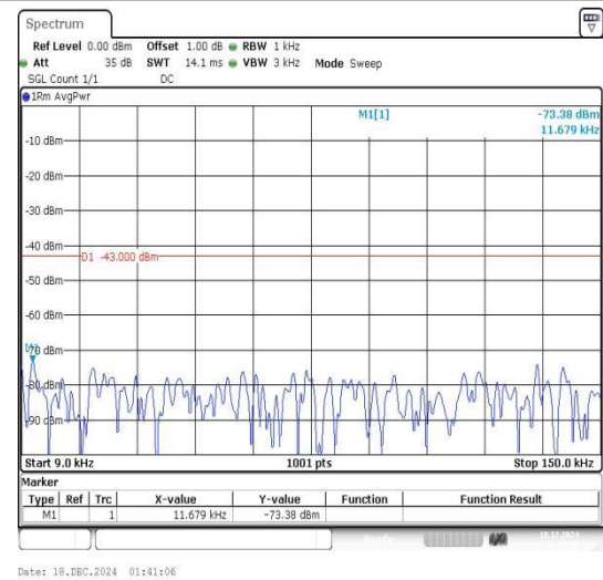
Band4_10MHz_16QAM_20175_1RB#0_0.009~0.15_5_0.009~0.15
