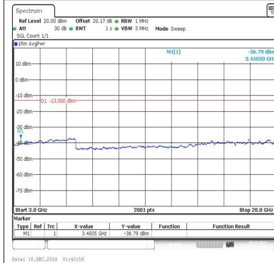
Band4_10MHz_QPSK_20175_1RB#0_3000~20000_3000~20000
