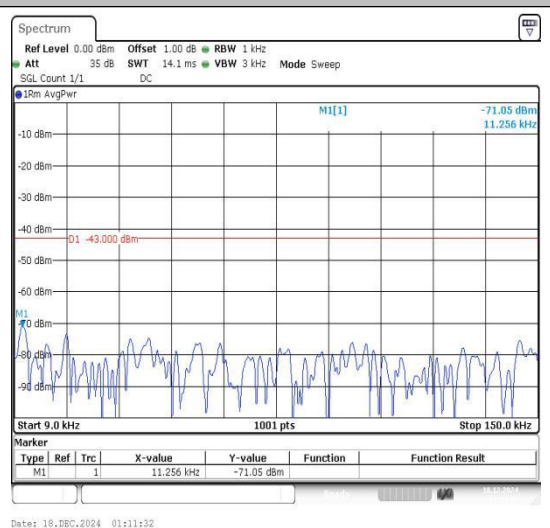
Band4_5MHz_16QAM_20375_1RB#0_0.009~0.15_0.009~0.15
