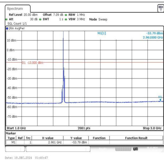
Band4_10MHz_QPSK_20175_1RB#0_1000~3000_1000~3000
