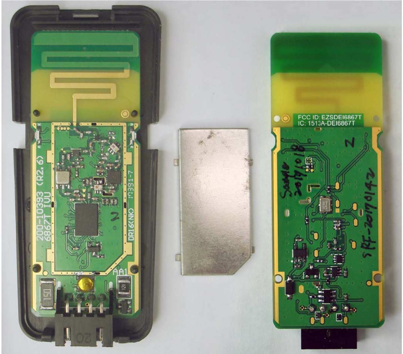
PCB top (left) and bottom (right) views. The shielding (center) is normally installed on the PCB top side.
