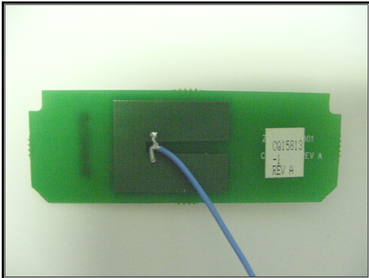
PHOTOGRAPH 43: ZPR POD (CQ15813-1) ANTENNA FRONT VIEW
