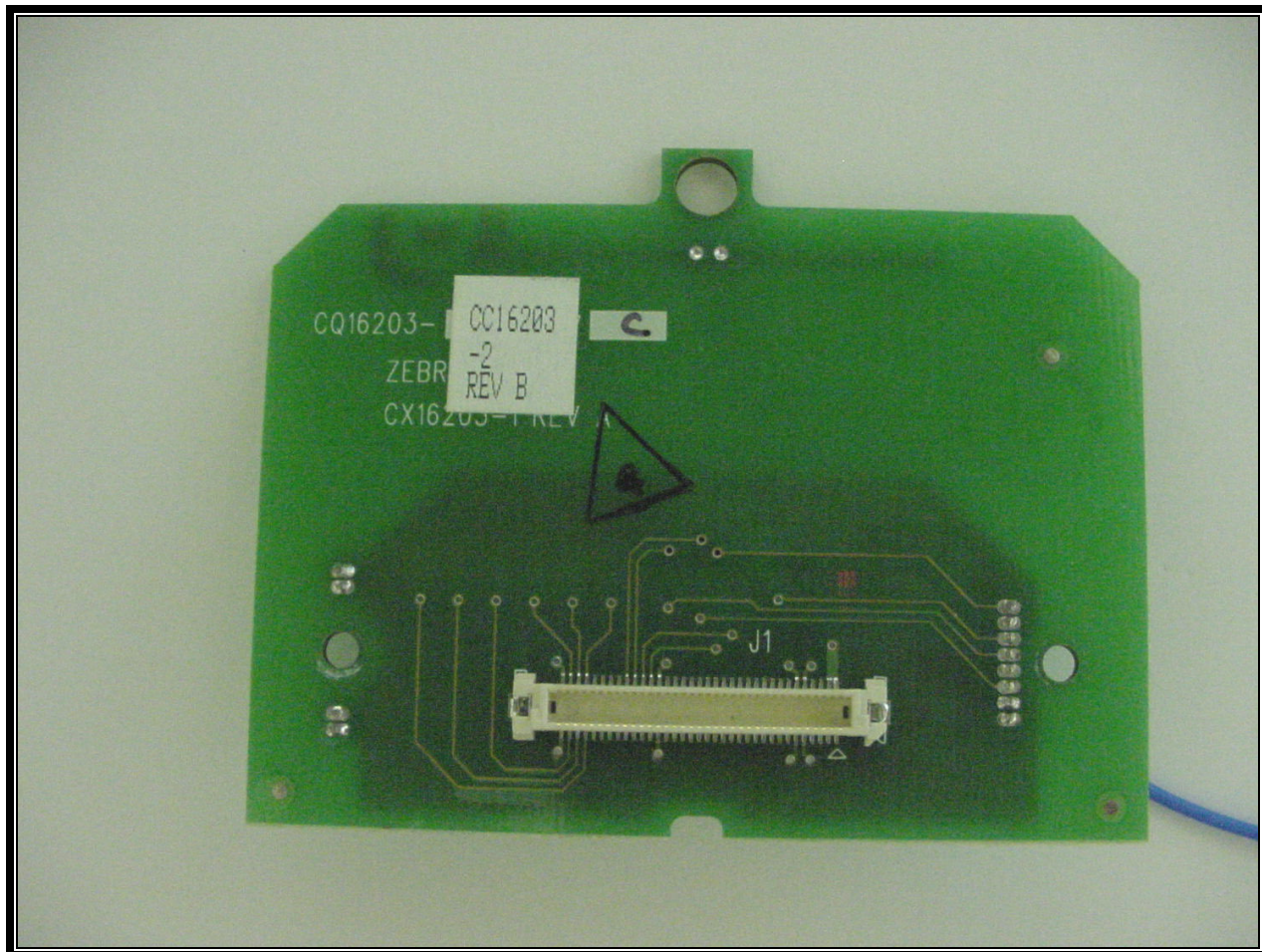
PHOTOGRAPH 40: QL FAMILY (CC16203-2) ANTENNA BACK VIEW
