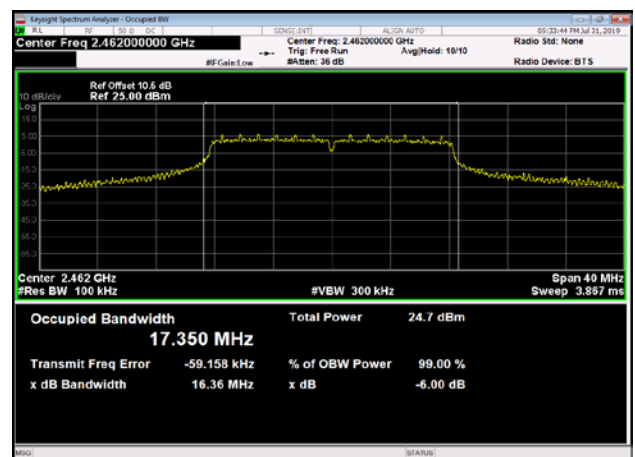
6dB Bandwidth-802.11g,2462MHz
