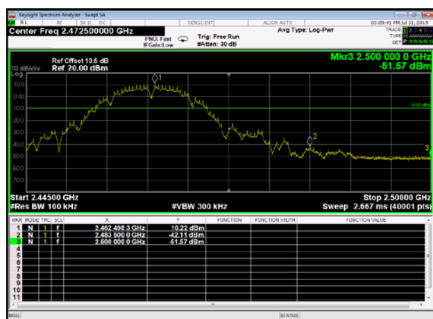
,Plot 2,Band Edge-802.11b,2462MHz
