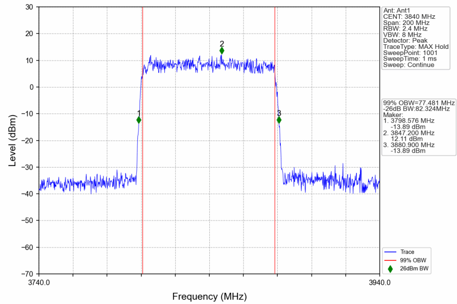
n77a_30kHz_SISO_NTNV_80MHz_DFT-s-OFDM_256_QAM_3840MHz_Outer_Full
