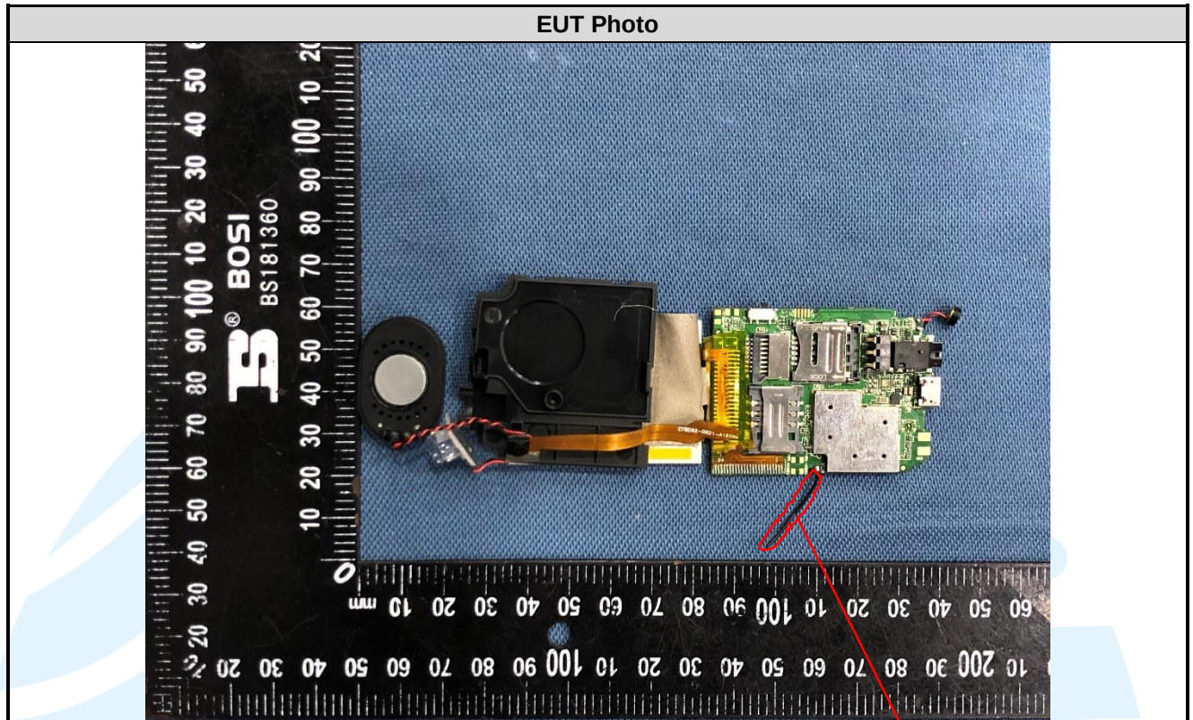
BT Antenna
