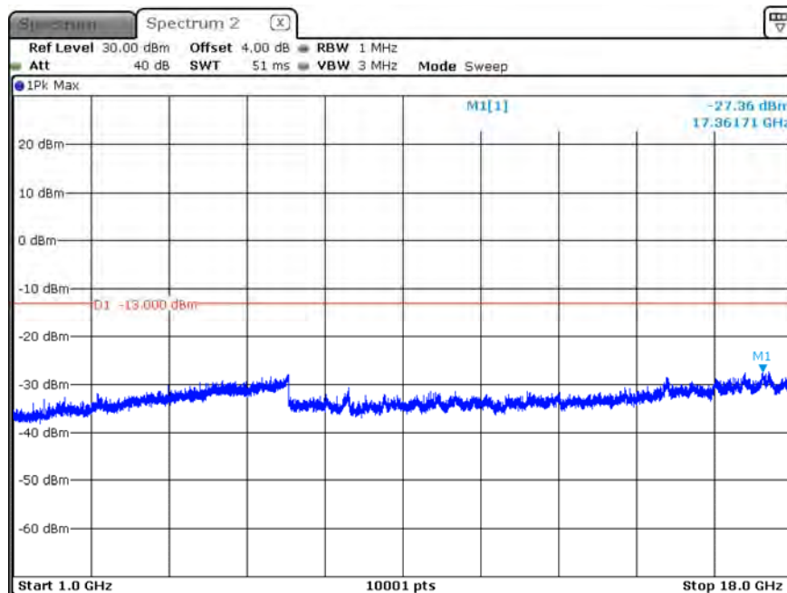
B12_CH23173_1.4M_1RB5_QPSK_Above 1G
