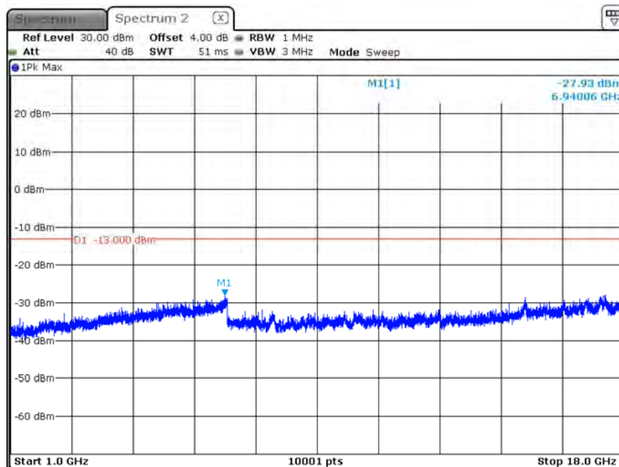
B12_CH23025_3M_1RB0_16-QAM_Above 1G
