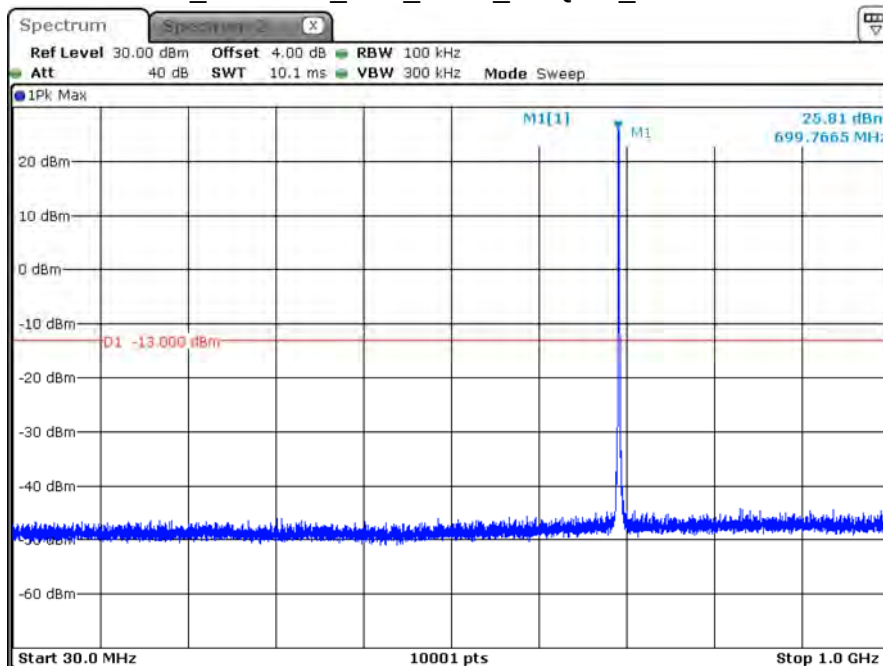
B12_CH23060_10M_1RB0_16-QAM_Below 1G
