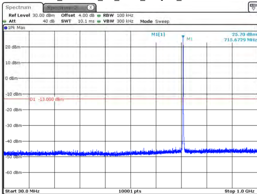
B12_CH23165_3M_1RB5_16-QAM_Below 1G
