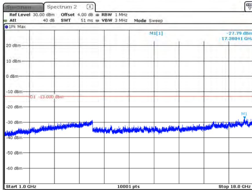
B12_CH23095_3M_1RB0_16-QAM_Above 1G
