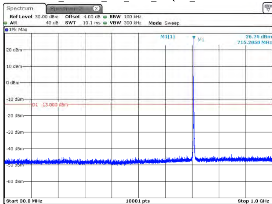
B12_CH23130_10M_1RB5_16-QAM_Below 1G
