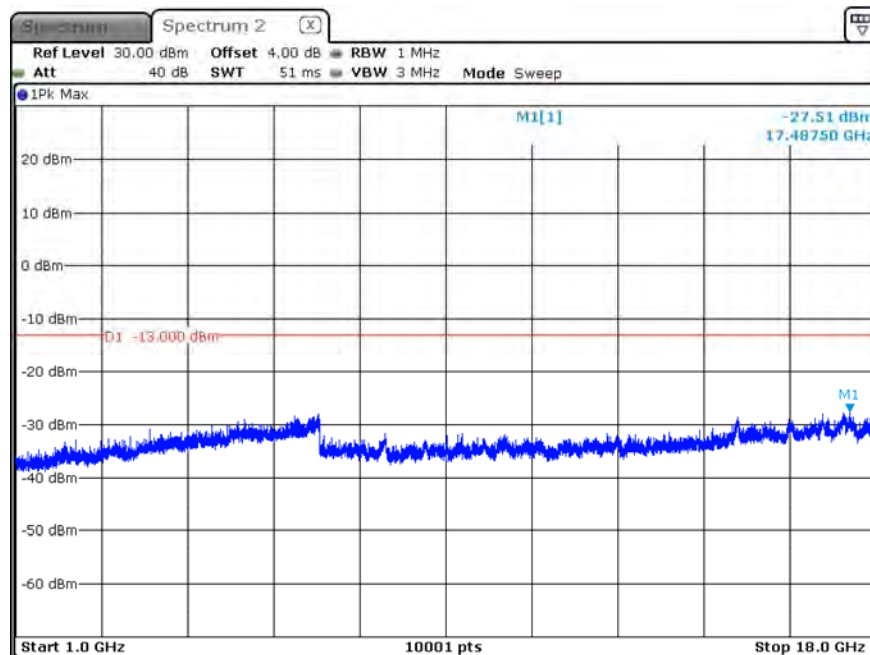
B12_CH23095_1.4M_1RB0_QPSK_Above 1G
