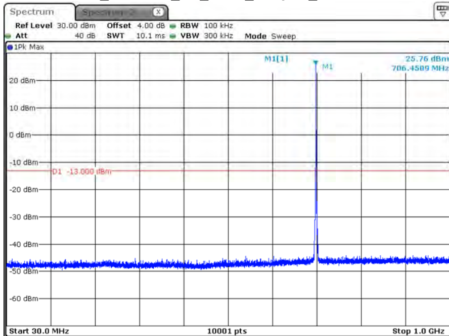
B12_CH23095_3M_1RB0_16-QAM_Below 1G
