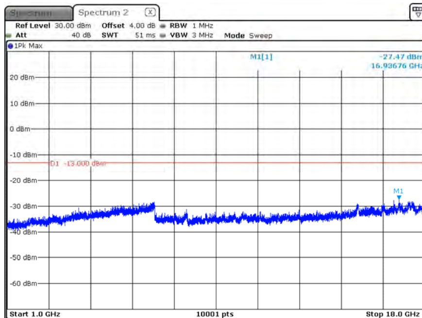
B12_CH23060_10M_1RB0_16-QAM_Above 1G
