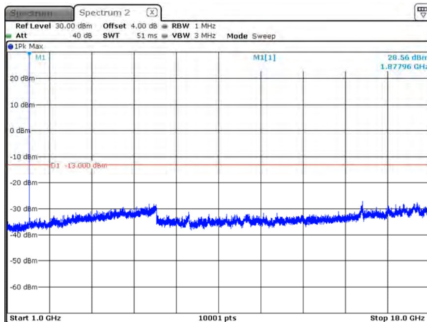
B25_CH26365_10M_1RB0_16-QAM_Above 1G
