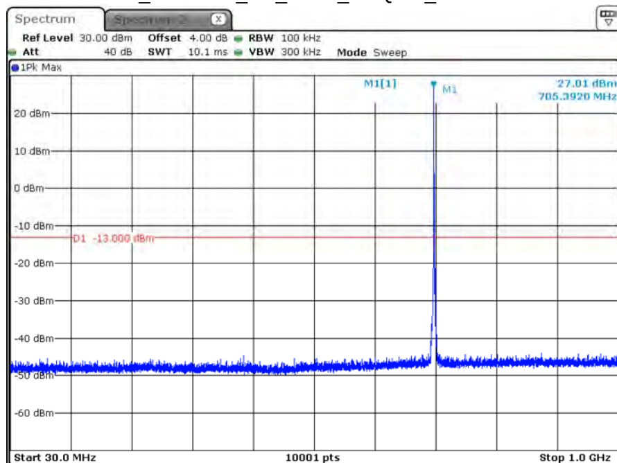
B12_CH23095_5M_1RB0_16-QAM_Below 1G
