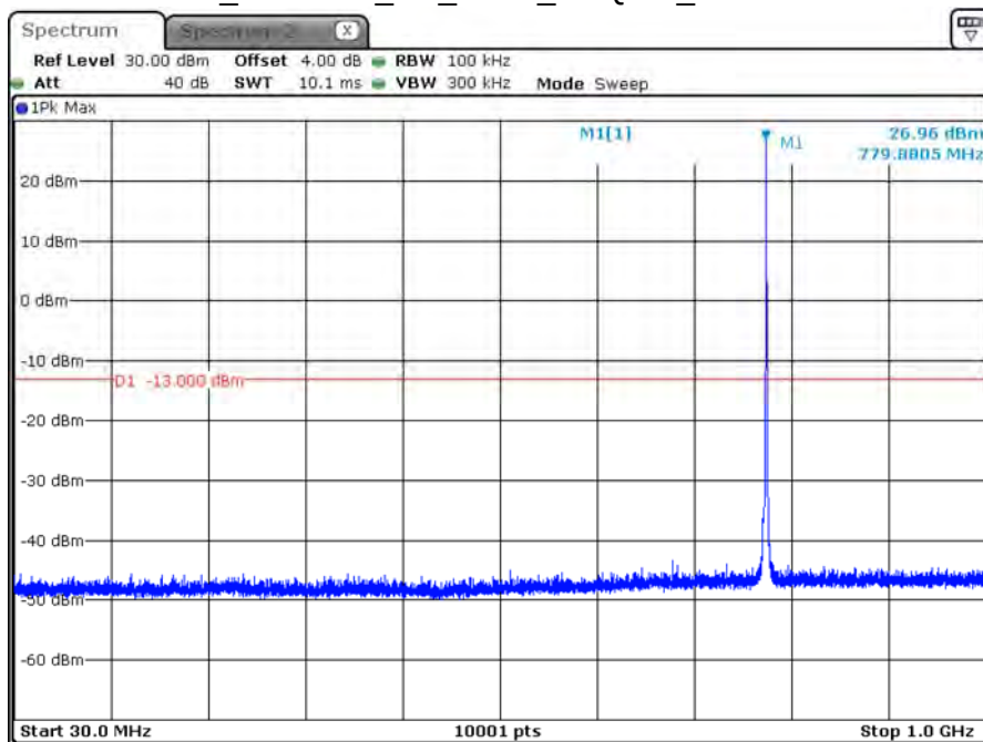
B13_CH23230_5M_1RB0_16-QAM_Below 1G
