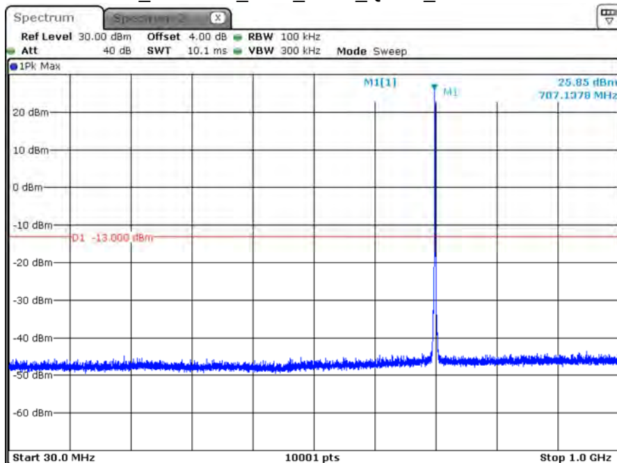
B12_CH23095_1.4M_1RB0_QPSK_Below 1G
