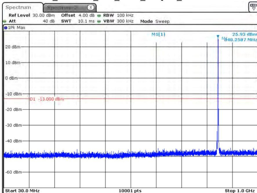
B5_CH20600_10M_1RB5_16-QAM_Below 1G
