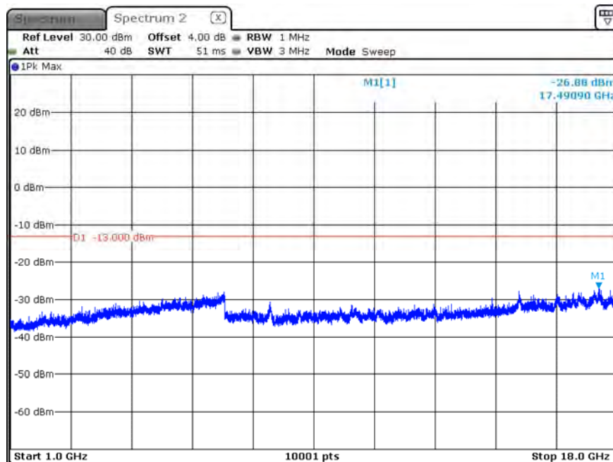
B12_CH23017_1.4M_1RB0_16-QAM_Above 1G
