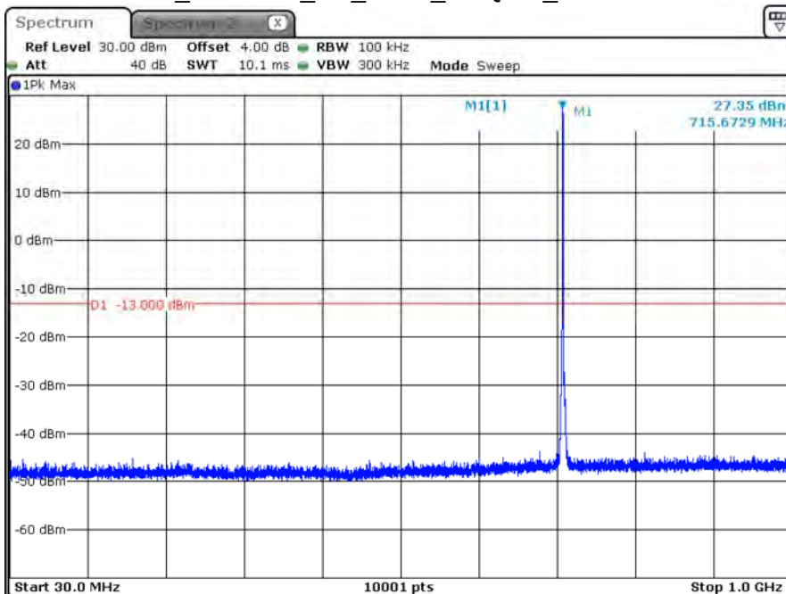
B12_CH23155_5M_1RB5_16-QAM_Below 1G
