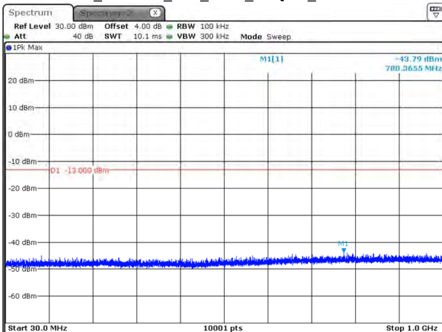
B25_CH26365_10M_1RB0_16-QAM_Below 1G
