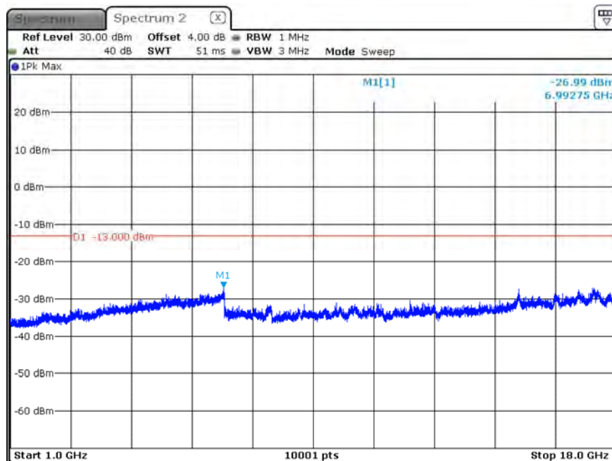
B13_CH23230_5M_1RB0_16-QAM_Above 1G
