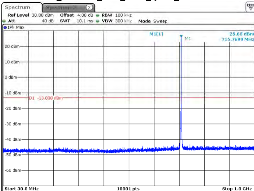
B12_CH23173_1.4M_1RB5_QPSK_Below 1G
