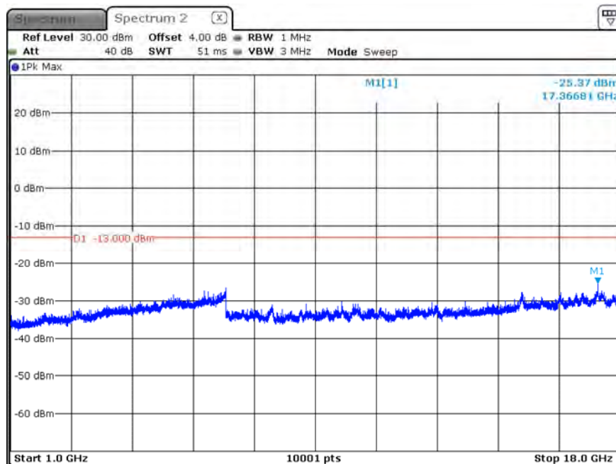
B5_CH20600_10M_1RB5_16-QAM_Above 1G
