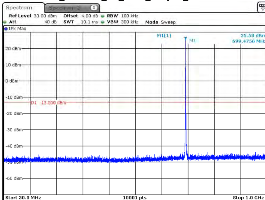
B12_CH23025_3M_1RB0_16-QAM_Below 1G
