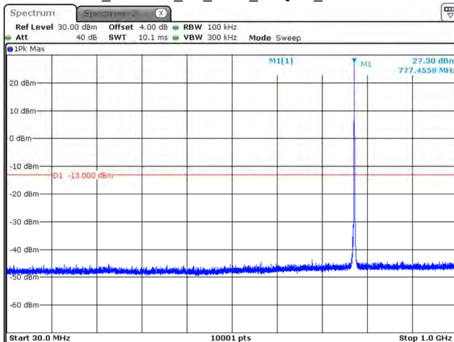
B13_CH23205_5M_1RB0_16-QAM_Below 1G
