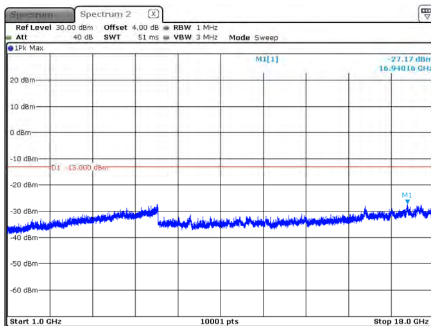
B12_CH23017_1.4M_1RB0_QPSK_Above 1G
