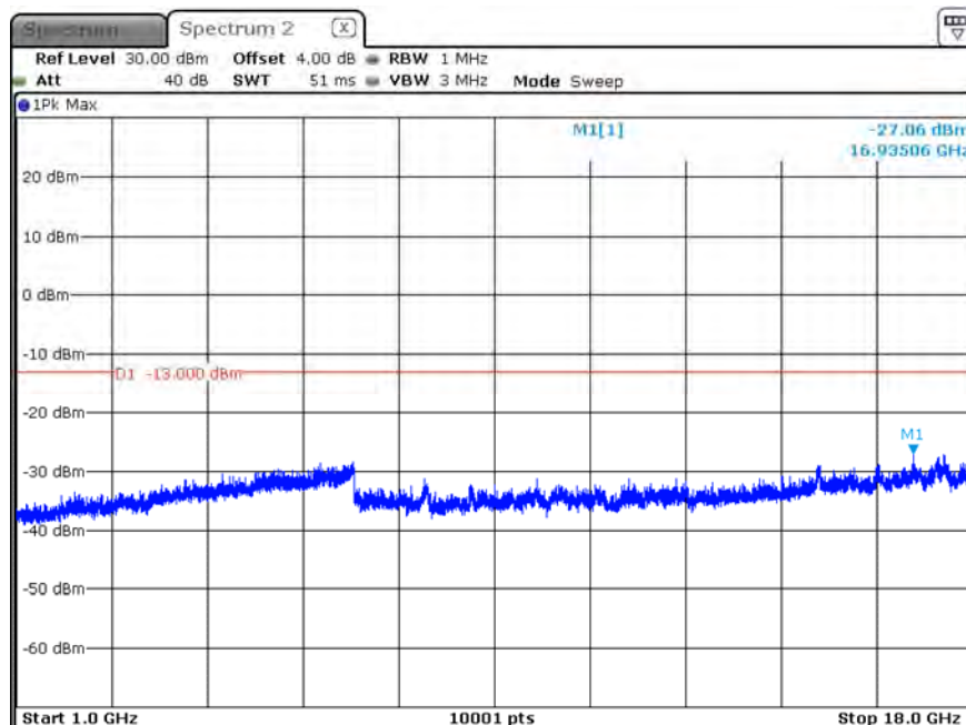
B12_CH23155_5M_1RB5_16-QAM_Above 1G
