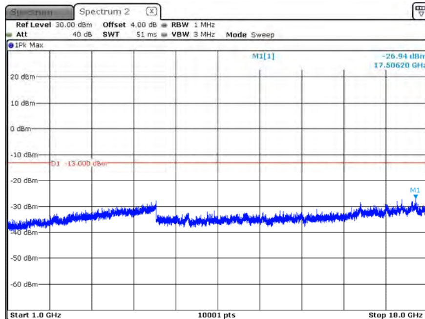
B12_CH23095_5M_1RB0_16-QAM_Above 1G
