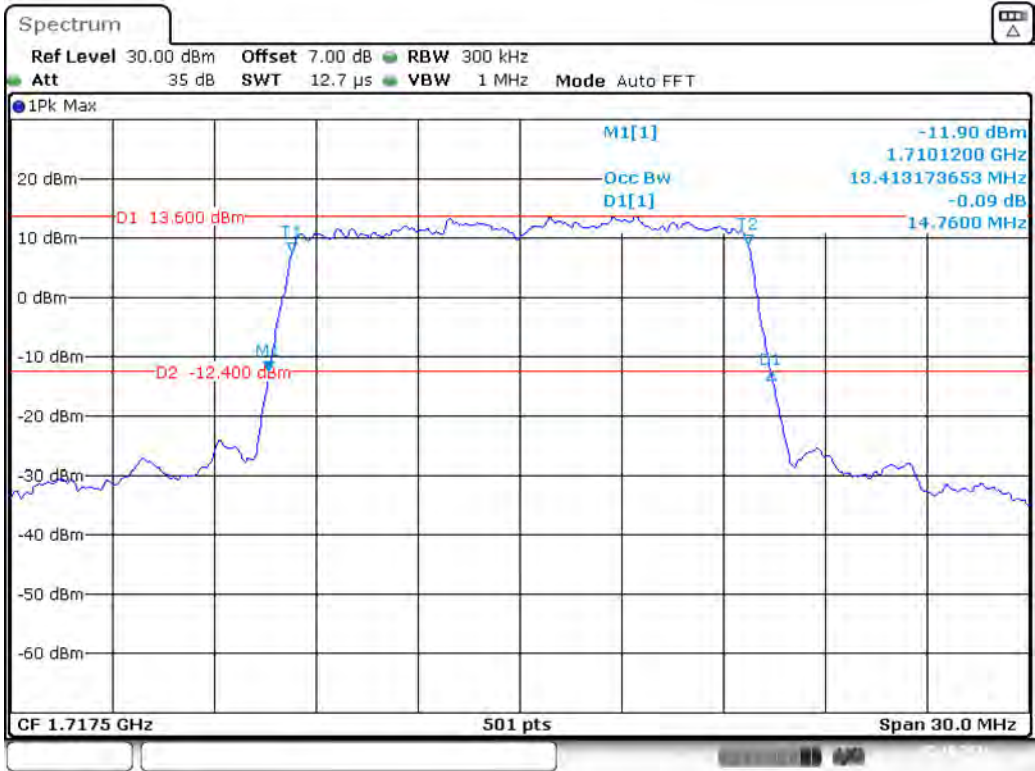
Band 4_15 MHz_Low_QPSK_RB75#0
