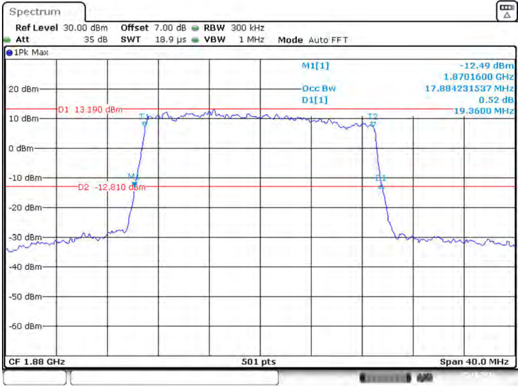
Band 2_20 MHz_Middle_16QAM_RB100#0
