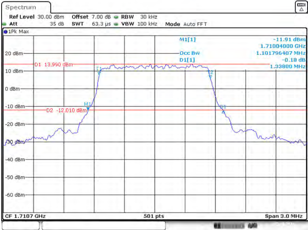
Band 4_1.4 MHz_Low_QPSK_RB6#0
