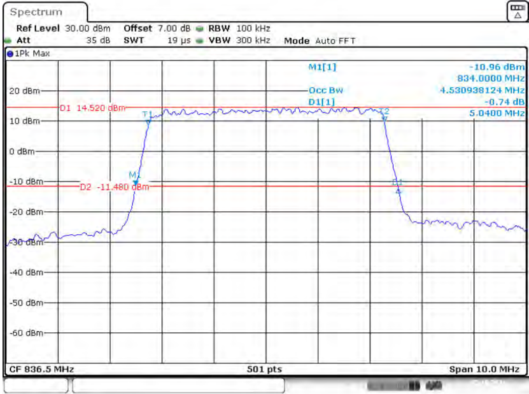
Band 5_5 MHz_Middle_16QAM_RB25#0
