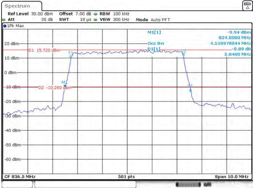
Band 5_5 MHz_Middle_QPSK_RB25#0
