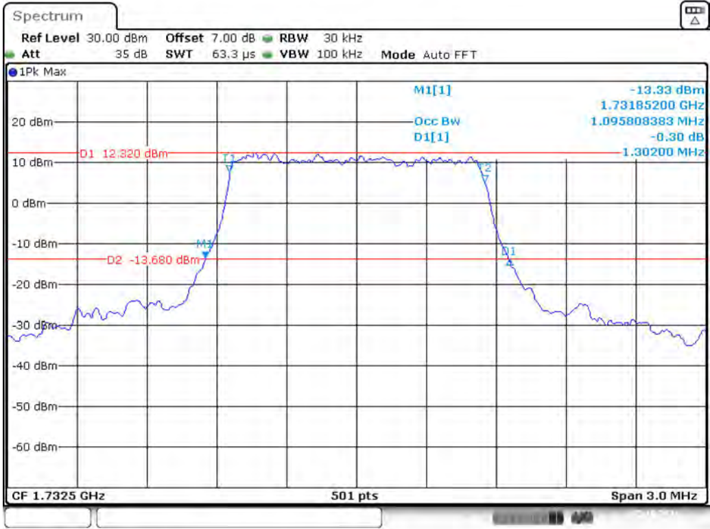
Band 4_1.4 MHz_Middle_16QAM_RB6#0
