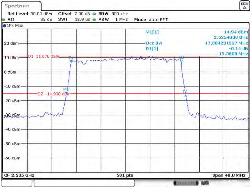
Band 7_20 MHz_Middle_QPSK_RB100#0
