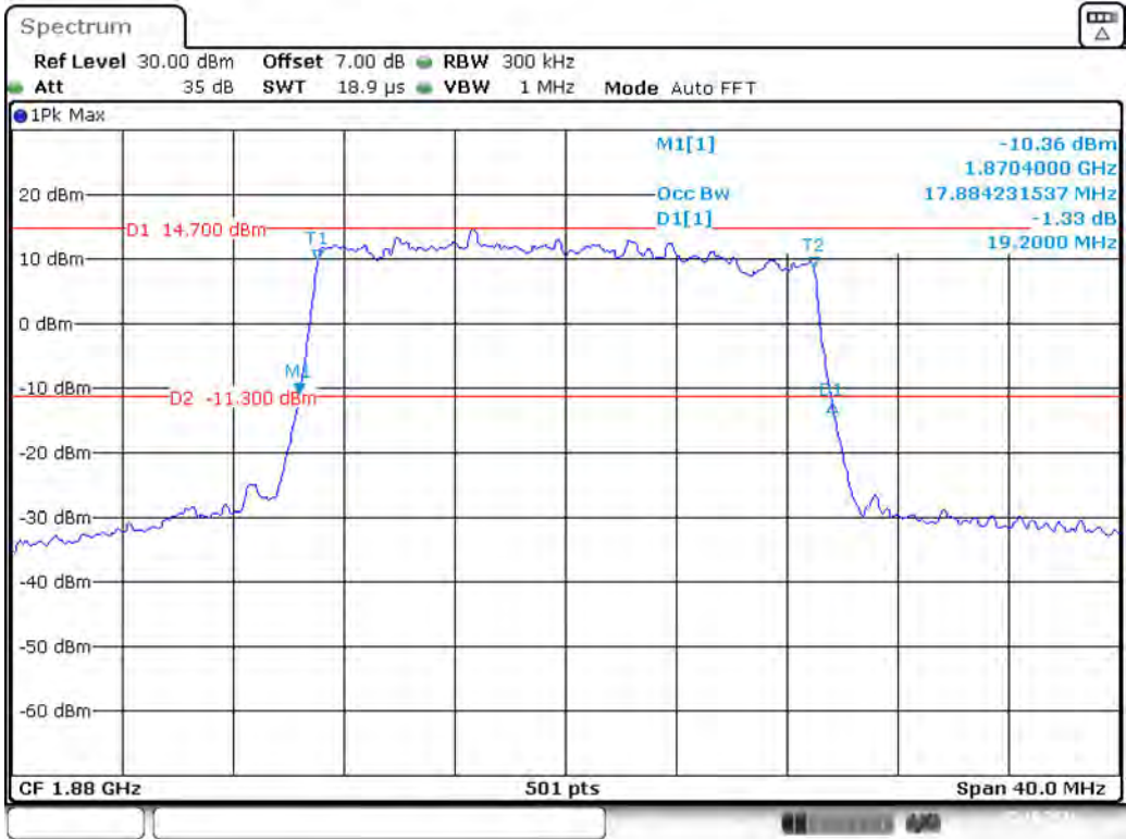
Band 2_20 MHz_Middle_QPSK_RB100#0
