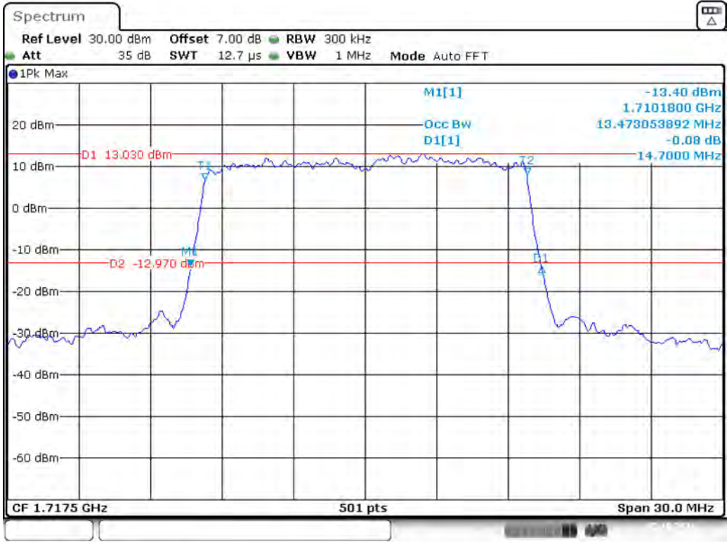
Band 4_15 MHz_Low_16QAM_RB75#0
