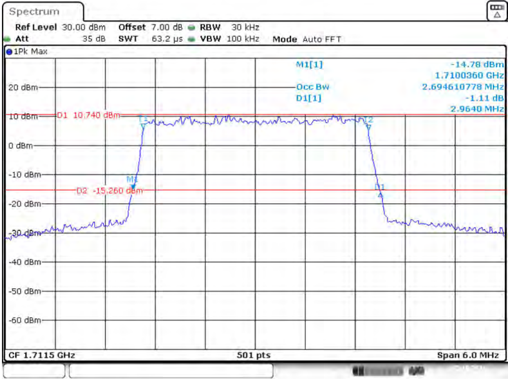
Band 66_3 MHz_Low_16QAM_RB15#0
