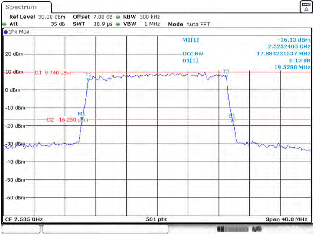
Band 7_20 MHz_Middle_16QAM_RB100#0
