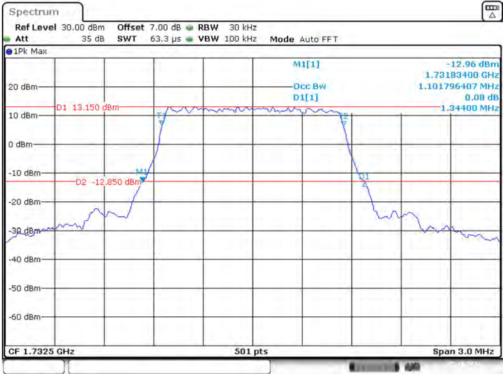
Band 4_1.4 MHz_Middle_QPSK_RB6#0
