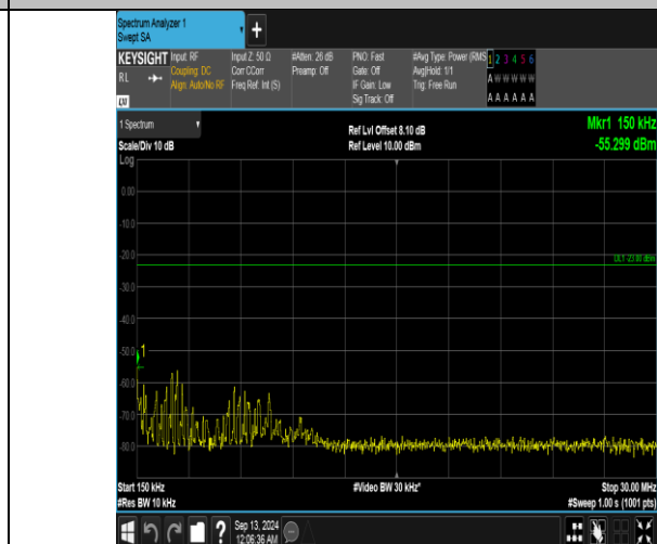
Band5_5MHz_QPSK_20625_1RB#0_0.15~30_0.15~30
