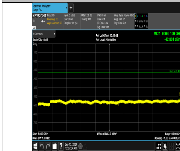
Band5_5MHz_QPSK_20625_1RB#0_3000~10000_3000~10000
