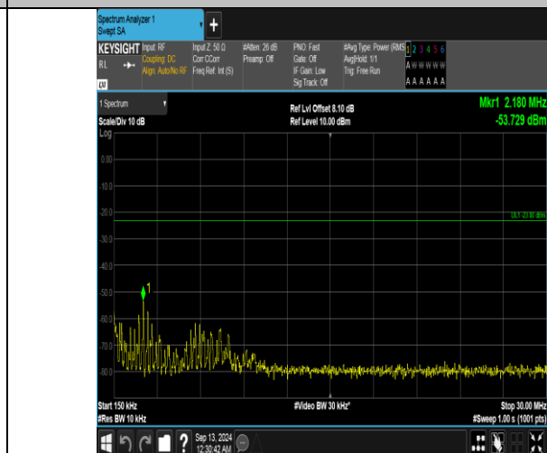
Band5_10MHz_QPSK_20525_1RB#0_0.15~30_0.15~30
