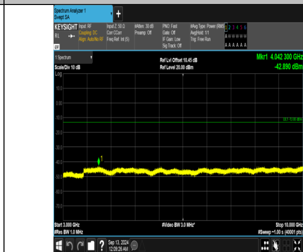
Band5_5MHz_16QAM_20625_1RB#24_3000~10000_3000~10000
