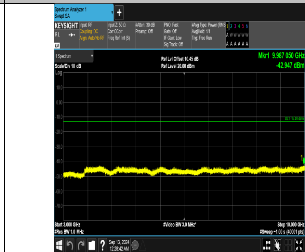
Band5_10MHz_16QAM_20450_1RB#49_3000~10000_3000~10000
