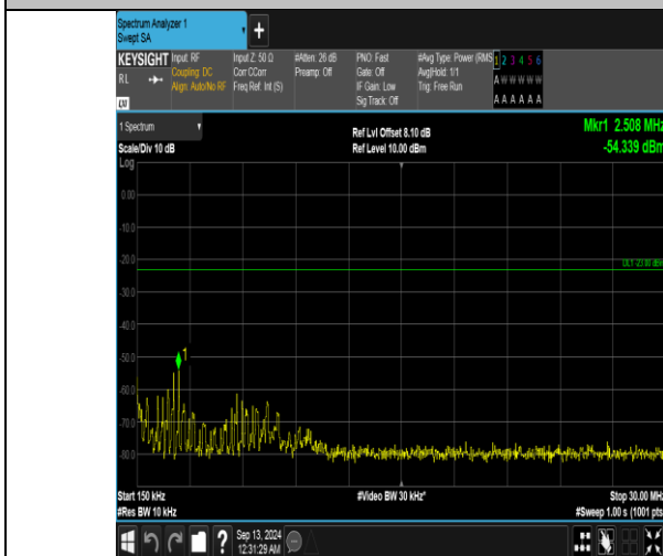
Band5_10MHz_16QAM_20525_1RB#0_0.15~30_0.15~30
