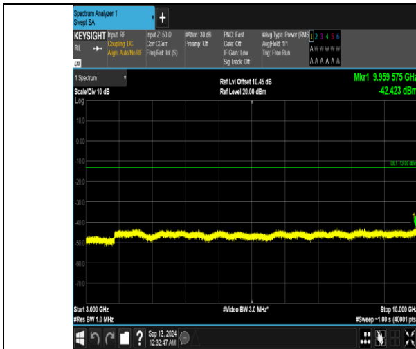
Band5_10MHz_QPSK_20525_1RB#49_3000~10000_3000~10000
