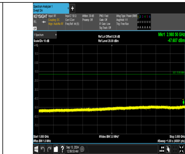
Band5_5MHz_QPSK_20625_1RB#0_1000~3000_1000~3000
