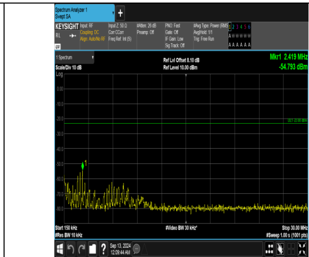
Band5_5MHz_QPSK_20625_25RB#0_0.15~30_0.15~30
