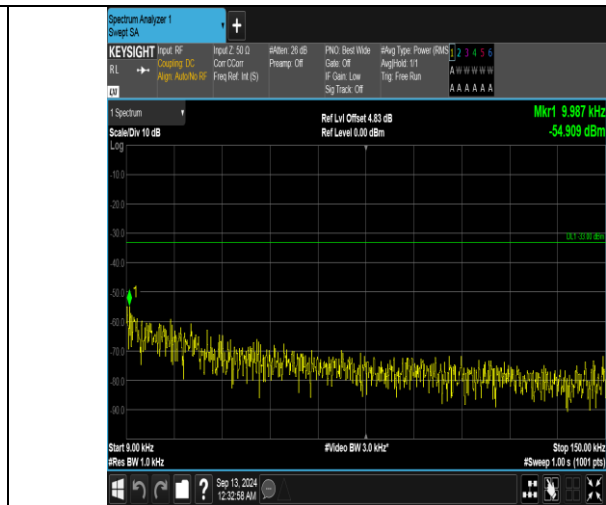
Band5_10MHz_16QAM_20525_1RB#49_0.009~0.15_0.009~0.15
