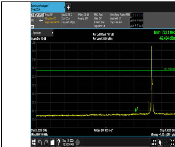
Band5_10MHz_QPSK_20525_1RB#0_30~1000_30~1000
