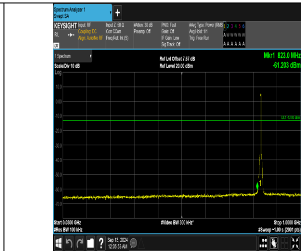
Band5_5MHz_16QAM_20525_25RB#0_30~1000_30~1000
