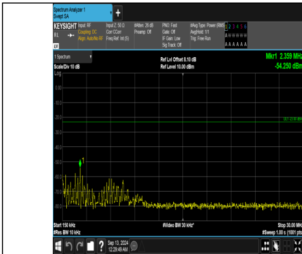
Band5_10MHz_16QAM_20450_50RB#0_0.15~30_0.15~30
