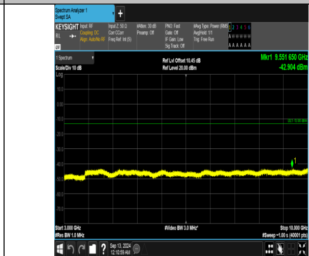
Band5_5MHz_16QAM_20625_25RB#0_3000~10000_3000~10000
