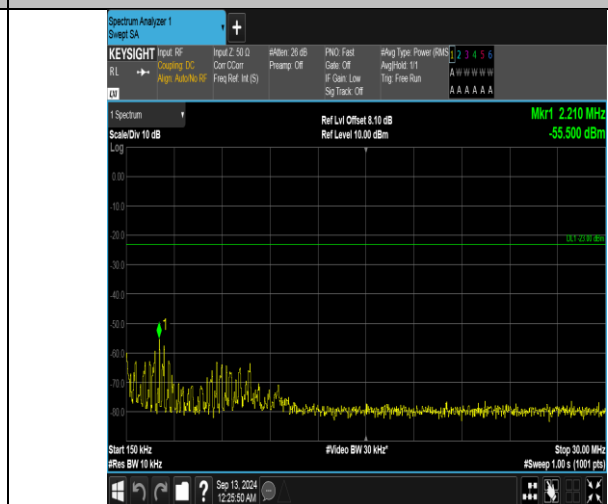
Band5_10MHz_QPSK_20450_1RB#0_0.15~30_0.15~30
