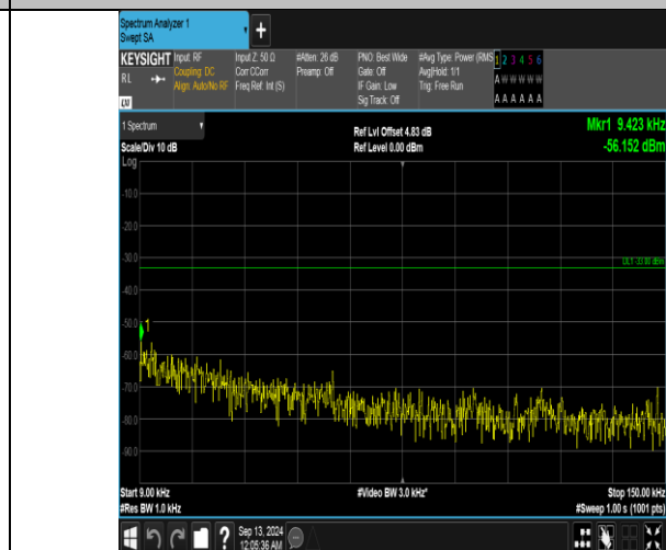
Band5_5MHz_16QAM_20525_25RB#0_0.009~0.15_0.009~0.15
