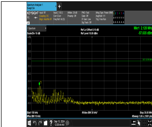
Band5_5MHz_16QAM_20525_25RB#0_0.15~30_0.15~30
