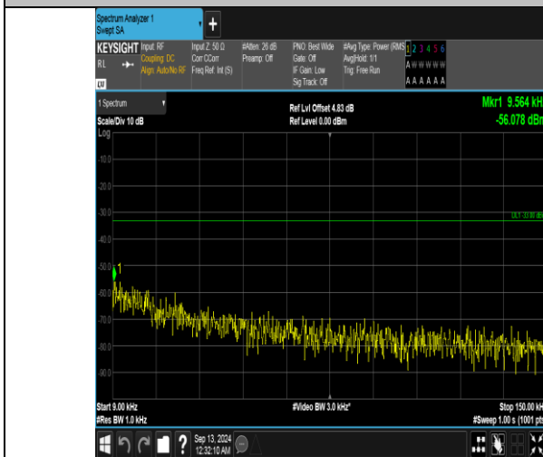
Band5_10MHz_QPSK_20525_1RB#49_0.009~0.15_0.009~0.15
