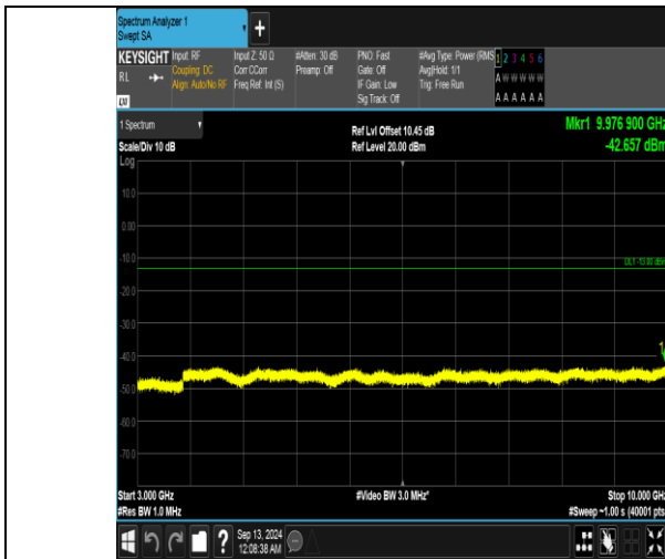
Band5_5MHz_QPSK_20625_1RB#24_3000~10000_3000~10000
