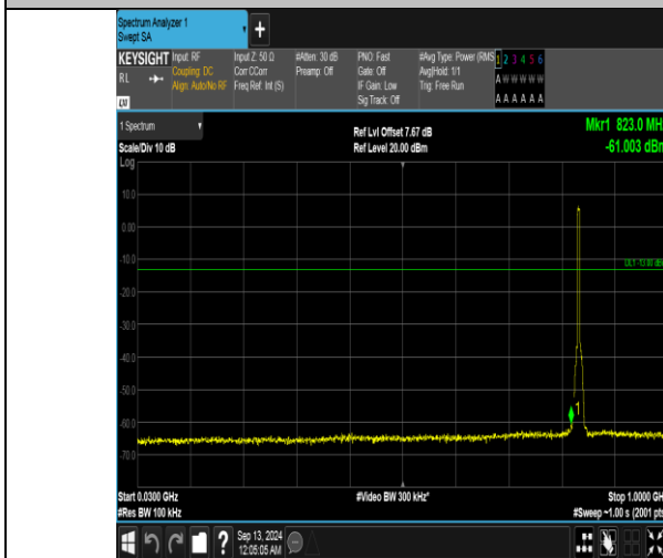
Band5_5MHz_QPSK_20525_25RB#0_30~1000_30~1000
