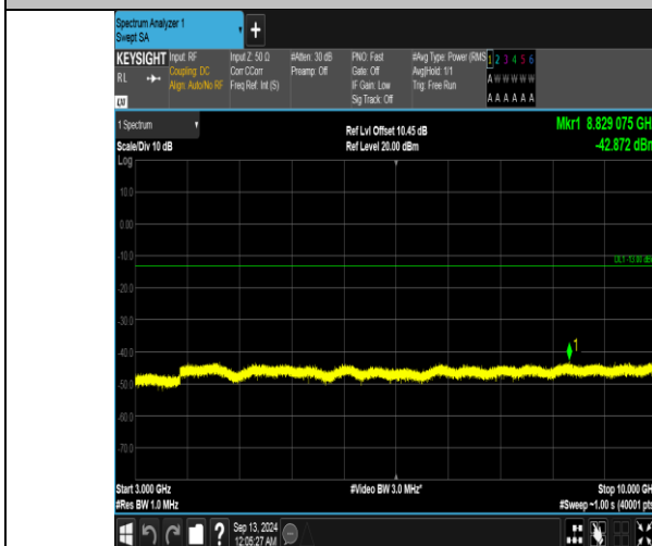
Band5_5MHz_QPSK_20525_25RB#0_3000~10000_3000~10000
