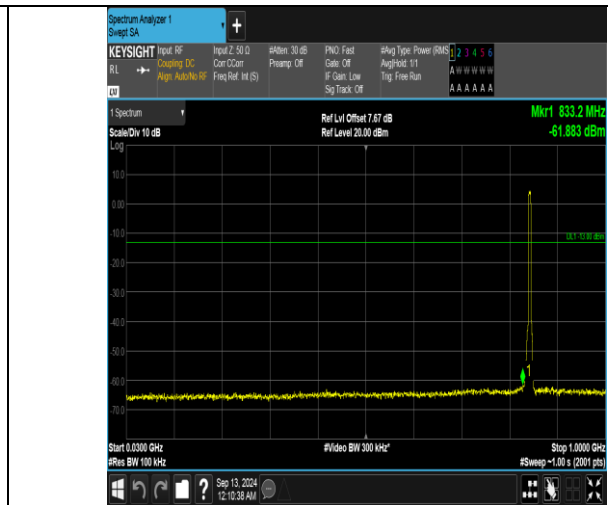
Band5_5MHz_16QAM_20625_25RB#0_30~1000_30~1000
