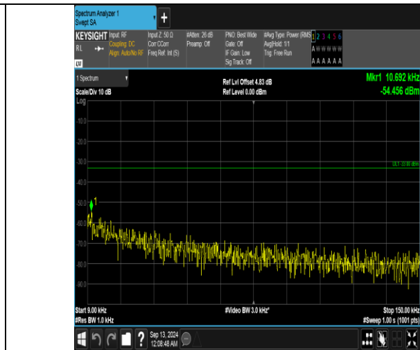
Band5_5MHz_16QAM_20625_1RB#24_0.009~0.15_0.009~0.15
