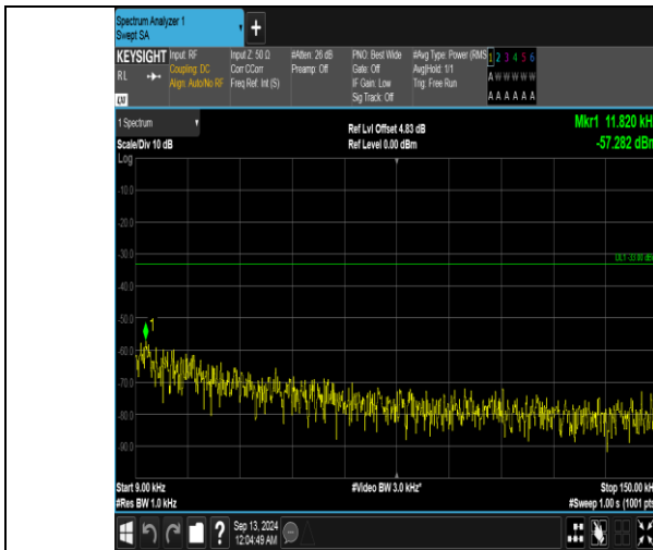
Band5_5MHz_QPSK_20525_25RB#0_0.009~0.15_0.009~0.15
