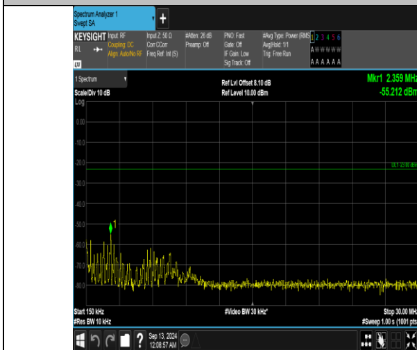
Band5_5MHz_16QAM_20625_1RB#24_0.15~30_0.15~30
