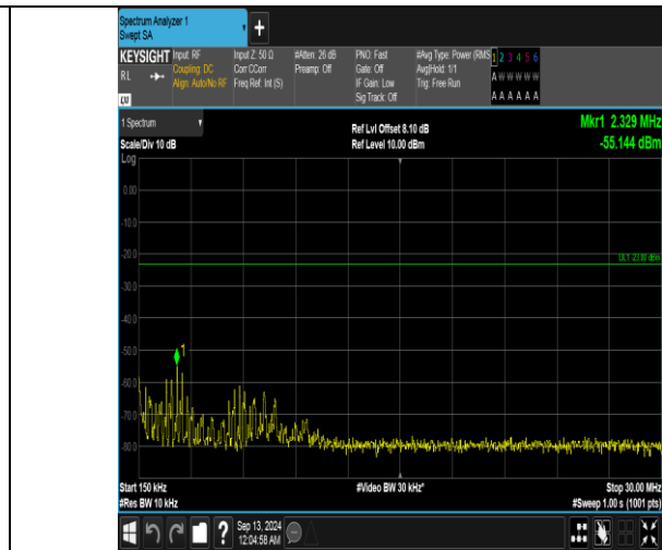
Band5_5MHz_QPSK_20525_25RB#0_0.15~30_0.15~30
