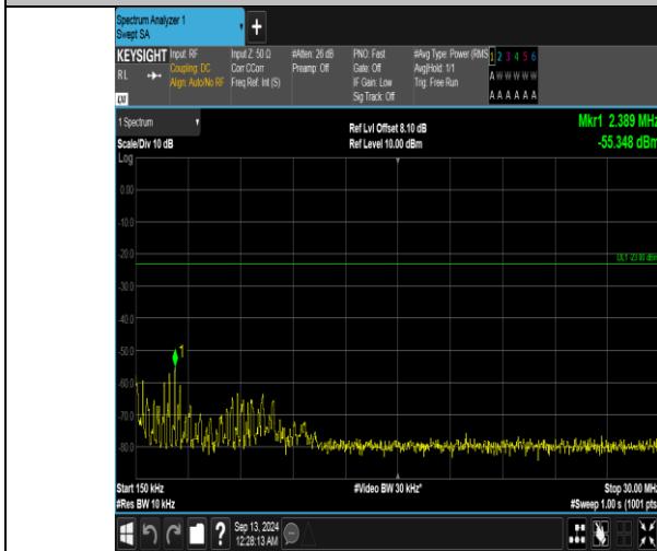
Band5_10MHz_16QAM_20450_1RB#49_0.15~30_0.15~30
