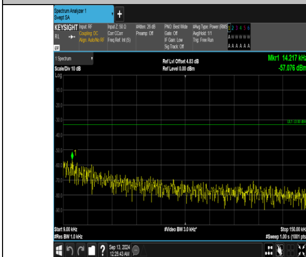
Band5_10MHz_QPSK_20450_1RB#0_0.009~0.15_0.009~0.15
