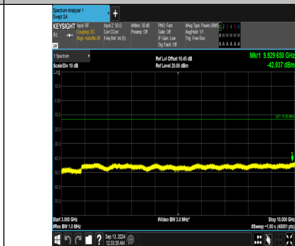
Band5_10MHz_16QAM_20525_1RB#49_3000~10000_3000~10000
