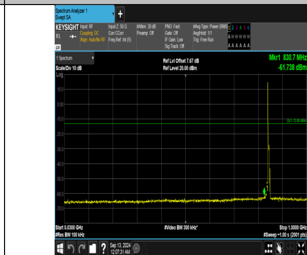
Band5_5MHz_16QAM_20625_1RB#0_30~1000_30~1000
