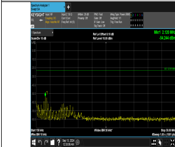
Band5_10MHz_16QAM_20525_1RB#49_0.15~30_0.15~30
