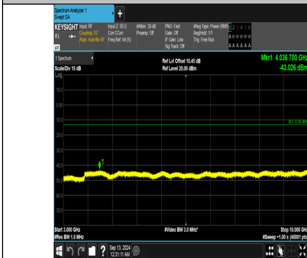
Band5_10MHz_QPSK_20525_1RB#0_3000~10000_3000~10000
