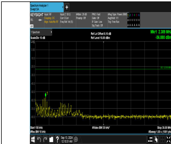
Band5_5MHz_16QAM_20625_25RB#0_0.15~30_0.15~30
