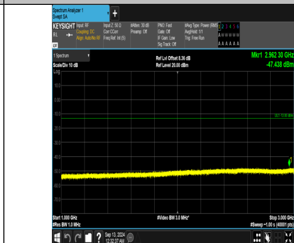
Band5_10MHz_QPSK_20525_1RB#49_1000~3000_1000~3000
