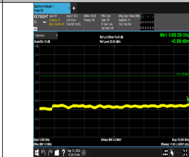
Band5_10MHz_16QAM_20450_50RB#0_3000~10000_3000~10000
