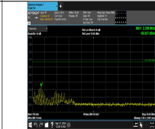
Band5_5MHz_QPSK_20625_1RB#24_0.15~30_0.15~30
