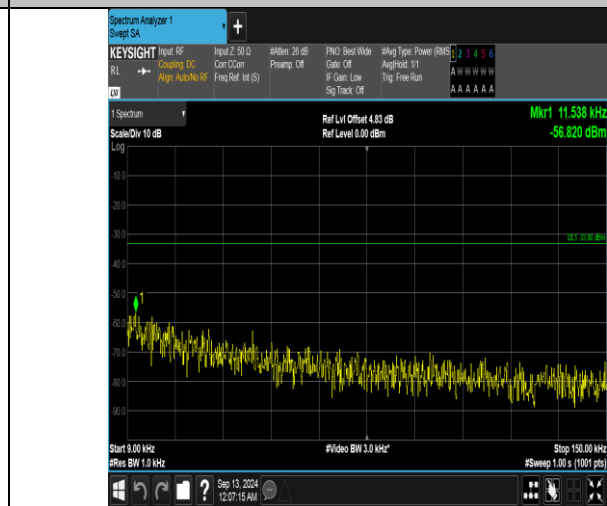
Band5_5MHz_16QAM_20625_1RB#0_0.009~0.15_0.009~0.15
