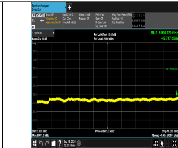
Band5_10MHz_16QAM_20525_1RB#0_3000~10000_3000~10000
