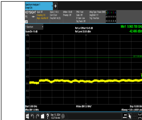
Band5_10MHz_QPSK_20450_1RB#49_3000~10000_3000~10000
