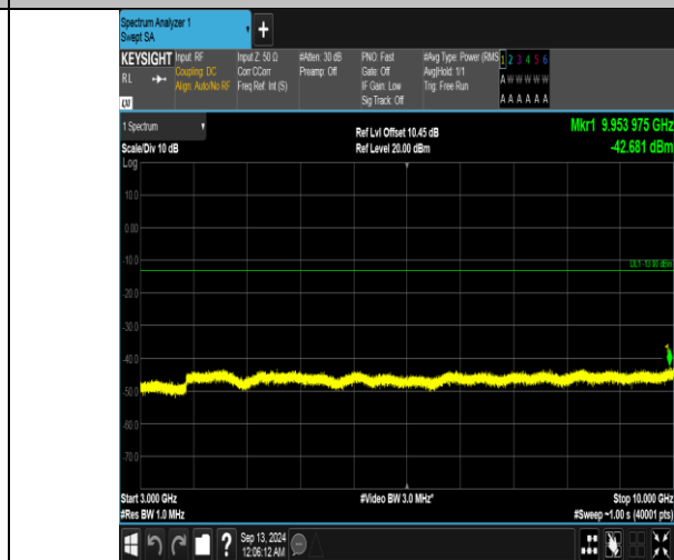
Band5_5MHz_16QAM_20525_25RB#0_3000~10000_3000~10000
