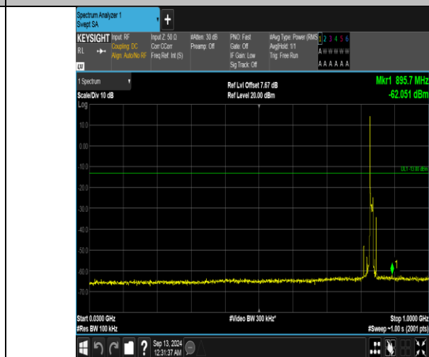
Band5_10MHz_16QAM_20525_1RB#0_30~1000_30~1000
