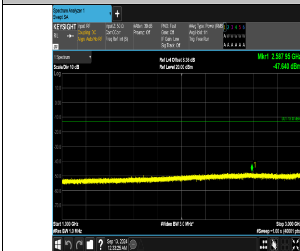
Band5_10MHz_16QAM_20525_1RB#49_1000~3000_1000~3000
