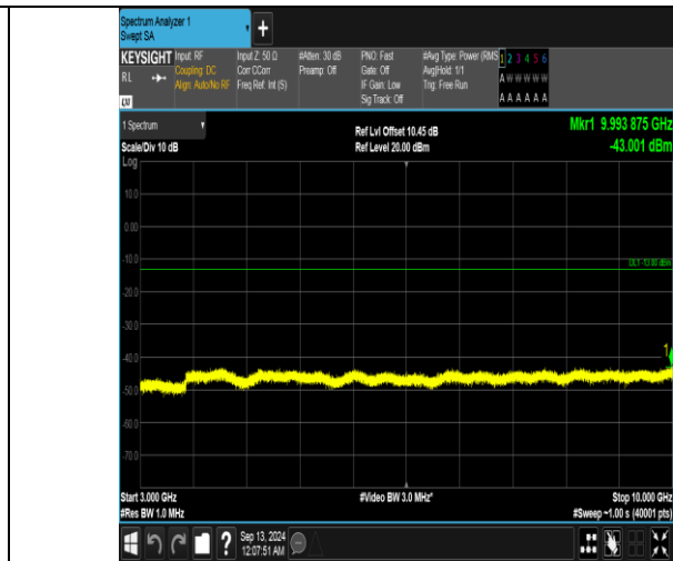
Band5_5MHz_16QAM_20625_1RB#0_3000~10000_3000~10000
