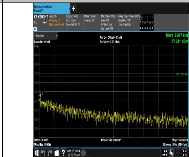
Band5_5MHz_16QAM_20625_25RB#0_0.009~0.15_0.009~0.15
