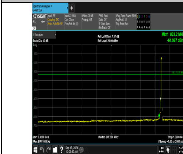
Band5_5MHz_QPSK_20625_25RB#0_30~1000_30~1000
