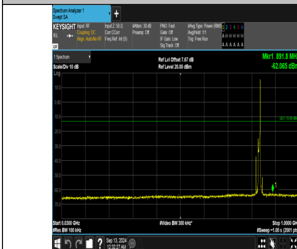
Band5_10MHz_QPSK_20525_1RB#49_30~1000_30~1000
