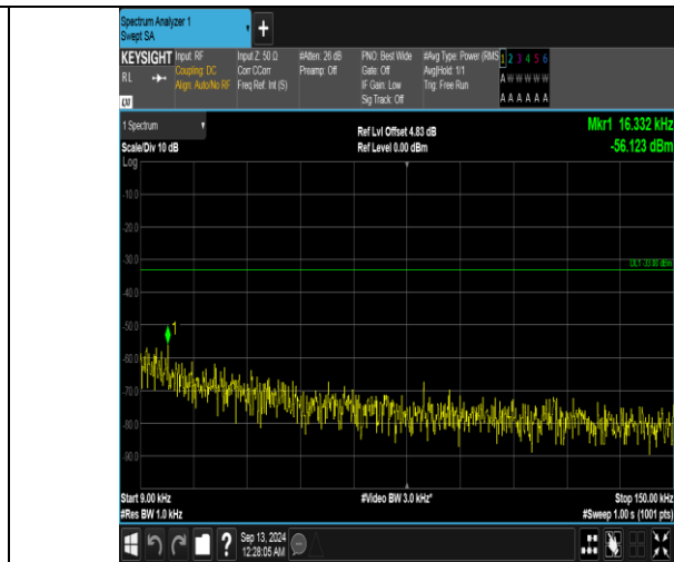
Band5_10MHz_16QAM_20450_1RB#49_0.009~0.15_0.009~0.15
