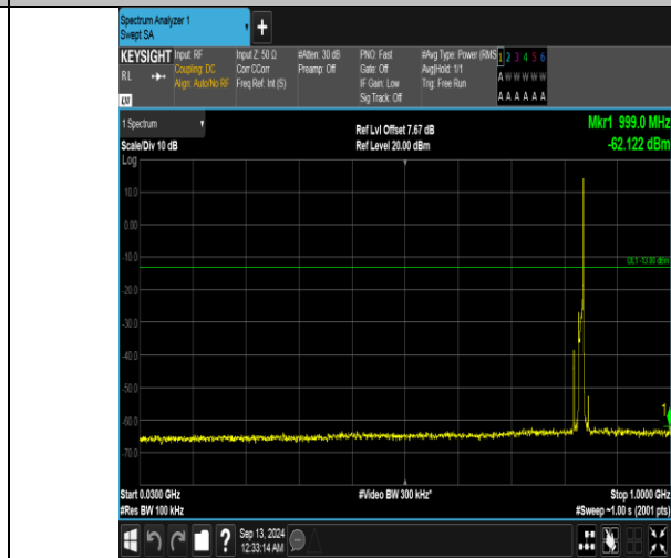
Band5_10MHz_16QAM_20525_1RB#49_30~1000_30~1000
