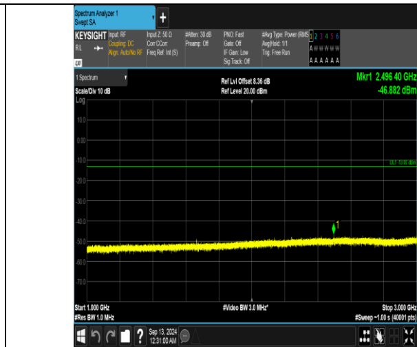
Band5_10MHz_QPSK_20525_1RB#0_1000~3000_1000~3000
