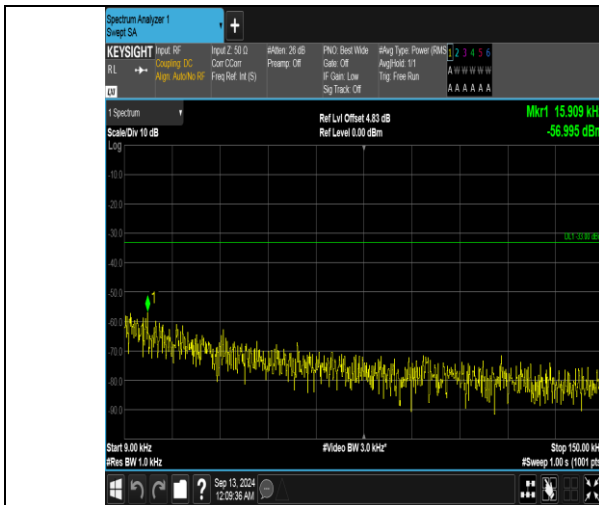
Band5_5MHz_QPSK_20625_25RB#0_0.009~0.15_0.009~0.15
