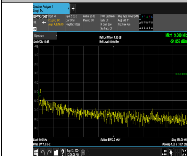
Band5_5MHz_QPSK_20625_1RB#0_0.009~0.15_0.009~0.15
