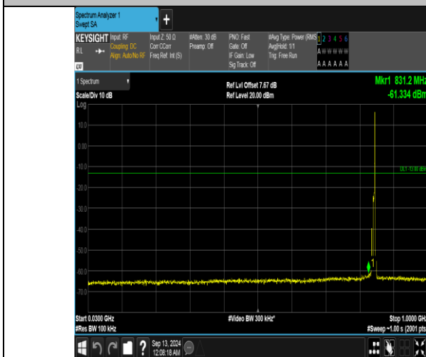
Band5_5MHz_QPSK_20625_1RB#24_30~1000_30~1000
