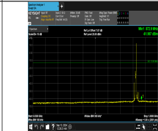
Band5_10MHz_16QAM_20450_1RB#49_30~1000_30~1000
