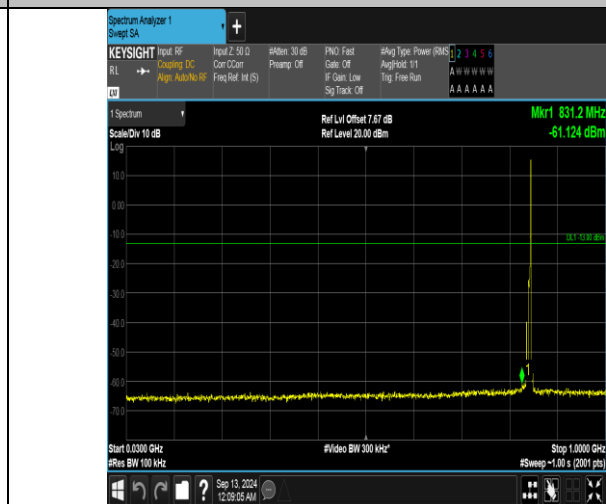
Band5_5MHz_16QAM_20625_1RB#24_30~1000_30~1000
