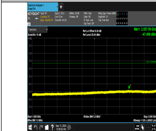
Band5_5MHz_16QAM_20525_25RB#0_1000~3000_1000~3000
