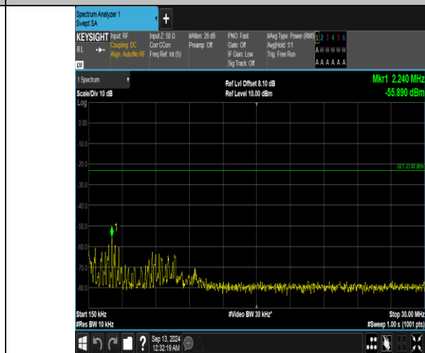
Band5_10MHz_QPSK_20525_1RB#49_0.15~30_0.15~30
