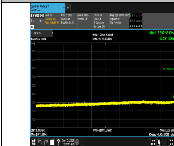
Band5_5MHz_16QAM_20625_1RB#24_1000~3000_1000~3000
