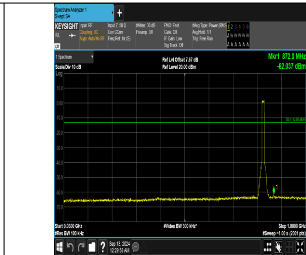
Band5_10MHz_16QAM_20450_50RB#0_30~1000_30~1000
