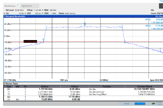
N66-15kHz-15MHz-CP-64QAM-Mid-Outer_Full---PASS
