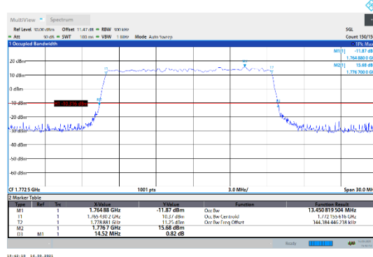
N66-15kHz-15MHz-DFT-256QAM-High-Outer_Full---PASS
