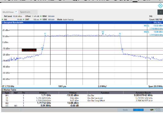
N66-15kHz-10MHz-CP-16QAM-Low-Outer_Full--- PASS
