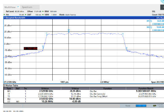
N7-15kHz-10MHz-CP-16QAM-Mid-Outer_Full---PASS
