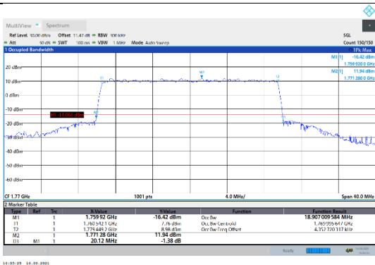
N66-15kHz-20MHz-CP-256QAM-High-Outer_Full---PASS
