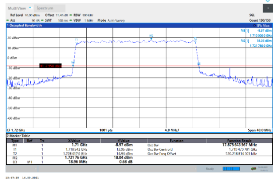
N66-15kHz-20MHz-DFT-QPSK-Low-Outer_Full---PASS
