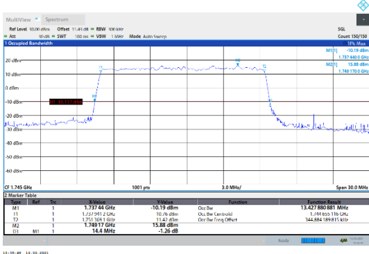
N66-15kHz-15MHz-DFT-256QAM-Mid-Outer_Full---PASS
