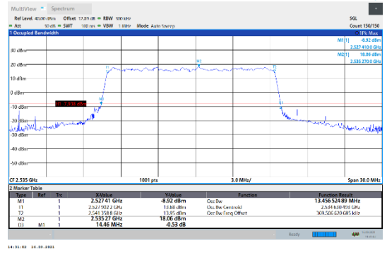
N7-15kHz-15MHz-DFT-QPSK-Mid-Outer_Full---PASS
