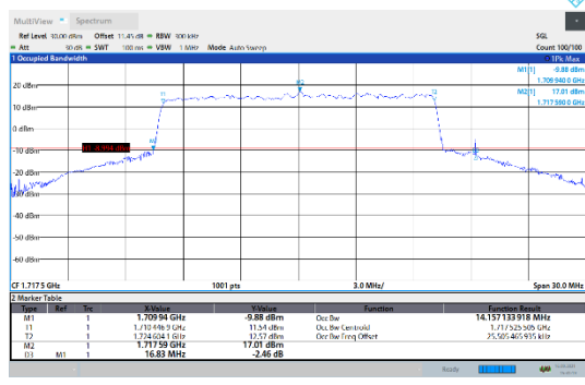
N66-15kHz-15MHz-CP-64QAM-Low-Outer_Full---PASS
