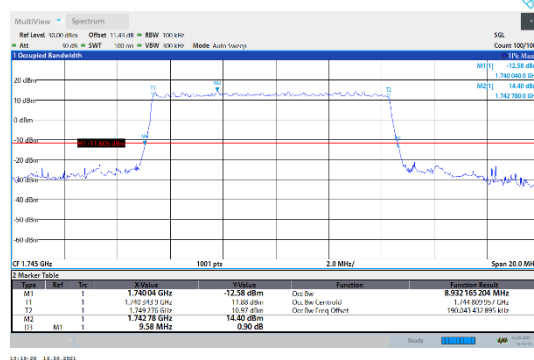
N66-15kHz-10MHz-DFT-16QAM-Mid-Outer_Full---PASS
