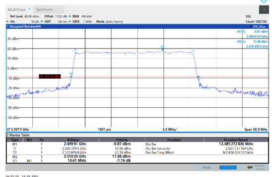
N7-15kHz-15MHz-DFT-16QAM-Low-Outer_Full---PASS
