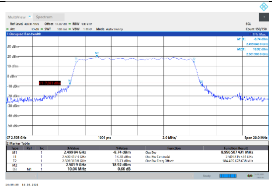
N7-15kHz-10MHz-DFT-64QAM-Low-Outer_Full--- PASS
