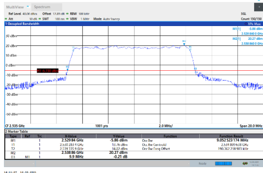
N7-15kHz-10MHz-DFT-QPSK-Mid-Outer_Full---PASS
