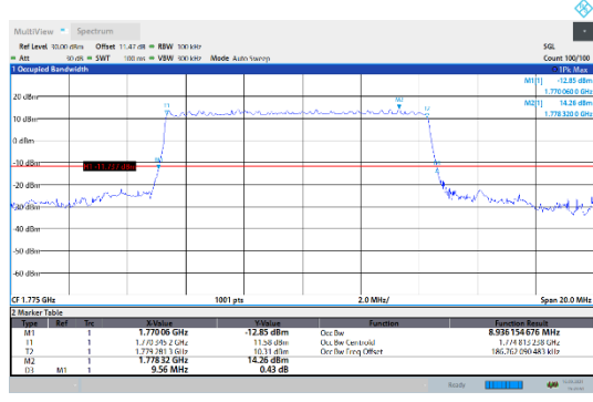
N66-15kHz-10MHz-DFT-16QAM-High-Outer_Full---PASS
