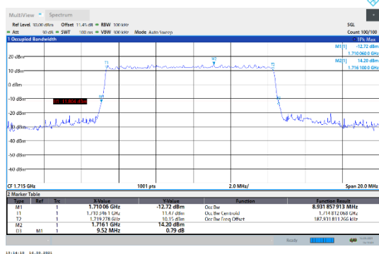
N66-15kHz-10MHz-DFT-16QAM-Low-Outer_Full---PASS
