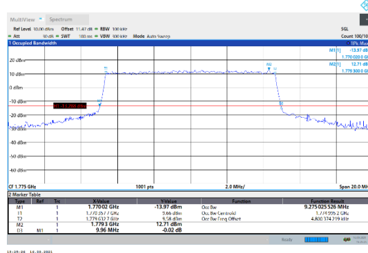
N66-15kHz-10MHz-CP-QPSK-High-Outer_Full---PASS
