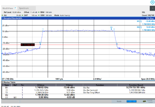
N66-15kHz-10MHz-CP-QPSK-Mid-Outer_Full---PASS
