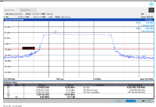
N7-15kHz-10MHz-DFT-64QAM-High-Outer_Full--- PASS
