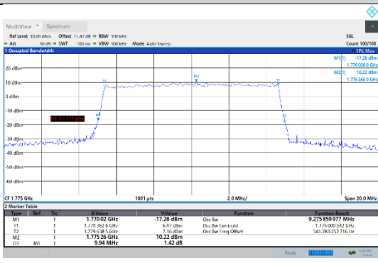
N66-15kHz-10MHz-CP-256QAM-High-Outer_Full--- PASS
