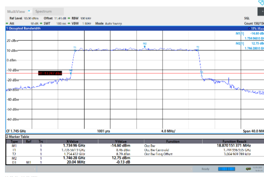
N66-15kHz-20MHz-CP-256QAM-Mid-Outer_Full--- PASS
