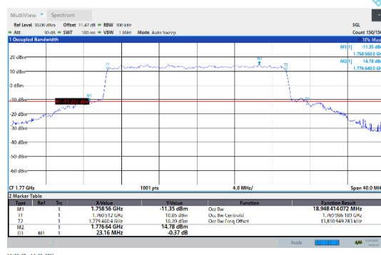
N66-15kHz-20MHz-CP-64QAM-High-Outer_Full--- PASS
