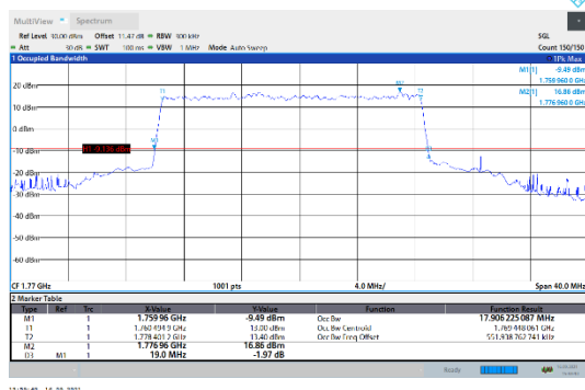
N66-15kHz-20MHz-DFT-16QAM-High-Outer_Full---PASS
