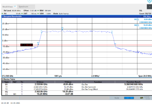
N7-15kHz-10MHz-CP-16QAM-High-Outer_Full---PASS
