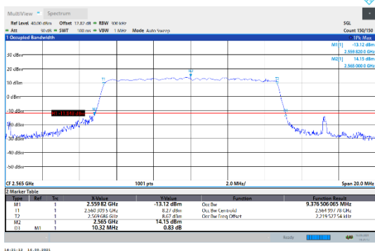
N7-15kHz-10MHz-CP-256QAM-High-Outer_Full---PASS
