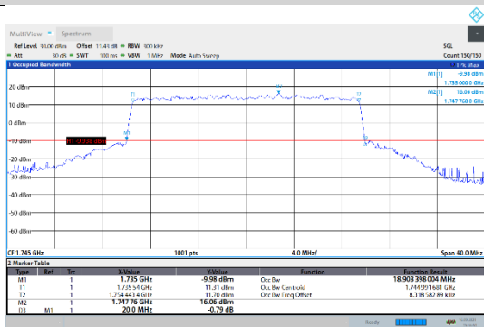
N66-15kHz-20MHz-CP-QPSK-Mid-Outer_Full---PASS
