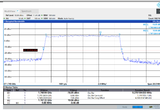
N66-15kHz-10MHz-CP-256QAM-Mid-Outer_Full--- PASS
