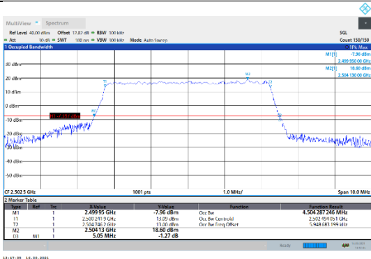
N7-15kHz-5MHz-DFT-QPSK-Low-Outer_Full---PASS
