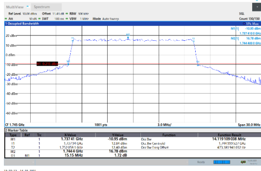
N66-15kHz-15MHz-CP-16QAM-Mid-Outer_Full---PASS
