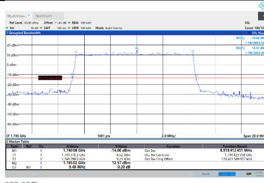
N66-15kHz-10MHz-DFT-256QAM-Mid-Outer_Full--- PASS
