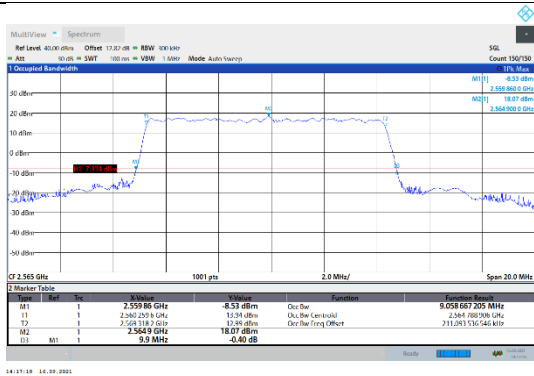
N7-15kHz-10MHz-DFT-16QAM-High-Outer_Full--- PASS
