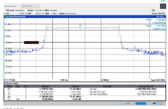
N66-15kHz-20MHz-DFT-64QAM-High-Outer_Full--- PASS
