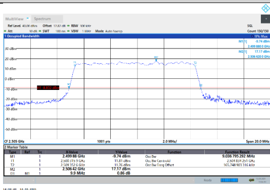
N7-15kHz-10MHz-DFT-256QAM-Low-Outer_Full--- PASS
