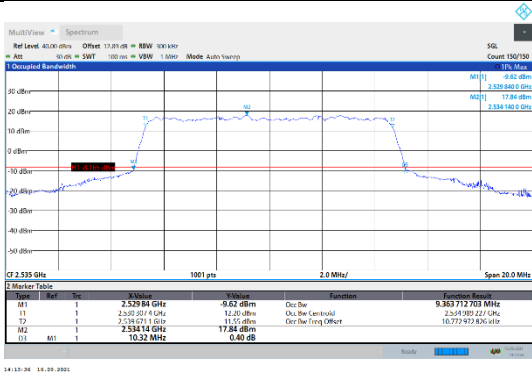
N7-15kHz-10MHz-CP-QPSK-Mid-Outer_Full---PASS
