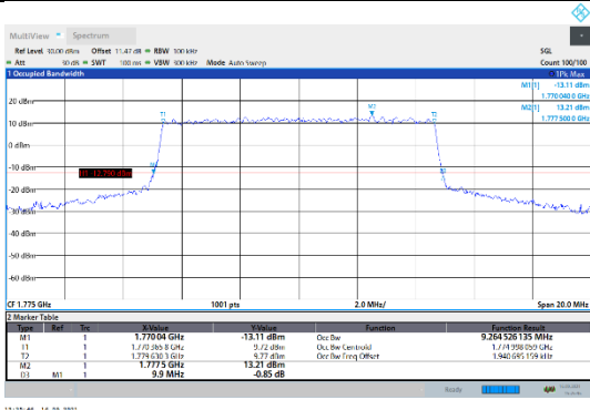
N66-15kHz-10MHz-CP-16QAM-High-Outer_Full--- PASS
