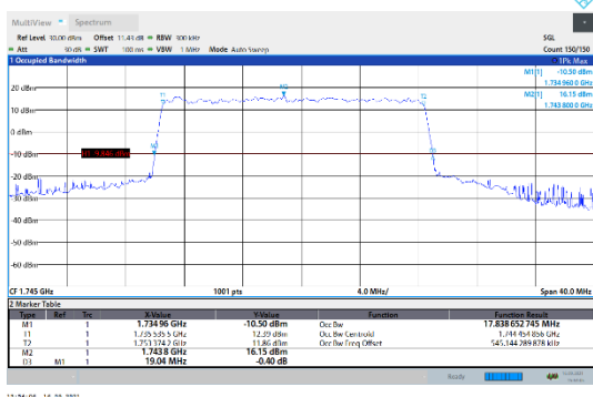
N66-15kHz-20MHz-DFT-64QAM-Mid-Outer_Full--- PASS
