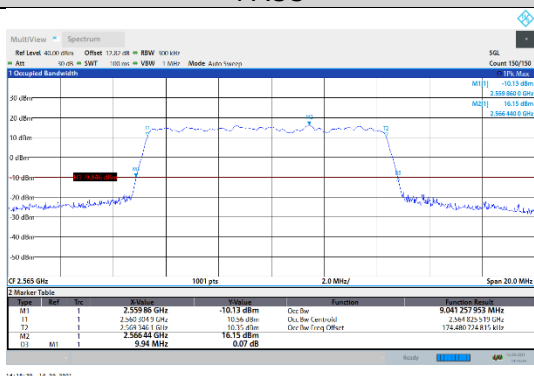
N7-15kHz-10MHz-DFT-256QAM-High-Outer_Full--- PASS
