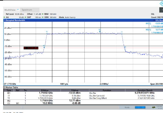
N66-15kHz-10MHz-CP-64QAM-Low-Outer_Full--- PASS
