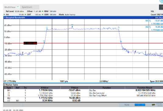
N66-15kHz-10MHz-DFT-QPSK-High-Outer_Full---PASS
