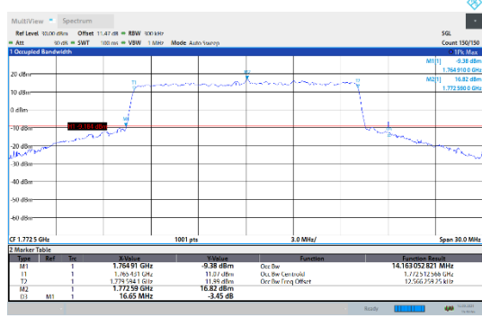
N66-15kHz-15MHz-CP-64QAM-High-Outer_Full---PASS
