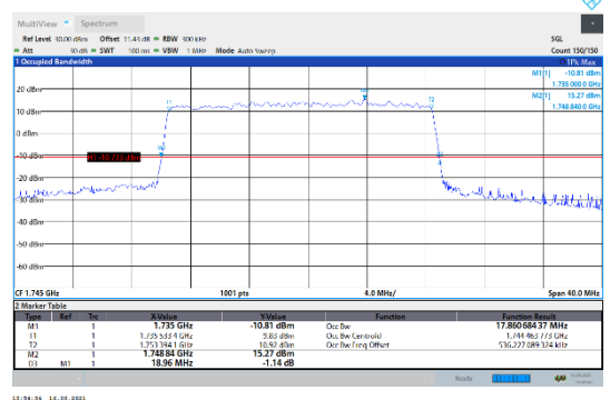
N66-15kHz-20MHz-DFT-256QAM-Mid-Outer_Full--- PASS
