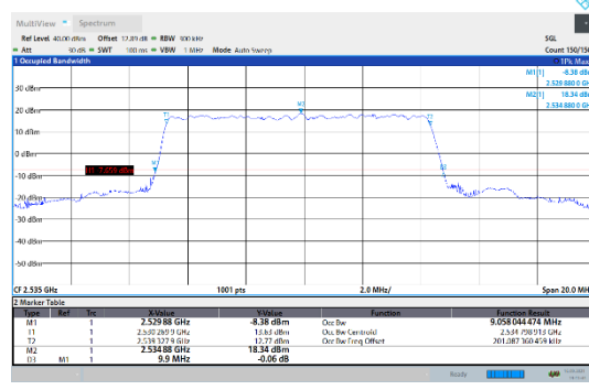
N7-15kHz-10MHz-DFT-16QAM-Mid-Outer_Full---PASS
