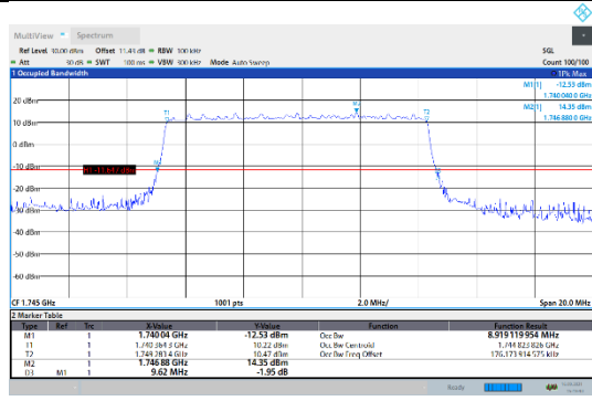
N66-15kHz-10MHz-DFT-64QAM-Mid-Outer_Full---PASS
