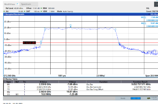
N7-15kHz-10MHz-DFT-QPSK-High-Outer_Full---PASS
