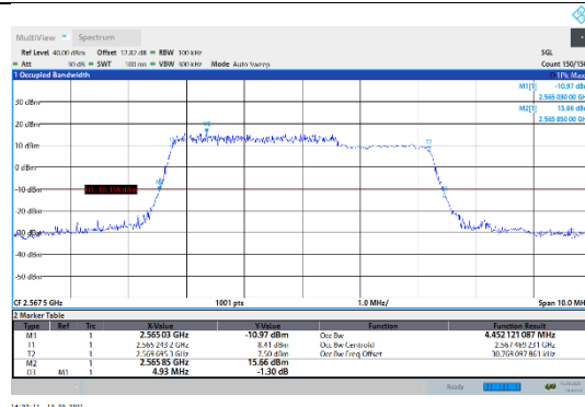
N7-15kHz-5MHz-CP-256QAM-High-Outer_Full---PASS
