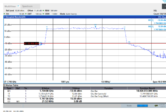
N66-15kHz-20MHz-CP-16QAM-Mid-Outer_Full--- PASS
