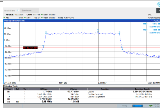
N66-15kHz-10MHz-CP-64QAM-High-Outer_Full--- PASS
