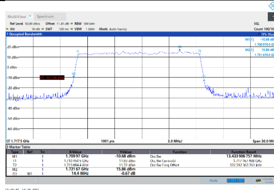
N66-15kHz-15MHz-DFT-256QAM-Low-Outer_Full---PASS
