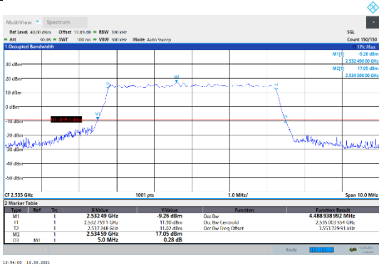
N7-15kHz-5MHz-DFT-16QAM-Mid-Outer_Full---PASS
