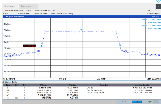
N7-15kHz-10MHz-DFT-16QAM-Low-Outer_Full---PASS
