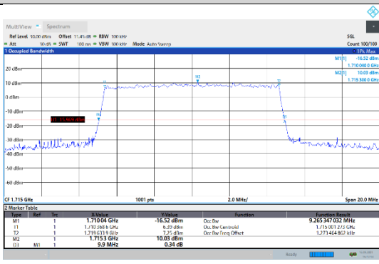
N66-15kHz-10MHz-CP-256QAM-Low-Outer_Full--- PASS
