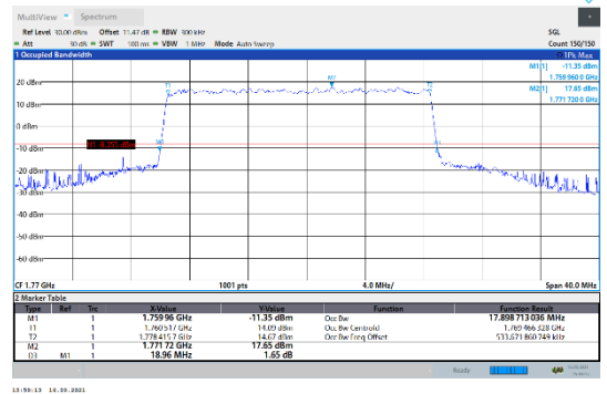
N66-15kHz-20MHz-DFT-QPSK-High-Outer_Full---PASS
