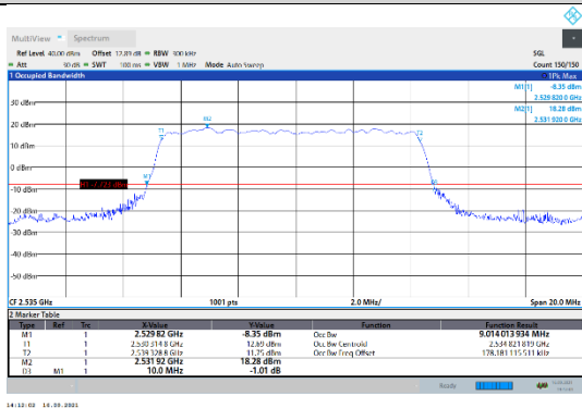
N7-15kHz-10MHz-DFT-64QAM-Mid-Outer_Full--- PASS
