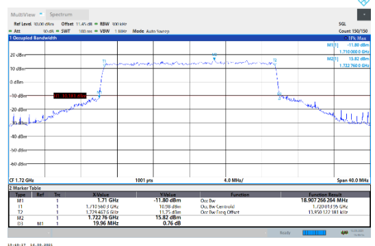
N66-15kHz-20MHz-CP-QPSK-Low-Outer_Full---PASS
