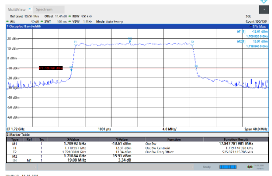
N66-15kHz-20MHz-DFT-64QAM-Low-Outer_Full---PASS
