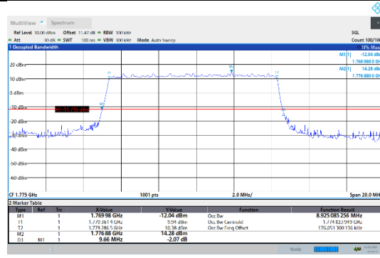
N66-15kHz-10MHz-DFT-64QAM-High-Outer_Full---PASS
