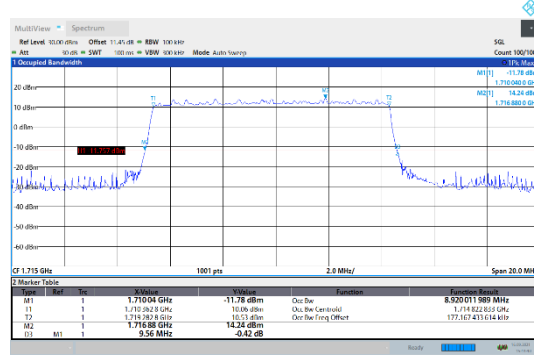
N66-15kHz-10MHz-DFT-64QAM-Low-Outer_Full---PASS
