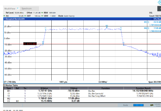
N66-15kHz-15MHz-CP-QPSK-Mid-Outer_Full---PASS
