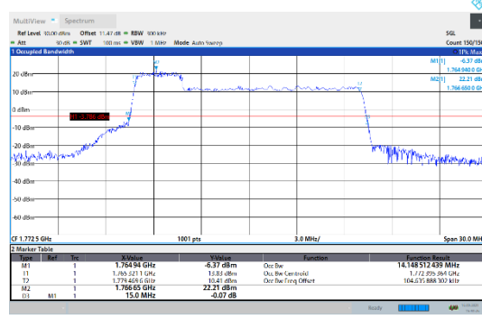
N66-15kHz-15MHz-CP-256QAM-High-Outer_Full---PASS
