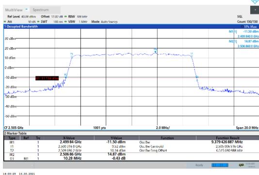
N7-15kHz-10MHz-CP-256QAM-Low-Outer_Full---PASS
