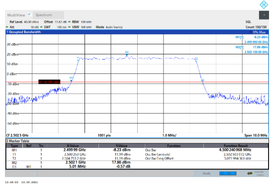
N7-15kHz-5MHz-DFT-16QAM-Low-Outer_Full---PASS
