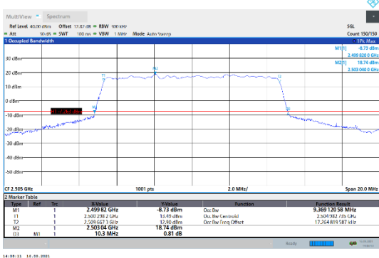
N7-15kHz-10MHz-CP-16QAM-Low-Outer_Full---PASS
