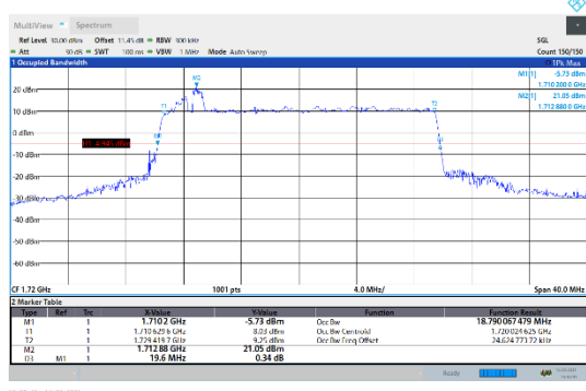
N66-15kHz-20MHz-CP-256QAM-Low-Outer_Full--- PASS
