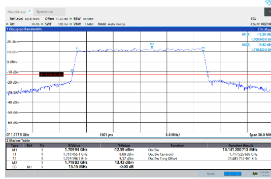
N66-15kHz-15MHz-CP-256QAM-Low-Outer_Full---PASS
