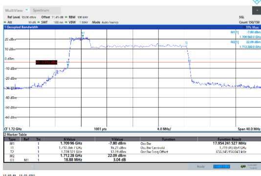
N66-15kHz-20MHz-DFT-256QAM-Low-Outer_Full--- PASS
