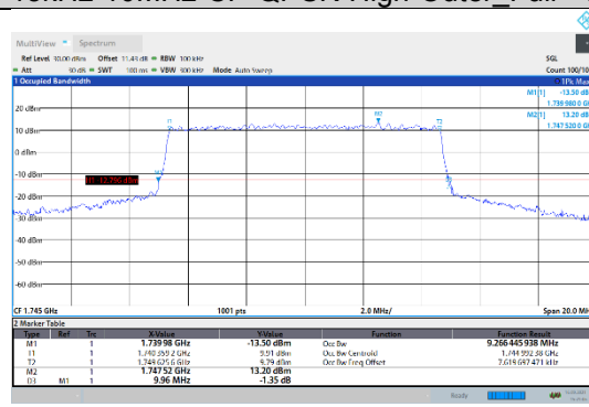
N66-15kHz-10MHz-CP-16QAM-Mid-Outer_Full--- PASS
