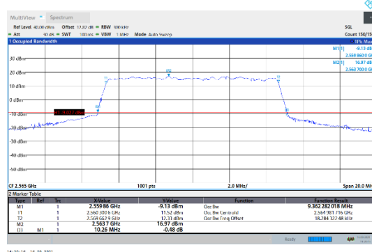
N7-15kHz-10MHz-CP-64QAM-High-Outer_Full---PASS
