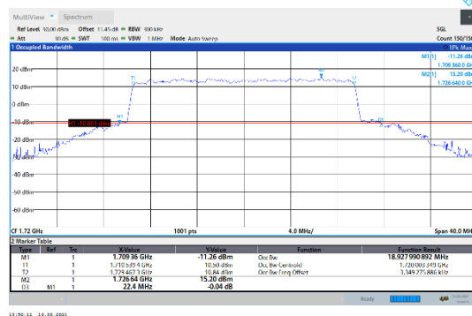
N66-15kHz-20MHz-CP-64QAM-Low-Outer_Full--- PASS
