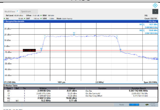
N7-15kHz-10MHz-CP-QPSK-Low-Outer_Full---PASS
