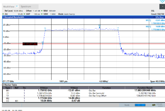
N66-15kHz-20MHz-DFT-256QAM-High-Outer_Full--- PASS
