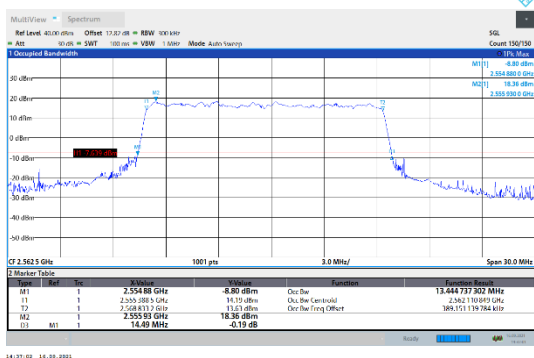
N7-15kHz-15MHz-DFT-QPSK-High-Outer_Full---PASS
