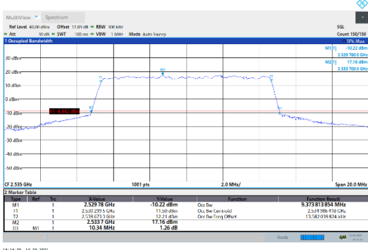
N7-15kHz-10MHz-CP-64QAM-Mid-Outer_Full---PASS
