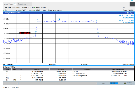
N66-15kHz-20MHz-DFT-16QAM-Mid-Outer_Full---PASS
