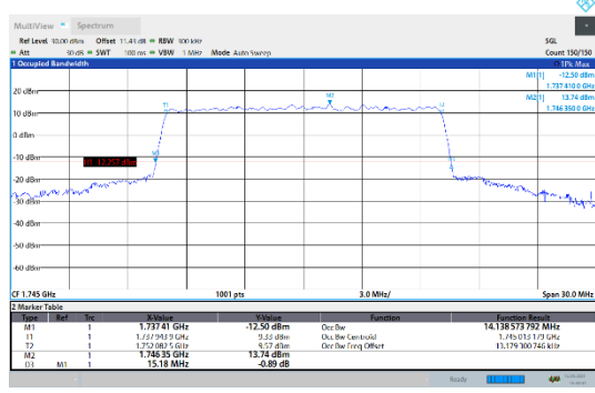
N66-15kHz-15MHz-CP-256QAM-Mid-Outer_Full---PASS
