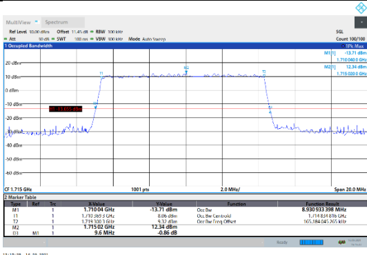
N66-15kHz-10MHz-DFT-256QAM-Low-Outer_Full--- PASS
