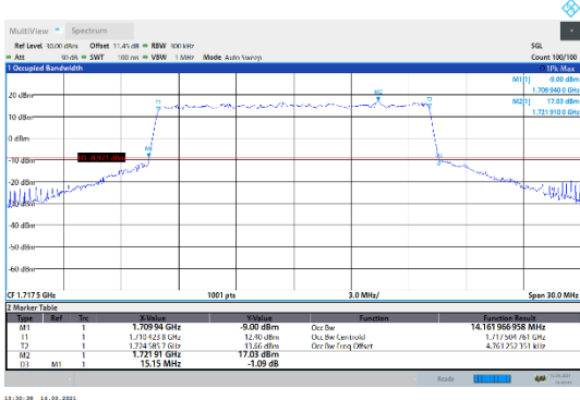
N66-15kHz-15MHz-CP-QPSK-Low-Outer_Full---PASS
