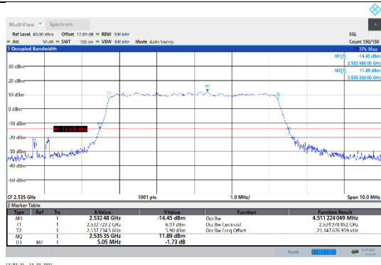
N7-15kHz-5MHz-CP-256QAM-Mid-Outer_Full---PASS
