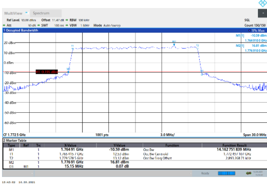
N66-15kHz-15MHz-CP-QPSK-High-Outer_Full---PASS
