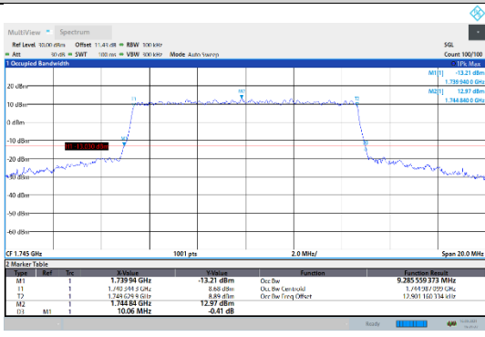
N66-15kHz-10MHz-CP-64QAM-Mid-Outer_Full--- PASS
