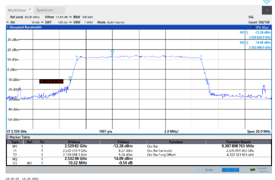
N7-15kHz-10MHz-CP-256QAM-Mid-Outer_Full---PASS
