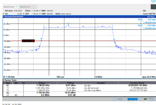
N66-15kHz-10MHz-DFT-QPSK-Mid-Outer_Full---PASS
