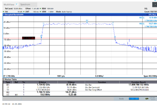
N66-15kHz-20MHz-DFT-QPSK-Mid-Outer_Full---PASS
