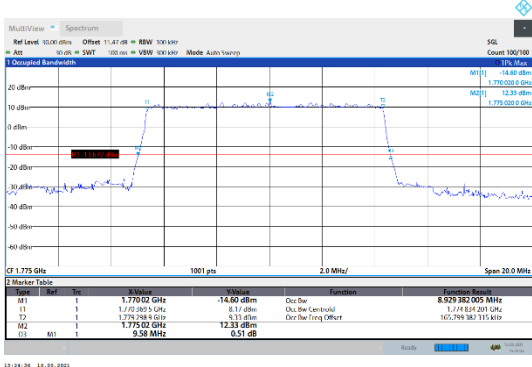
N66-15kHz-10MHz-DFT-256QAM-High-Outer_Full--- PASS
