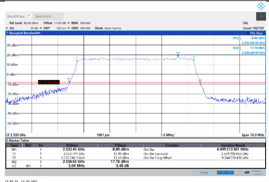
N7-15kHz-5MHz-DFT-QPSK-Mid-Outer_Full---PASS
