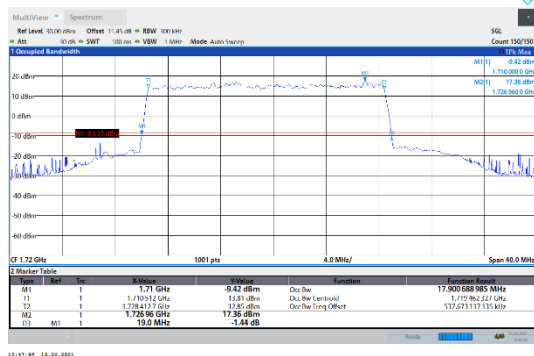
N66-15kHz-20MHz-DFT-16QAM-Low-Outer_Full---PASS
