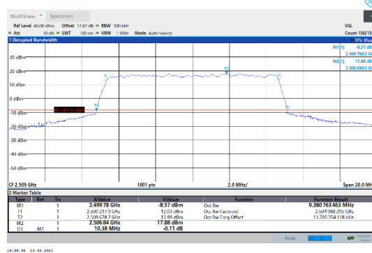
N7-15kHz-10MHz-CP-64QAM-Low-Outer_Full---PASS
