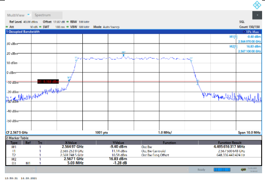
N7-15kHz-5MHz-DFT-16QAM-High-Outer_Full---PASS
