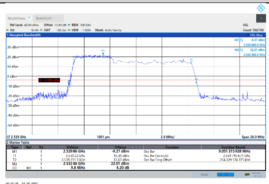
N7-15kHz-10MHz-DFT-256QAM-Mid-Outer_Full--- PASS
