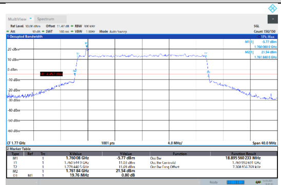
N66-15kHz-20MHz-CP-QPSK-High-Outer_Full---PASS
