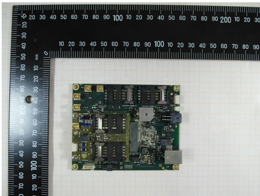
Photo 2: top view of the main PCB
