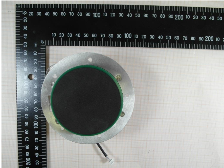
Photo 9: top view of the disassembled wifi PCB-antenna
