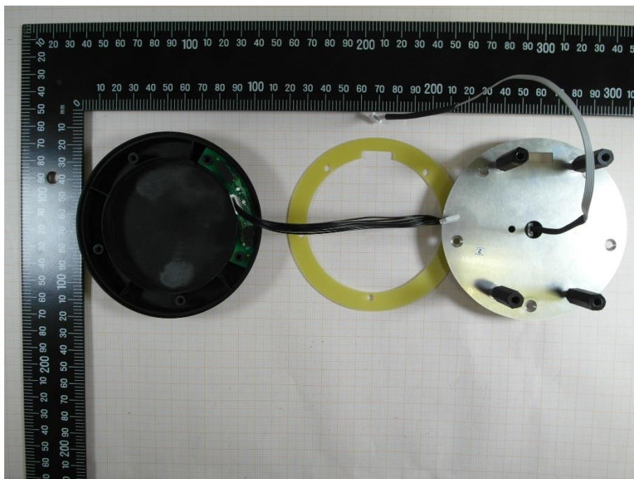
Photo 10: bottom view of the disassembled wifi PCB-antenna
