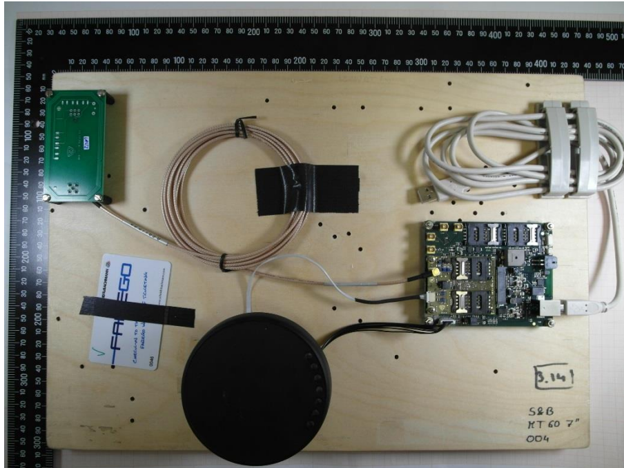
Photo 1: summary of the test arrangement board
