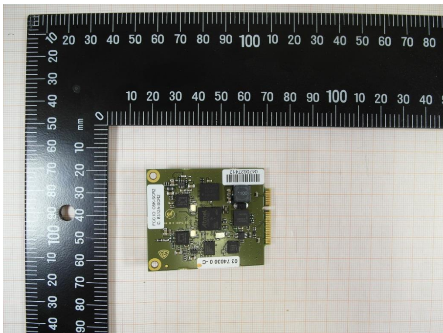
Photo 6: bottom view of the RF module
