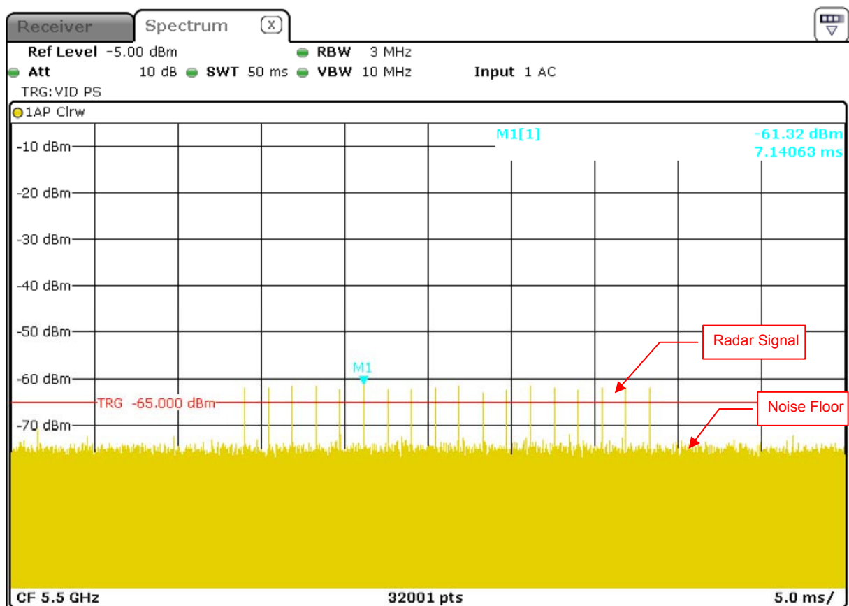
Radar Signal 0
