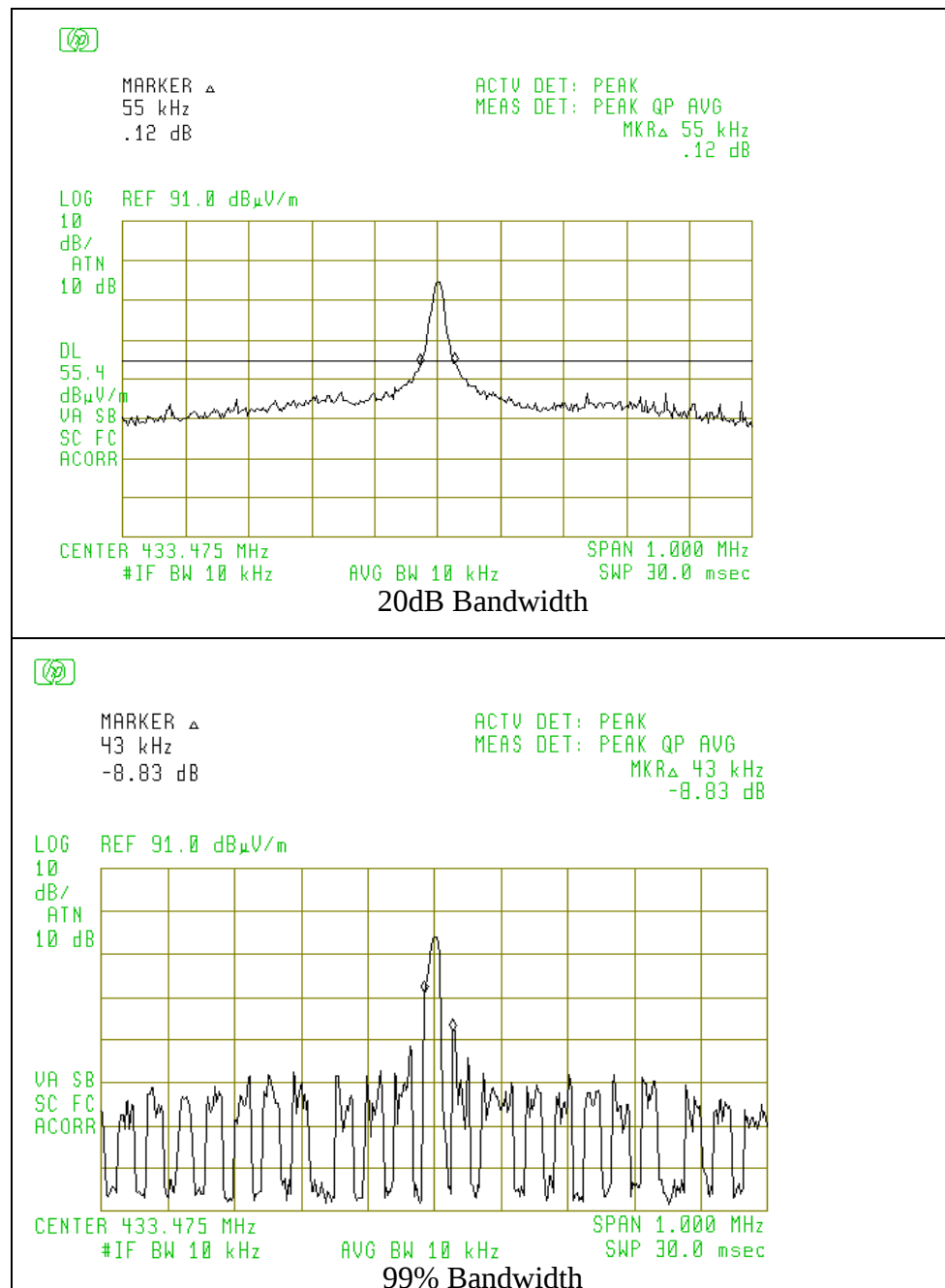
Figure 6.1 Occupied Bandwidth
