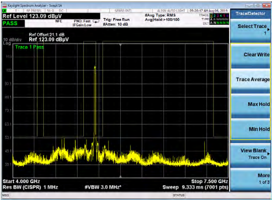
5335 MHz_20 Mhz Channel_J3
