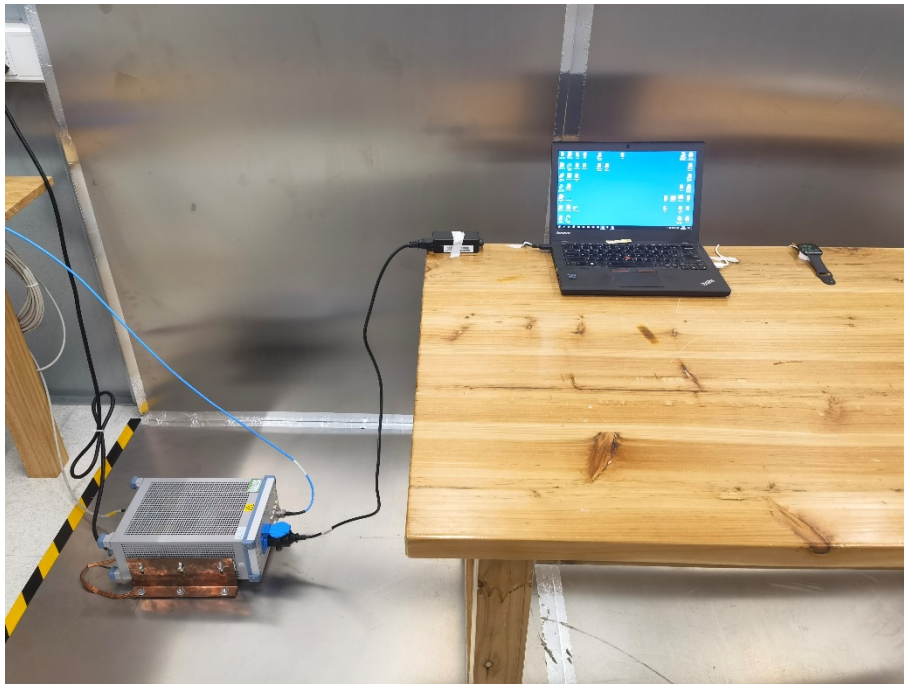
Photograph 3: Set-up photo for Conducted Emission
