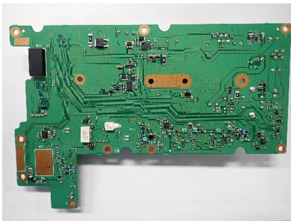
MAIN-D (BOTTOM)
