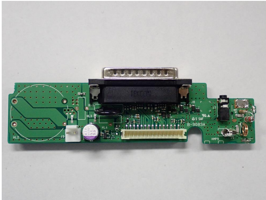
D-CONNECT-B(TOP)
