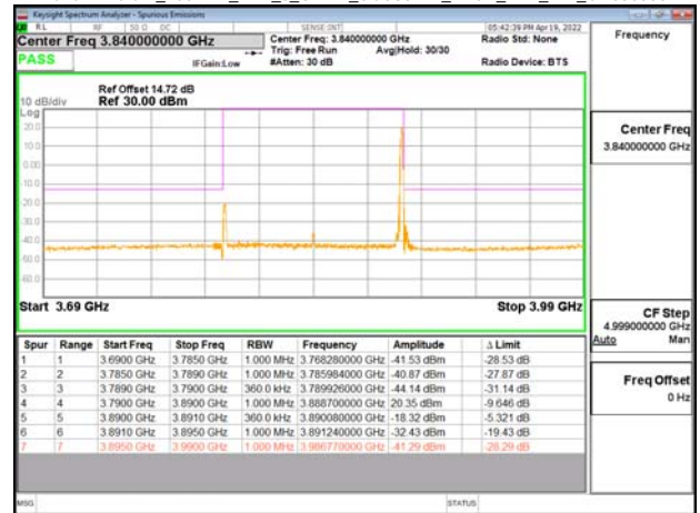
Band77-Part27_100MHz_DFT_s_OFDM_SCS30kHz_BPSK_RB1_272_CH662000
