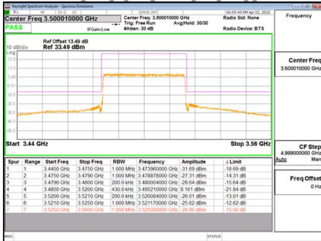
Band77-Part27_40MHz_CP_OFDM_SCS30kHz_OPSK_RB106_0_CH633332
