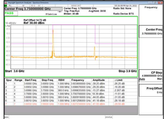
Band77-Part27_100MHz_CP_OFDM_SCS30kHz_QPSK_RB1_0_CH650000
