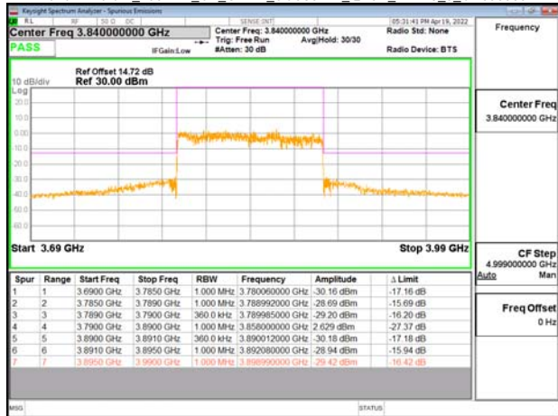
Band77-Part27_100MHz_CP_OFDM_SCS30kHz_QPSK_RB273_0_CH656000
