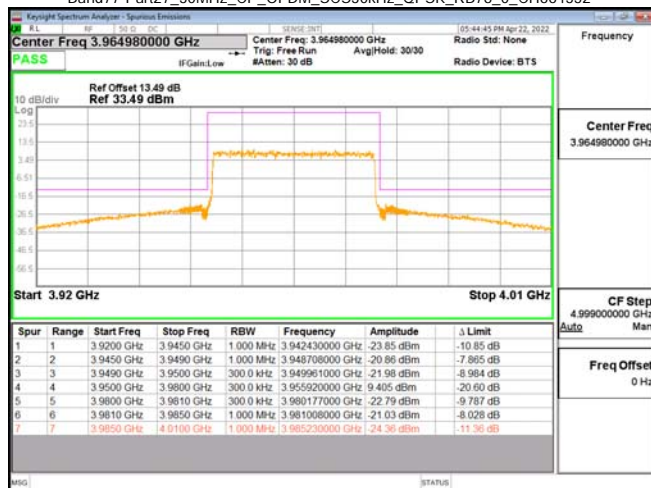
Band77-Part27_30MHz_CP_OFDM_SCS30kHz_QPSK_RB78_0_CH664332
