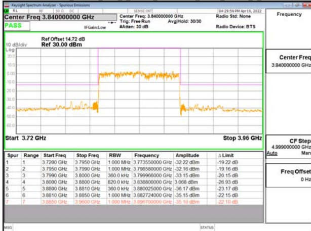
Band77-Part27_80MHz_DFT_s_OFDM_SCS30kHz_BPSK_RB216_0_CH656000
