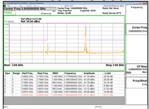
Band77-Part27_100MHz_CP_OFDM_SCS30kHz_QPSK_RB1_272_CH62000
