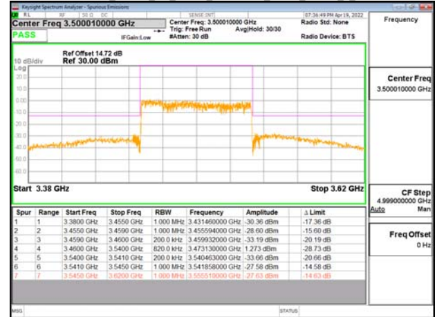
Band77-Part27_80MHz_CP_OFDM_SCS30kHz_OPSK_RB217_0_CH633334
