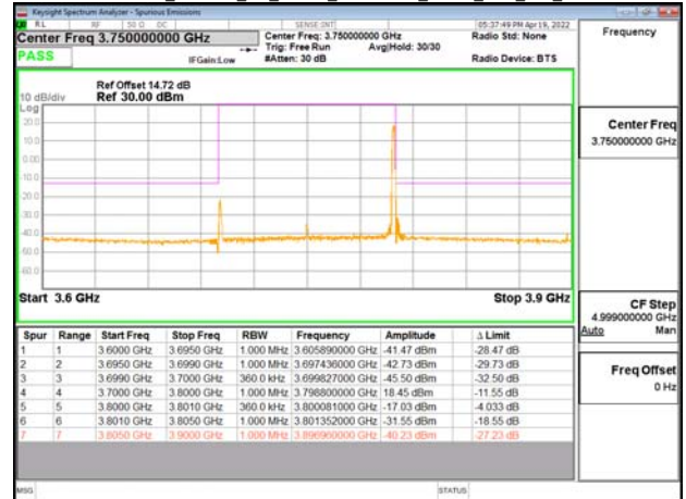
Band77-Part27_100MHz_CP_OFDM_SCS30kHz_QPSK_RB1_272_CH656000
