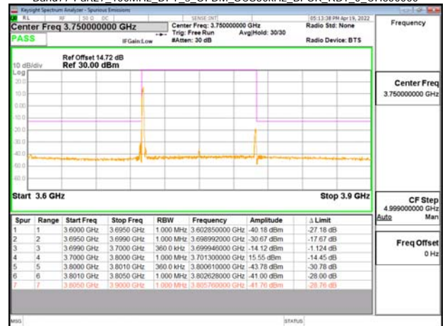
Band77-Part27_100MHz_DFT_s_OFDM_SCS30kHz_BPSK_RB1_0_CH650000
