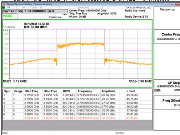
Band77-Part27_80MHz_CP_OFDM_SCS30kHz_OPSK_RB217_0_CH656000
