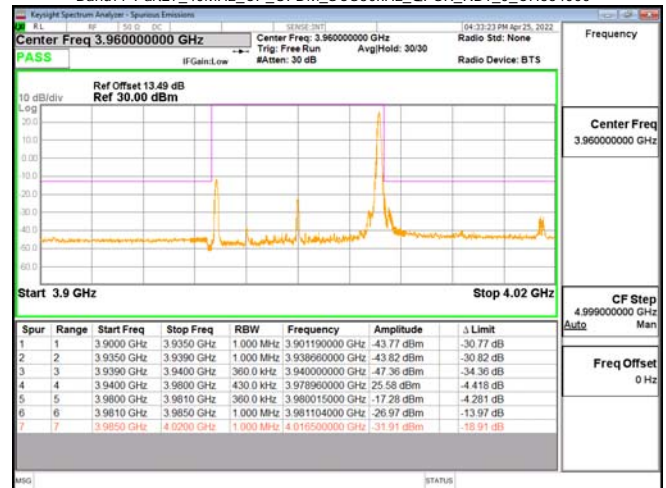
Band77-Part27_40MHz_CP_OFDM_SCS30kHz_QPSK_RB1_0_CH664000
