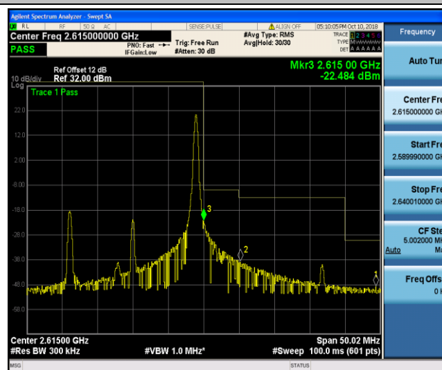
Band41_20MHz_16QAM_40740_1RB#99
