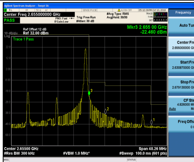
Band41_20MHz_QPSK_41140_1RB#99
