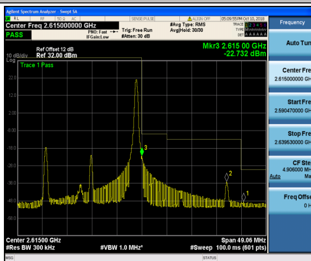
Band41_20MHz_QPSK_40740_1RB#99
