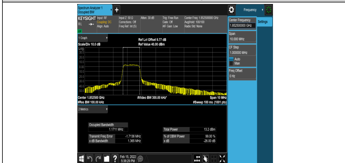
Band25-5MHz-QPSK-26065-6-0-Low-1.1711-1.365-PASS
