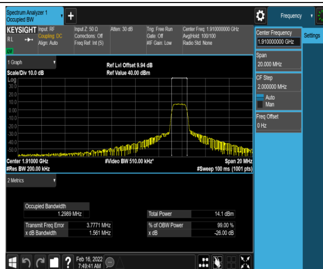
Band25-10MHz-16QAM-26640-6-0-High-1.2989-1.561-PASS
