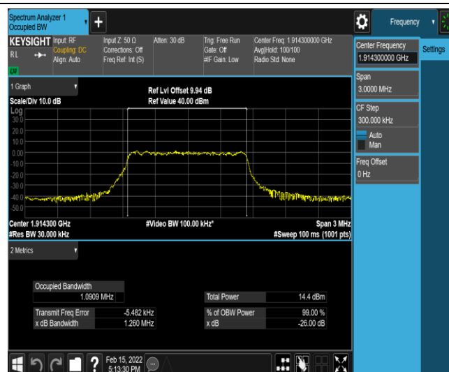
Band25-1.4MHz-QPSK-26683-6-0-High-1.0909-1.260-PASS
