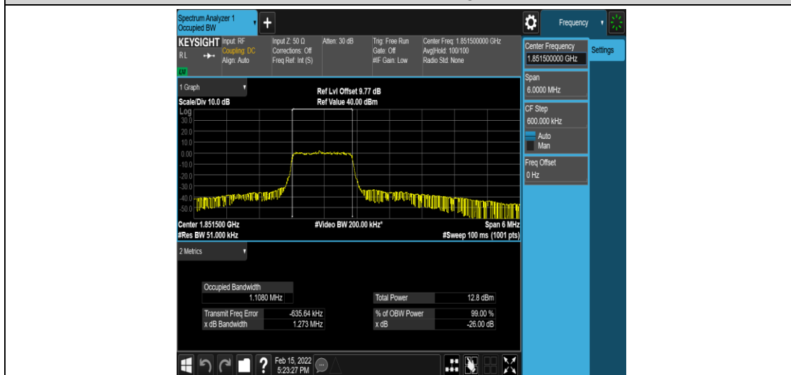
Band25-3MHz-QPSK-26055-6-0-Low-1.1080-1.273-PASS
