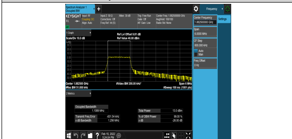
Band25-3MHz-QPSK-26365-6-0-Low-1.1089-1.256-PASS
