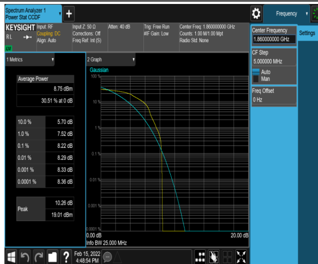
Band25-20MHz-16QAM-26140-1-0-Low-8.22-&lt;=13-PASS
