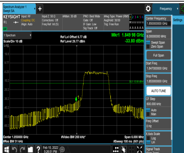
Band25-3MHz-QPSK-26055-6-0-Low--33.80-PASS
