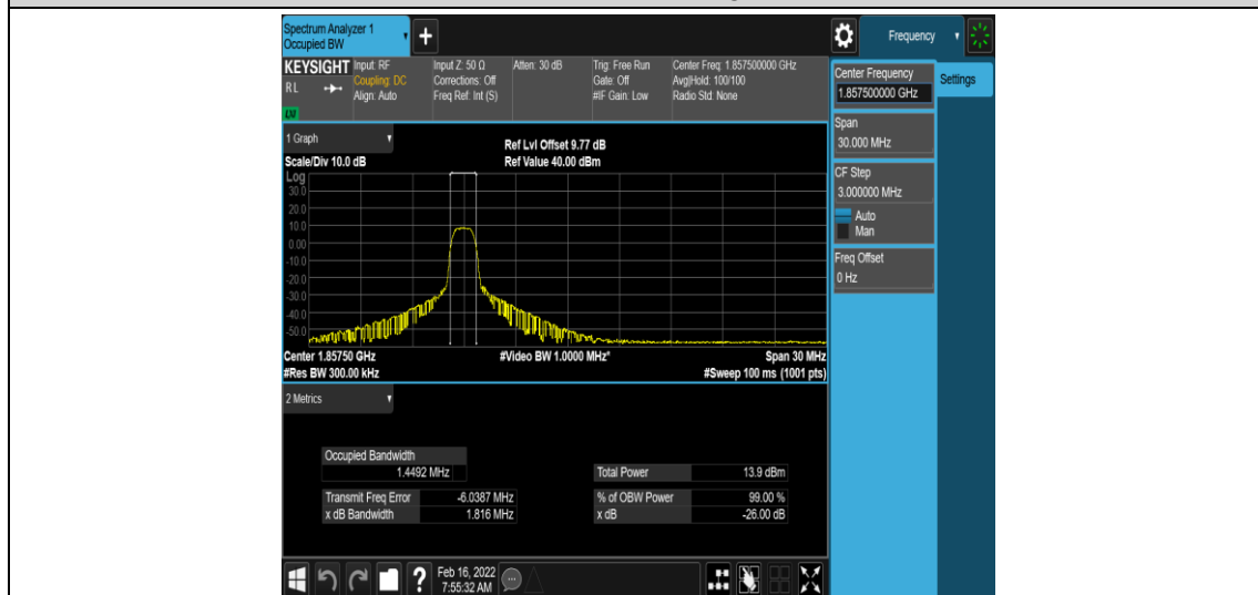
Band25-15MHz-16QAM-26115-6-0-Low-1.4492-1.816-PASS
