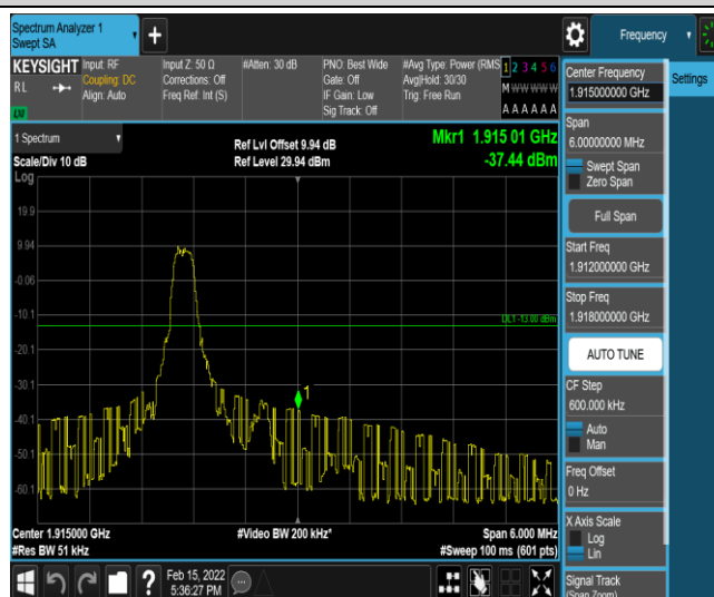
Band25-3MHz-QPSK-26675-1-0-High--37.44-PASS
