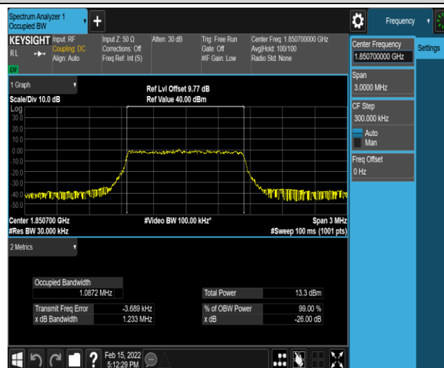
Band25-1.4MHz-16QAM-26047-6-0-Low-1.0872-1.233-PASS
