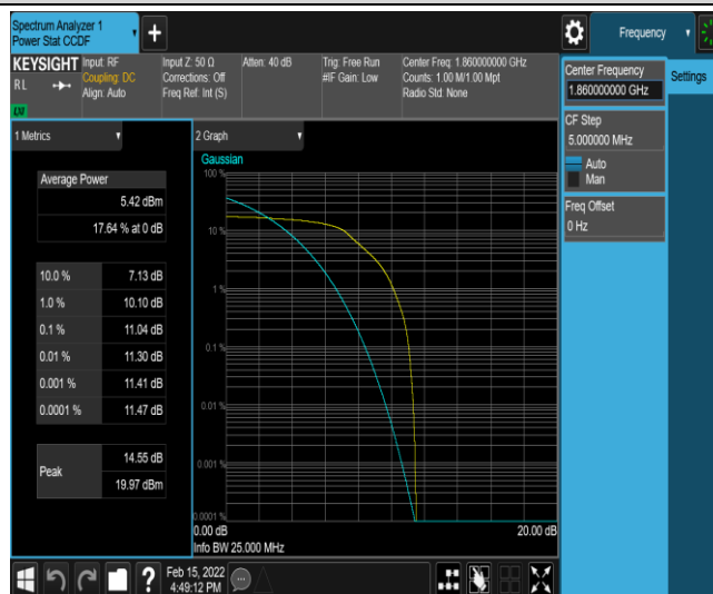
Band25-20MHz-16QAM-26140-6-0-Low-11.04-&lt;=13-PASS
