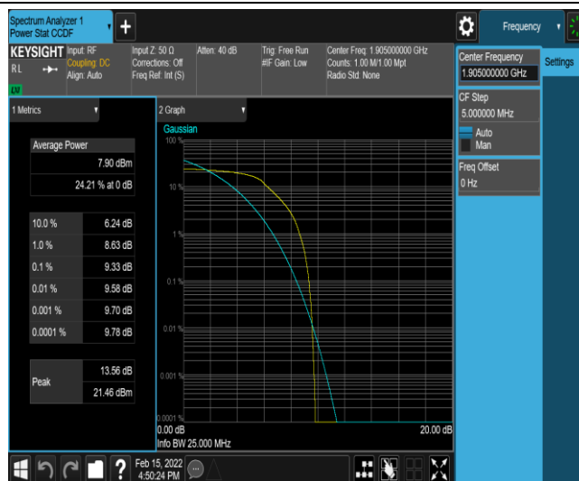
Band25-20MHz-QPSK-26590-6-0-High-9.33-&lt;=13-PASS
