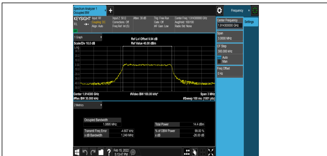
Band25-1.4MHz-16QAM-26683-6-0-High-1.0895-1.249-PASS
