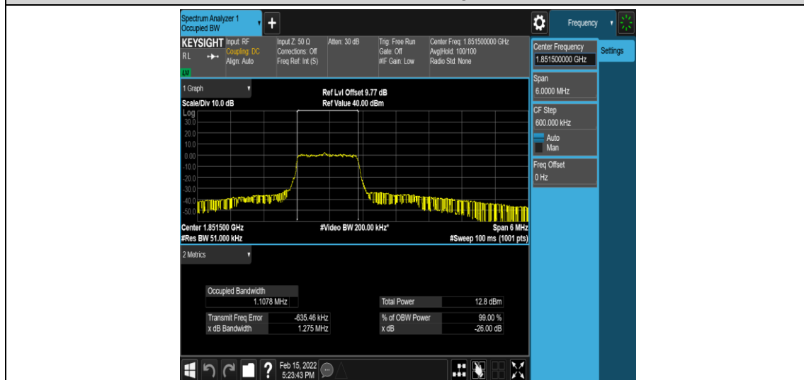
Band25-3MHz-16QAM-26055-6-0-Low-1.1078-1.275-PASS
