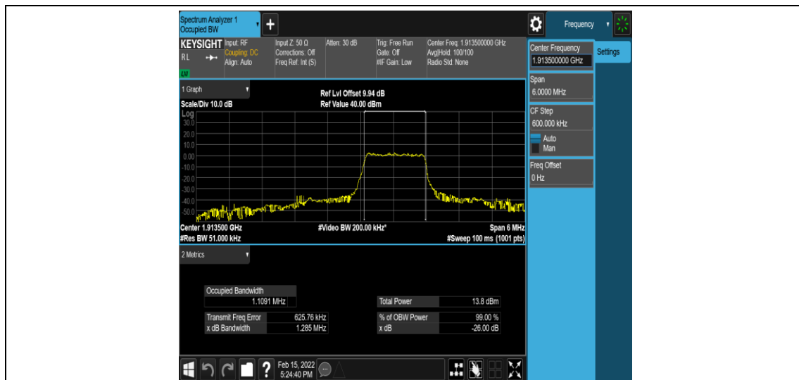
Band25-3MHz-QPSK-26675-6-0-High-1.1091-1.285-PASS
