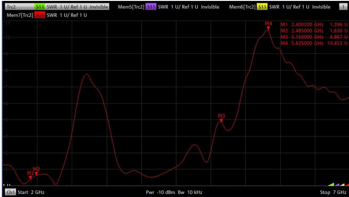
WiFi Antenna
