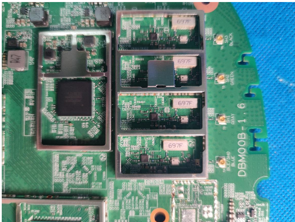
(4) EUT Photo(AP410C)
