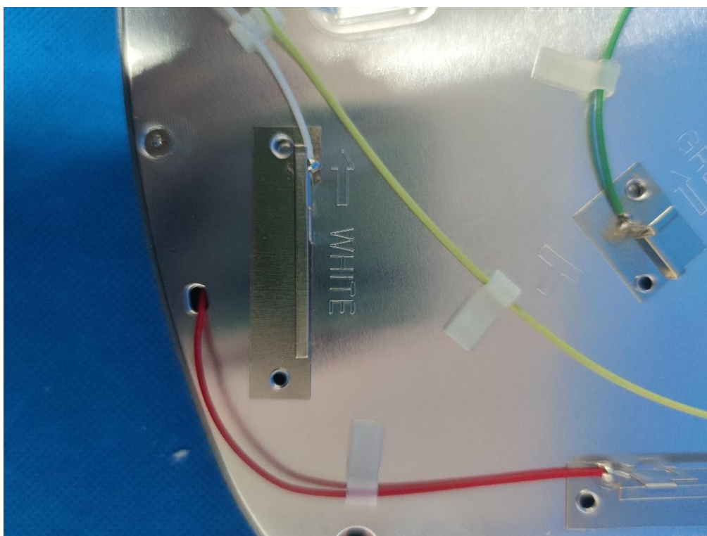
(13) EUT Photo(AP410C)
