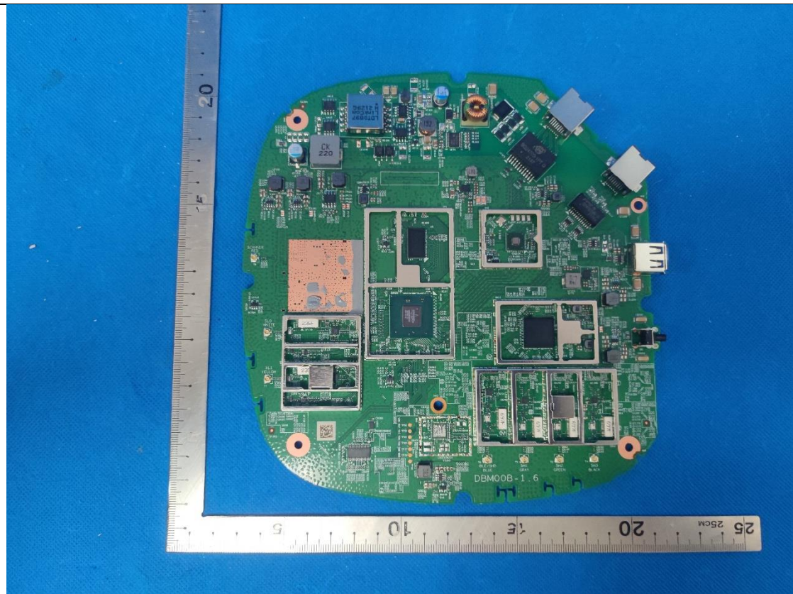
(4) EUT Photo(AP410C)
