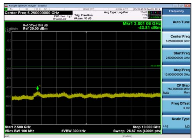
,Plot 4,2500MHz~10000MHz-802.11n(HT40 ) ,2452MHz,Ant1
