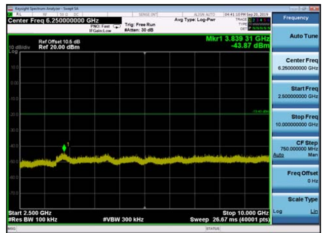
,Plot 4,2500MHz~10000MHz-802.11n(HT40 ) ,2437MHz,Ant1
