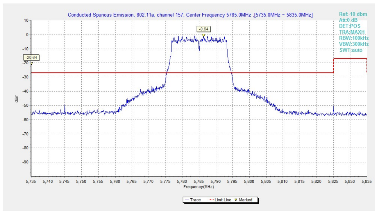
Fig. 12 Conducted Spurious Emission (802.11a, Ch157, Center Frequency)
