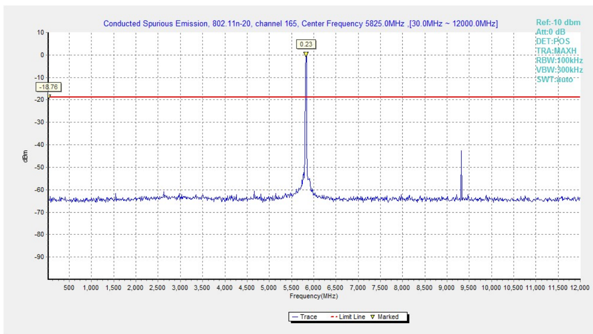
Fig. 27 Conducted Spurious Emission (802.11n-HT20, Ch165, 30 MHz-12 GHz)
