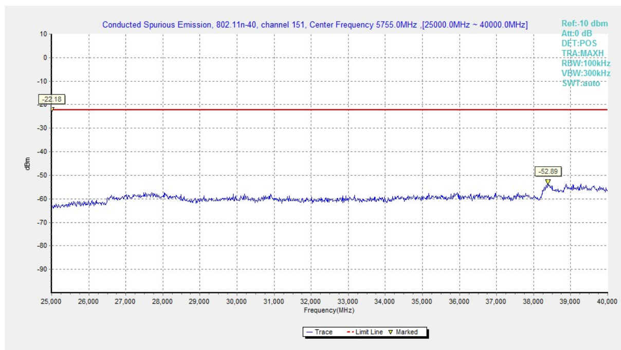
Fig. 33 Conducted Spurious Emission (802.11n-HT40, Ch151, 25 GHz-40 GHz)
