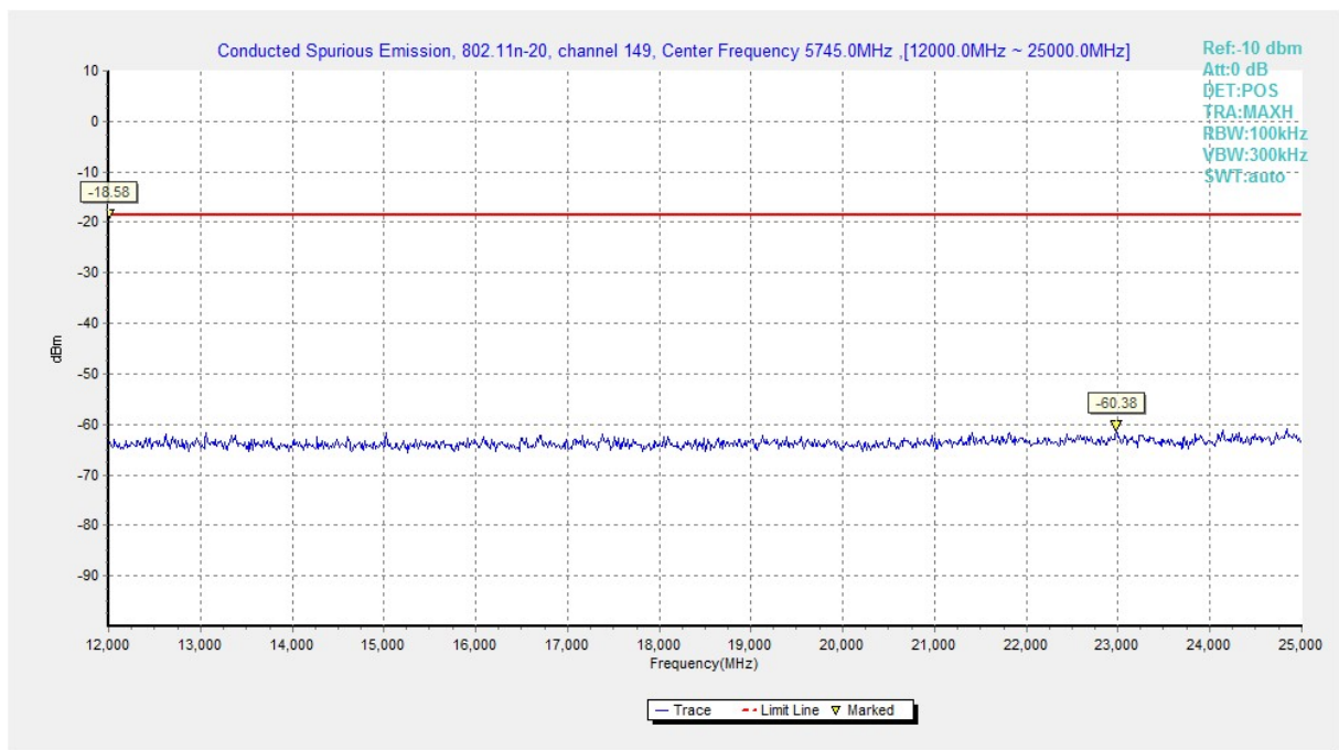
Fig. 20 Conducted Spurious Emission (802.11n-HT20, Ch149, 12 GHz-25 GHz)
