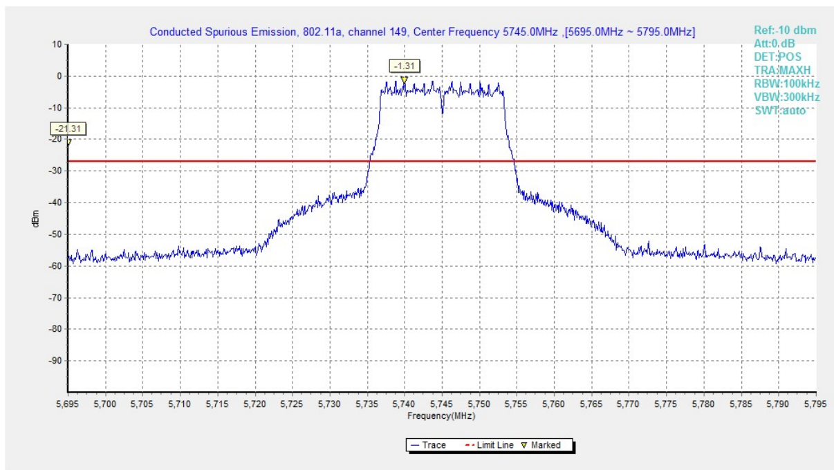
Fig. 9 Conducted Spurious Emission (802.11a, Ch149, Center Frequency)
