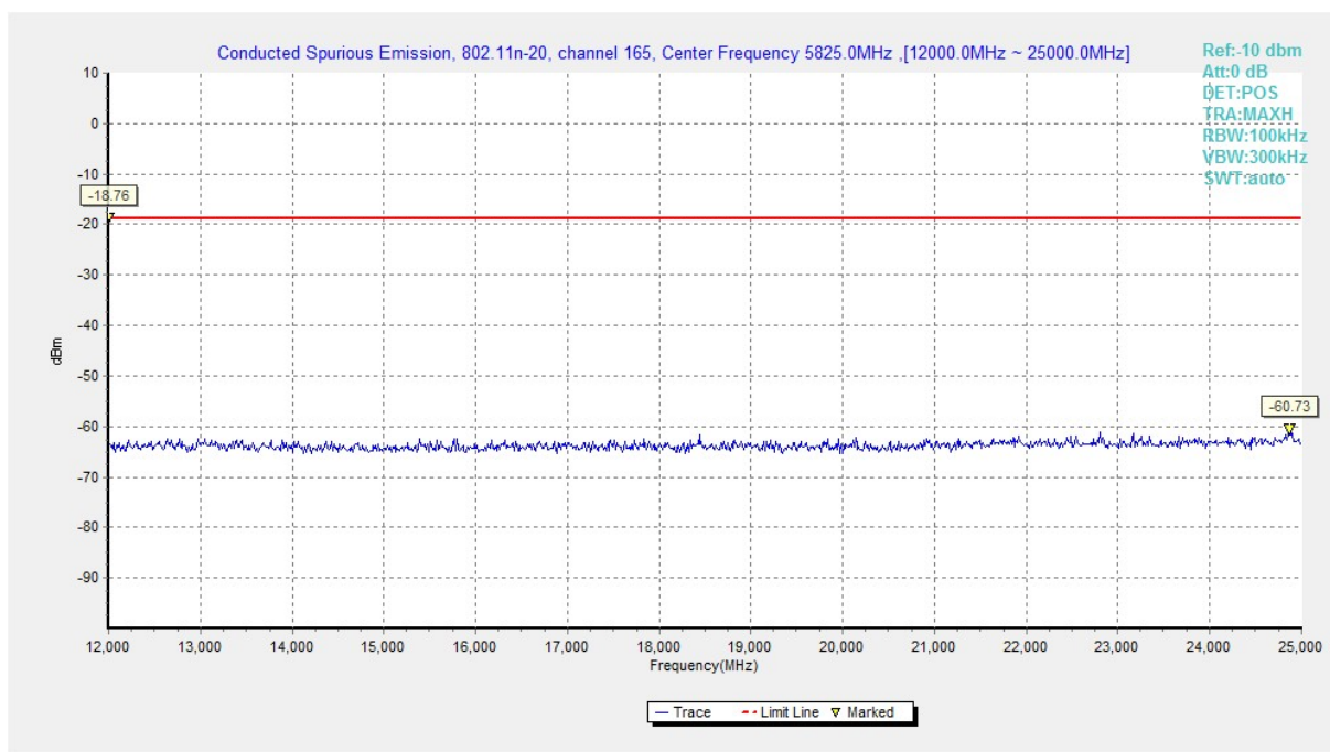
Fig. 28 Conducted Spurious Emission (802.11n-HT20, Ch165, 12 GHz-25 GHz)
