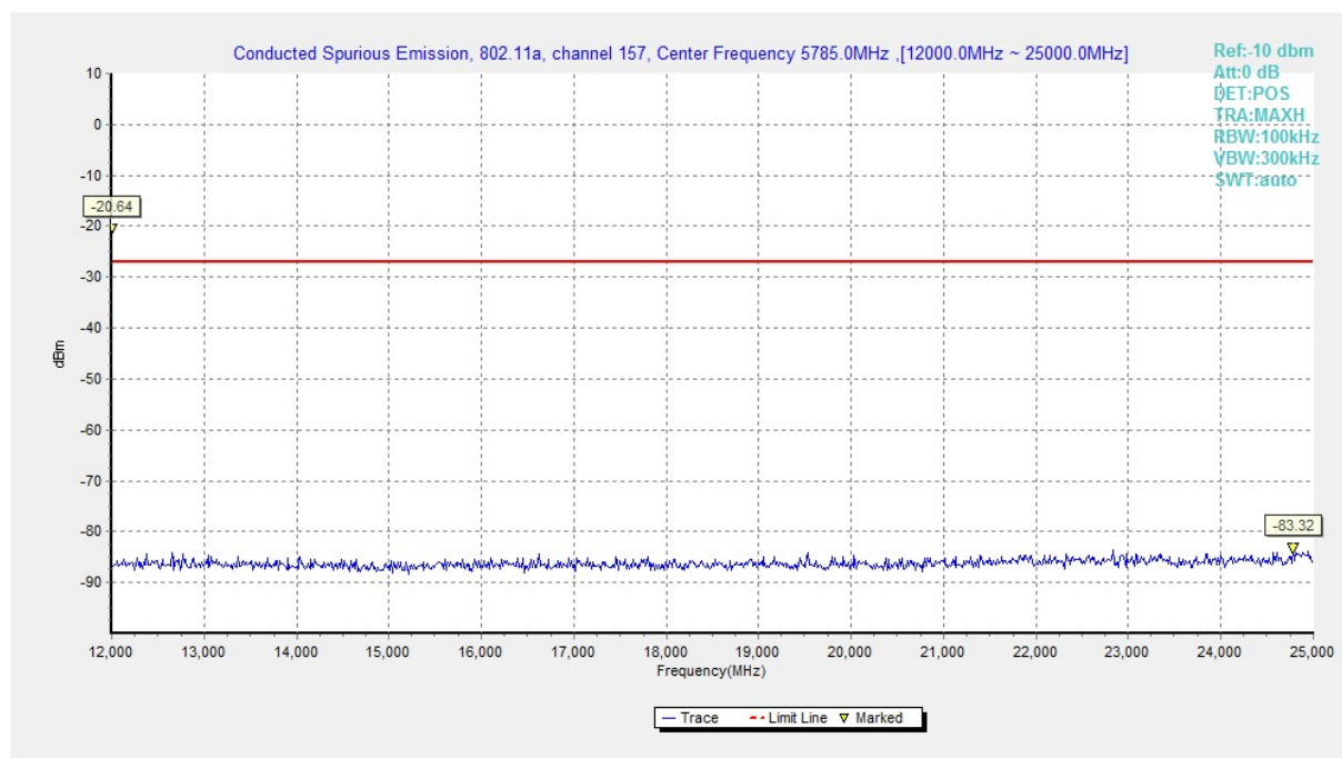
Fig. 14 Conducted Spurious Emission (802.11a, Ch157, 12 GHz-25 GHz)
