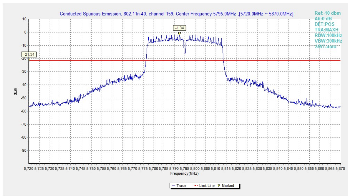
Fig. 34 Conducted Spurious Emission (802.11n-HT40, Ch159, Center Frequency)
