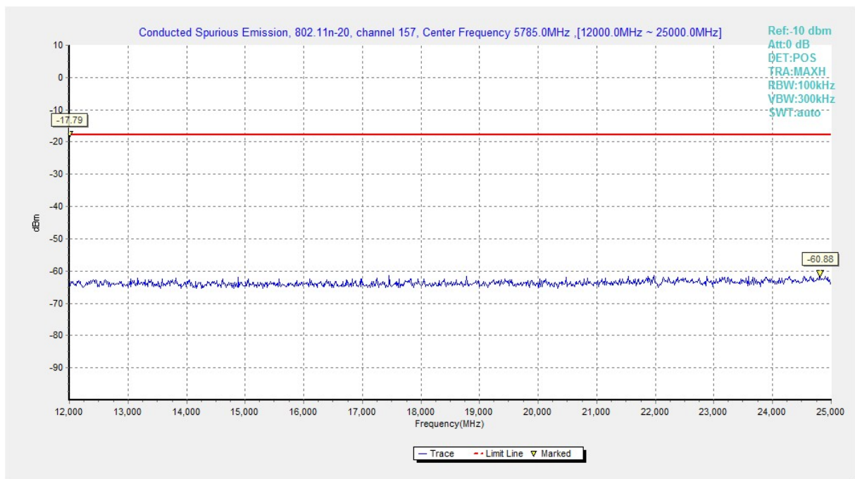
Fig. 24 Conducted Spurious Emission (802.11n-HT20, Ch157, 12 GHz-25 GHz)
