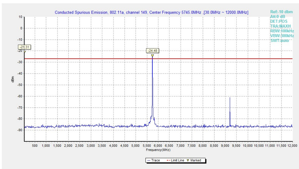
Fig. 10 Conducted Spurious Emission (802.11a, Ch149, 30 MHz-12 GHz)
