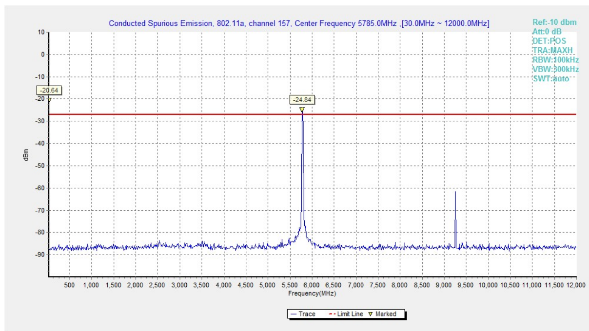
Fig. 13 Conducted Spurious Emission (802.11a, Ch157, 30 MHz-12 GHz)
