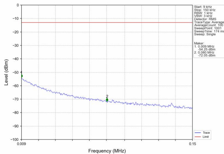
Band66_5MHz_16QAM_HCH_1777.5MHz_RB_1_0_NTNV
