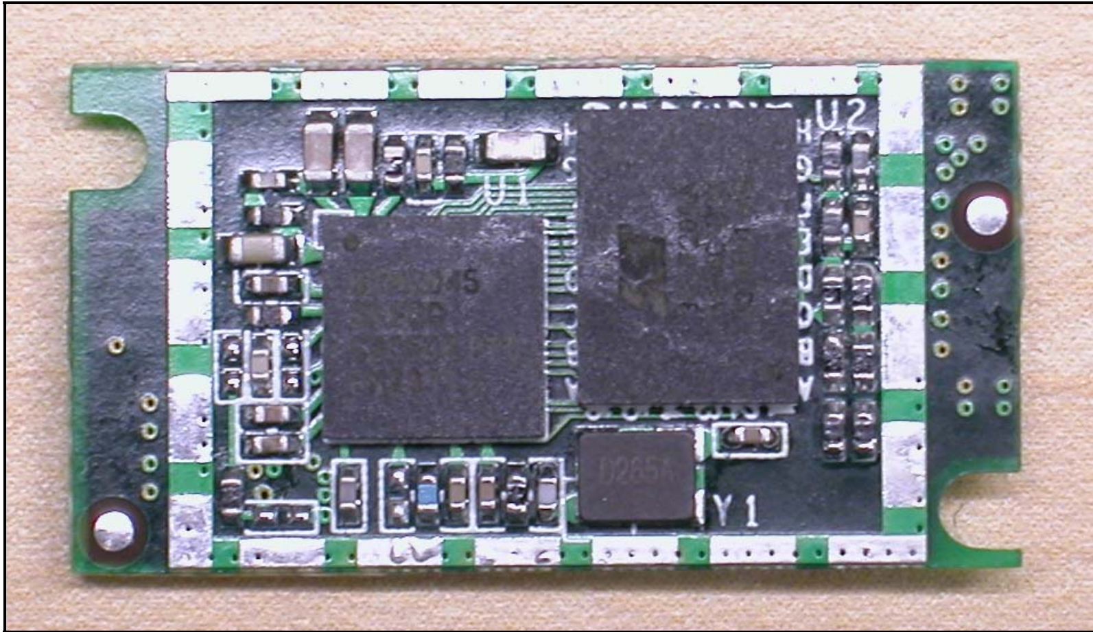
BCM92045NMD Internal Photos
