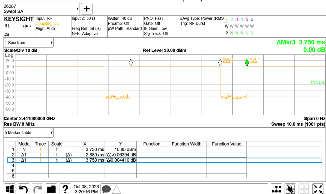
Bluetooth-BDR (DH5)
