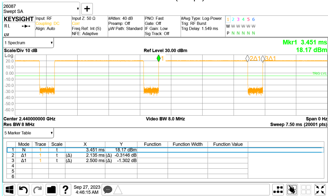
Bluetooth-LE (1Mbps)
