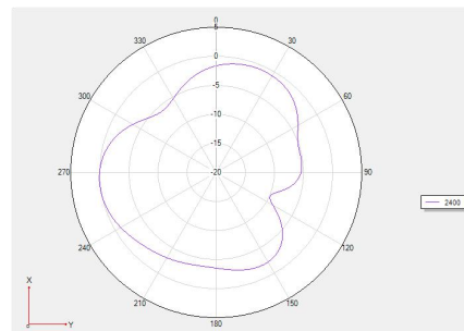
Theta =90 freq=2400MHz
