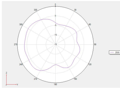
Phi =90 freq=2500MHz
