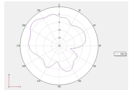
Theta =90 freq=5850MHz
