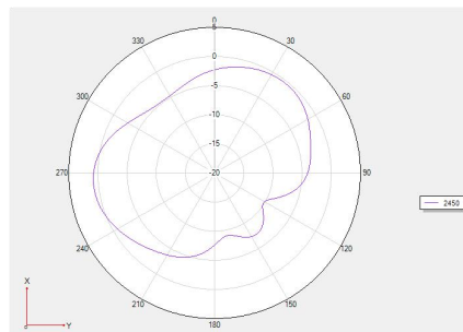
Theta =90 freq=2450MHz
