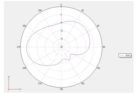
Theta =90 freq=2500MHz
