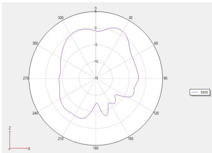
Phi =0 freq=5500MHz
