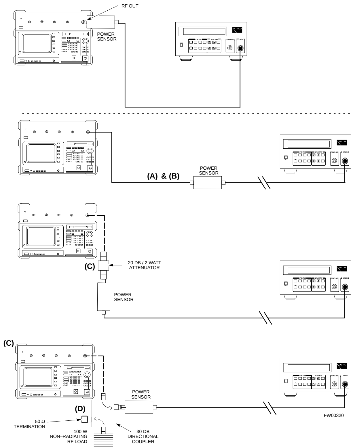
Figure F-8: Cable Calibration Using Advantest R3465
