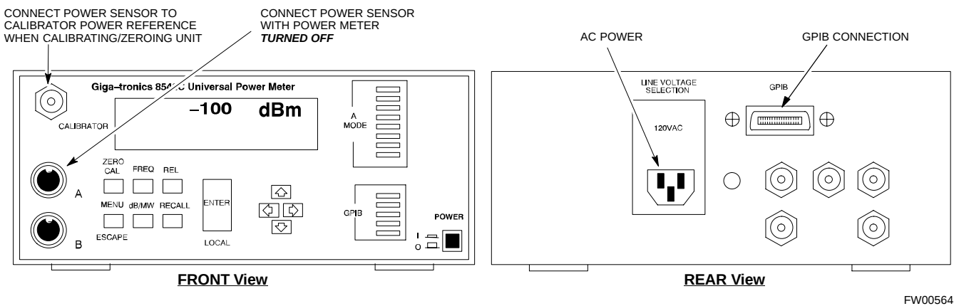
Figure F-6: Gigatronics 8542C Power Meter Detail
