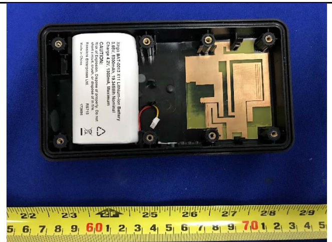
EUT battery and antenna
