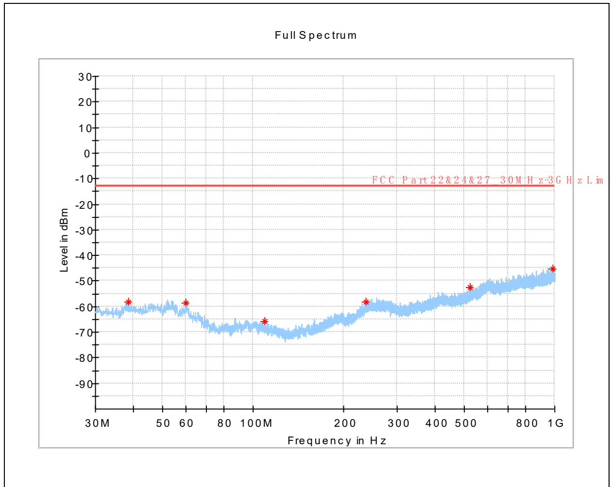
(LTE Band 17 _QPSK_ Low Channel _ 30MHz to 1GHz _ Horizontal)
