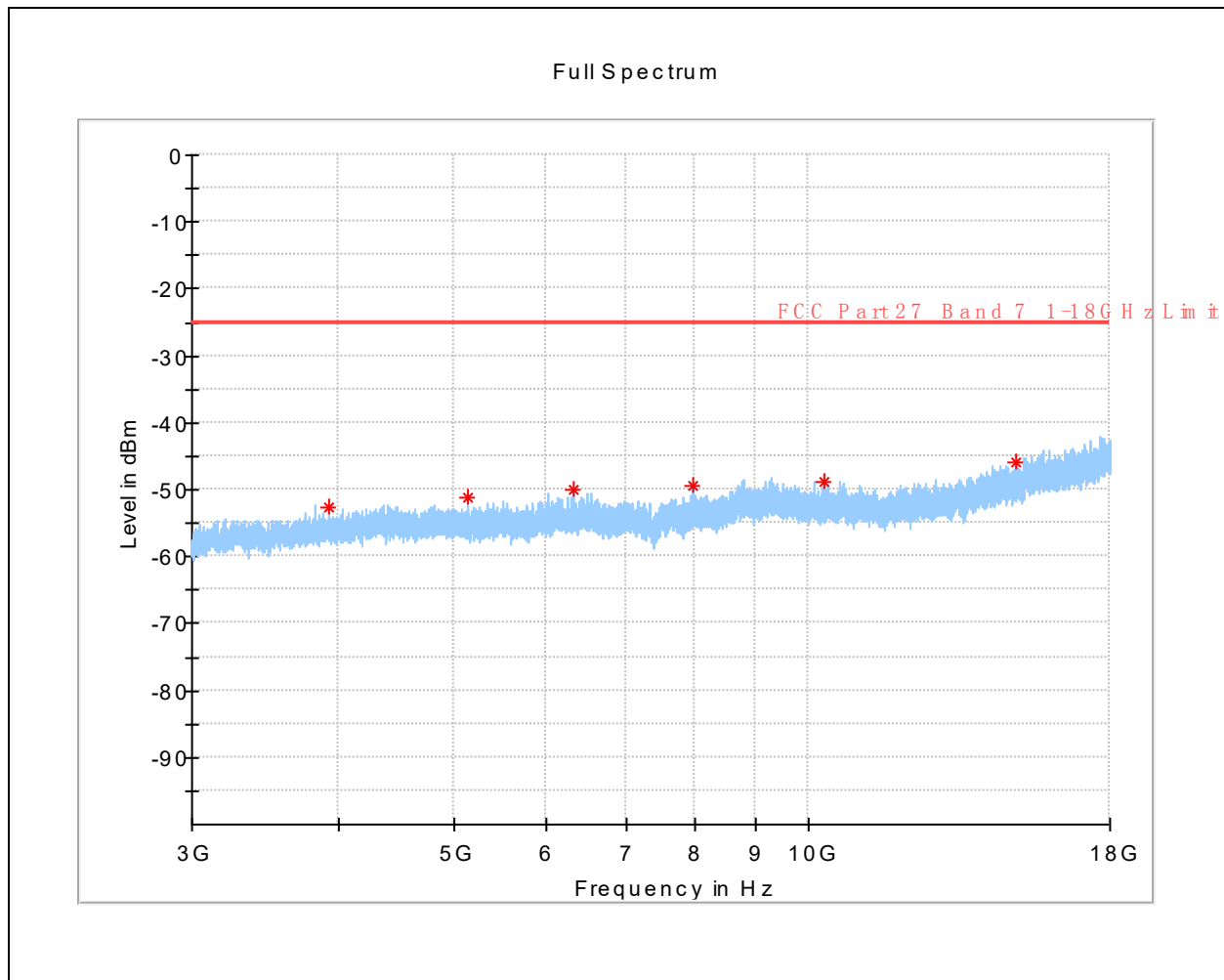
(LTE Band 7 _QPSK_ Middle Channel _ 3GHz to 18GHz _ Horizontal)
