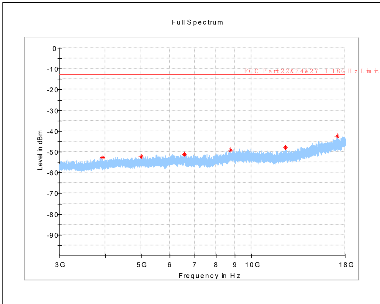
(LTE Band 25 _QPSK_ Low Channel _ 3GHz to 18GHz _ Horizontal)
