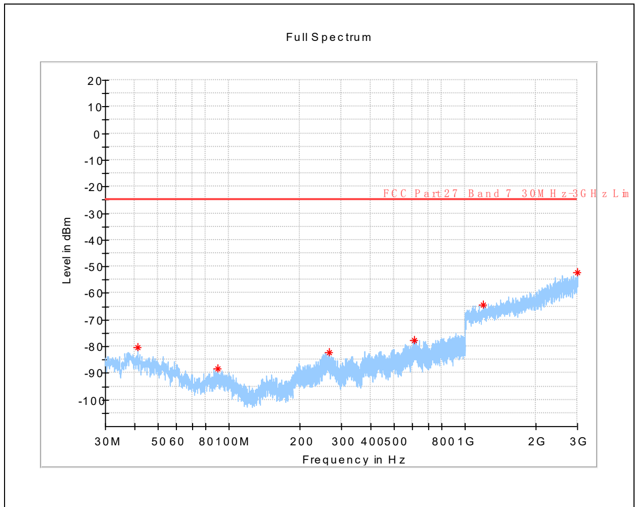
(LTE Band 7 _QPSK_ Middle Channel _ 30MHz to 3GHz _ Horizontal)
