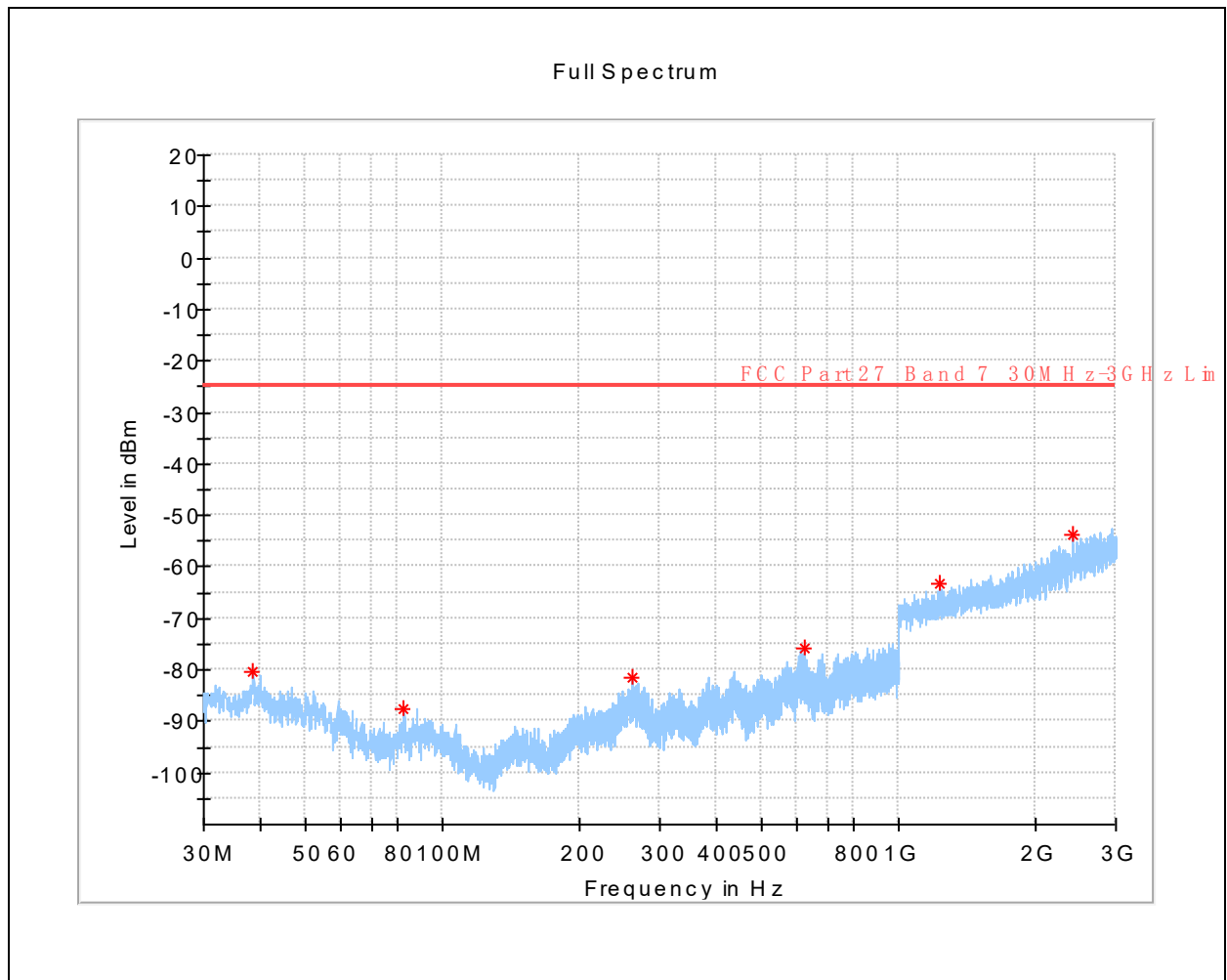
(LTE Band 7 _QPSK_ High Channel _ 30MHz to 3GHz _ Horizontal)
