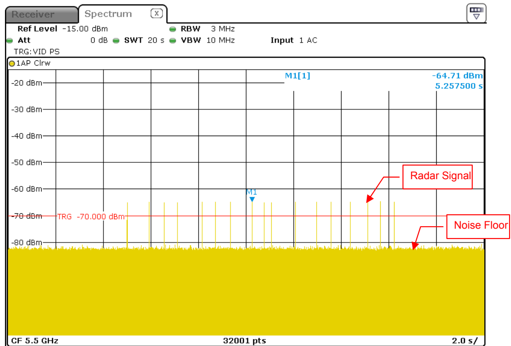
Radar Signal 5
