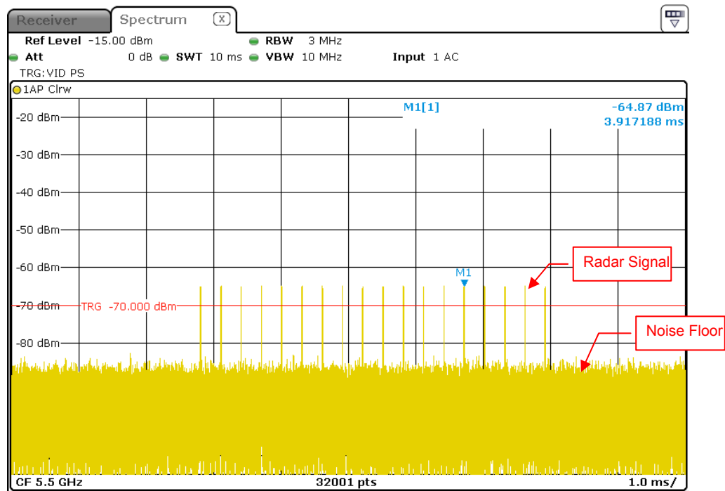
Radar Signal 3
