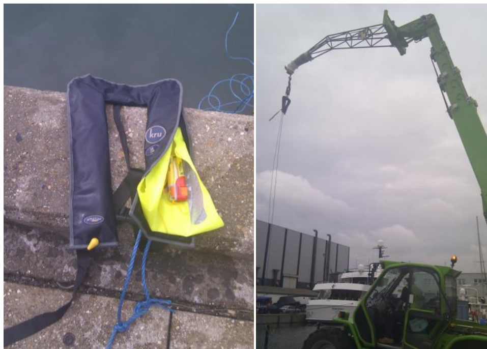
Test Set-up – Drop into Water Z501 installed in lifejacket and being hoisted by crane
