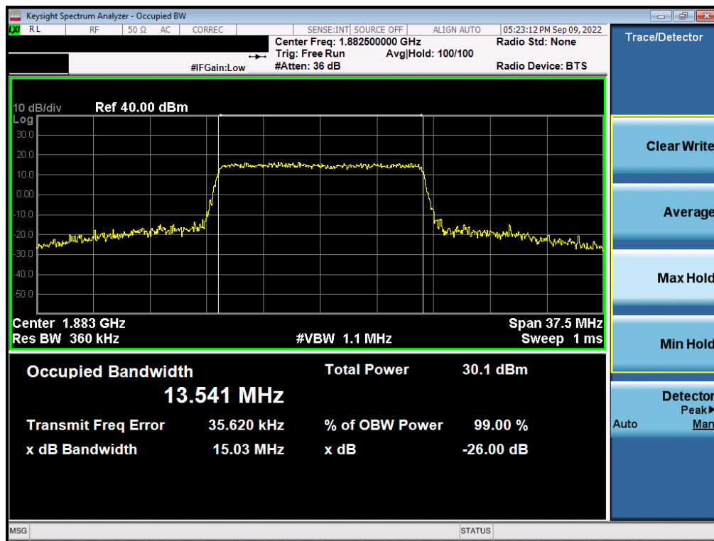
Plot 7-4. Occupied Bandwidth Plot (LTE Band 25/2 - 15MHz 16-QAM - Full RB - ANT A)
