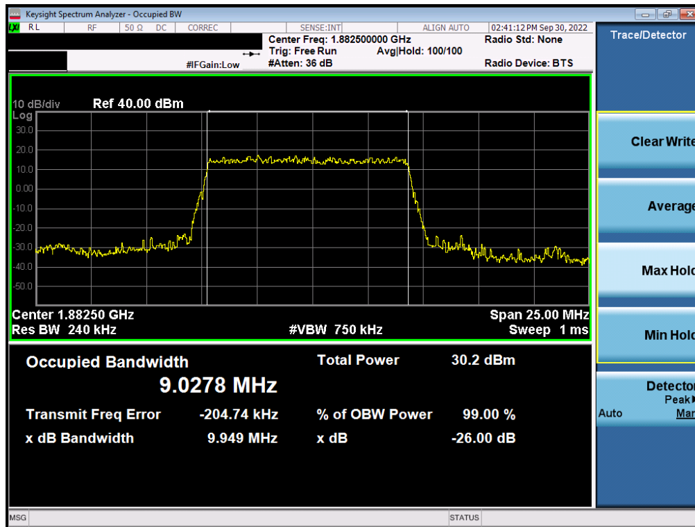
Plot 7-61. Occupied Bandwidth Plot (NR Band n25/2 - 10.0MHz DFT-s-OFDM BPSK - Full RB - ANT F)
