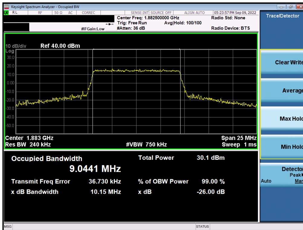
Plot 7-6. Occupied Bandwidth Plot (LTE Band 25/2 - 10MHz 16-QAM - Full RB - ANT A)
