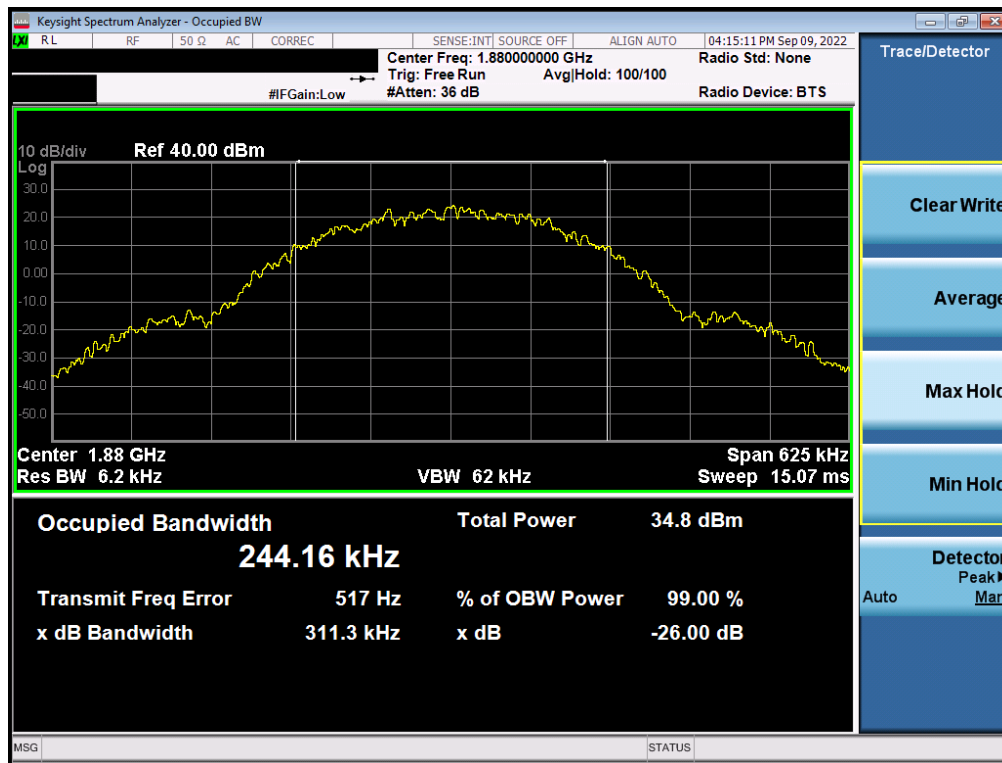
Plot 7-67. Occupied Bandwidth Plot (GPRS, Ch. 661 - ANT A)
