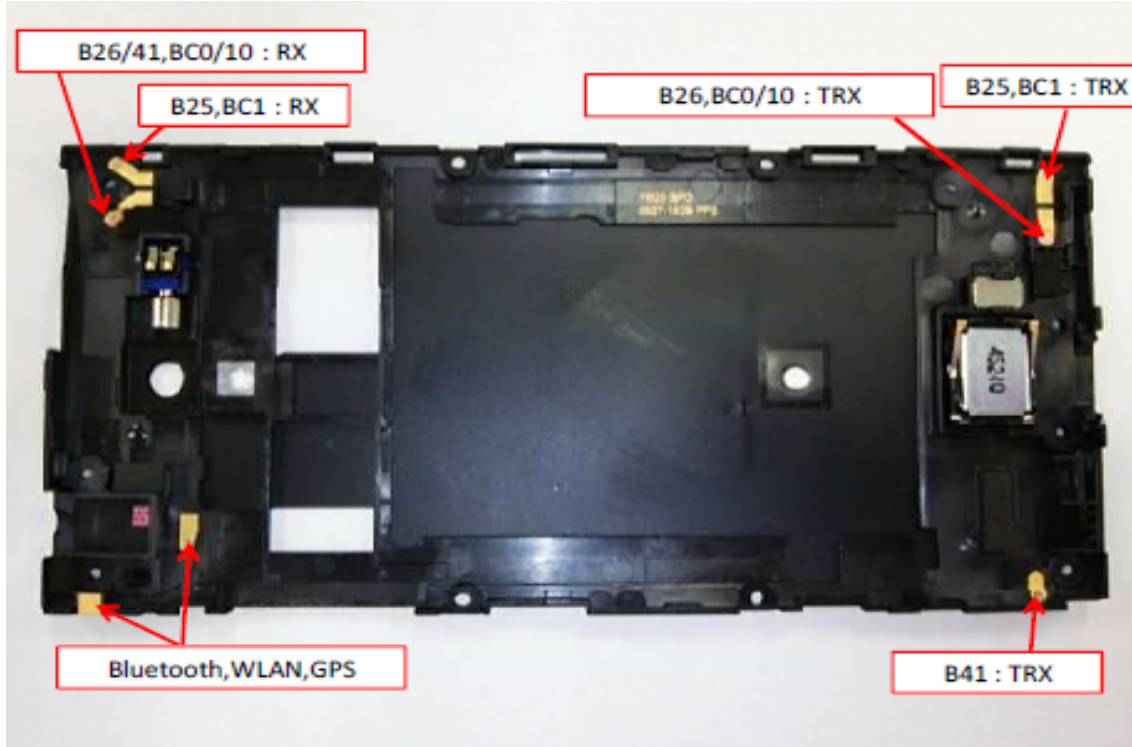
BT/WLAN/WWAN/GPS Antenna
