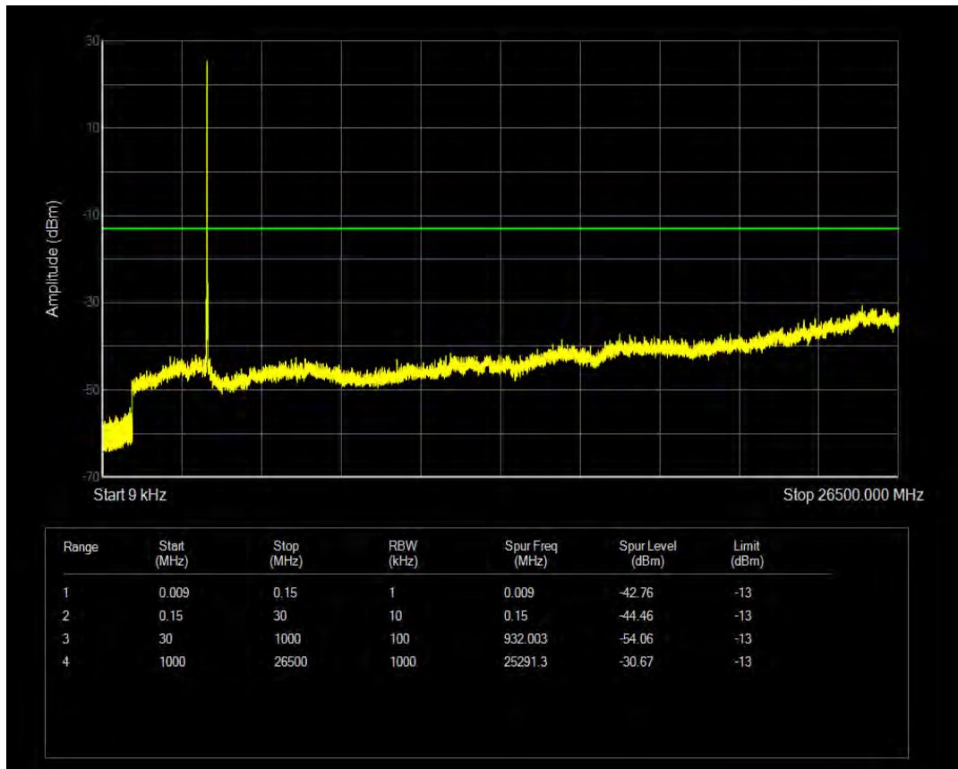
Band42 QPSK BW=15MHz Channel=42590 RB Size=75 Position=#0
