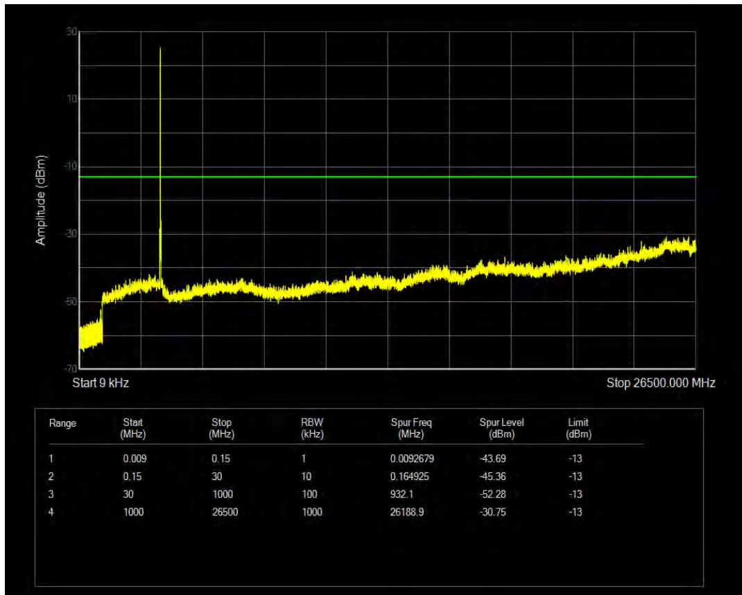
Band42 16QAM BW=15MHz Channel=42590 RB Size=75 Position=#0
