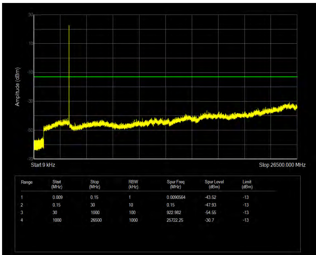
Band42 QPSK BW=10MHz Channel=42140 RB Size=1 Position=#0
