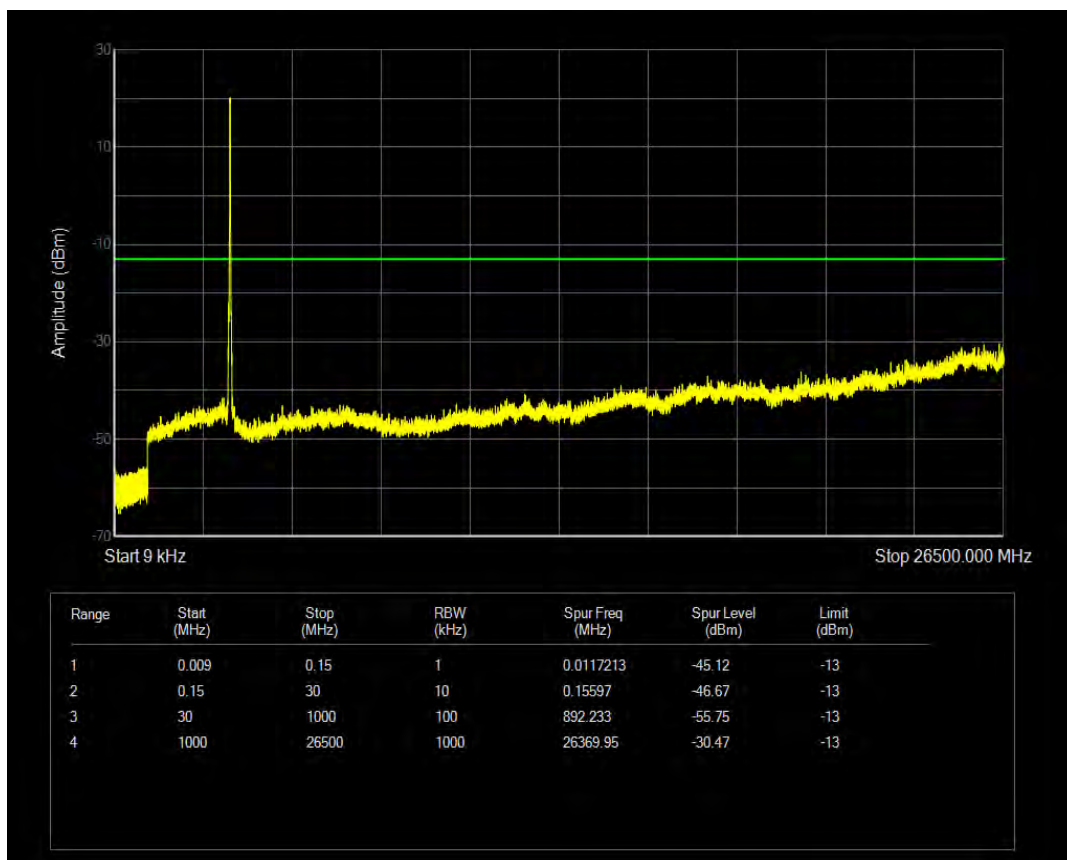
Band42 16QAM BW=20MHz Channel=42190 RB Size=1 Position=#0
