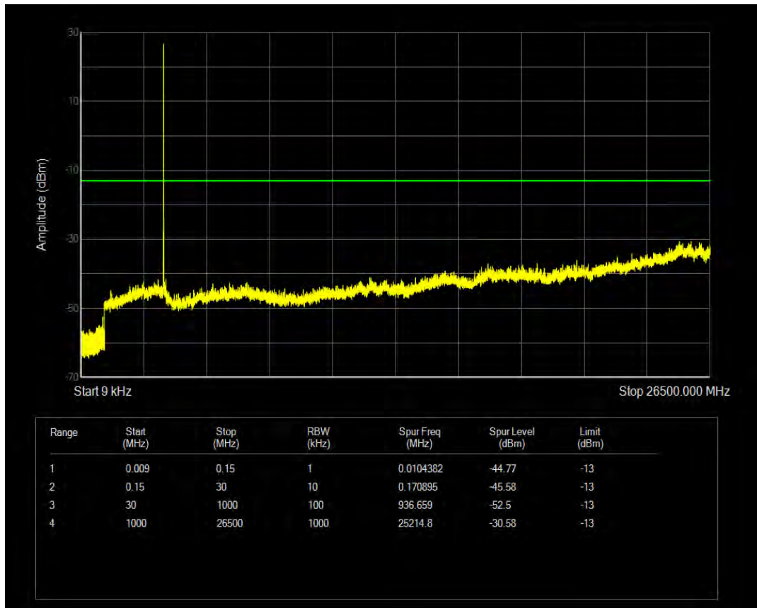
Band42 16QAM BW=5MHz Channel=42590 RB Size=25 Position=#0
