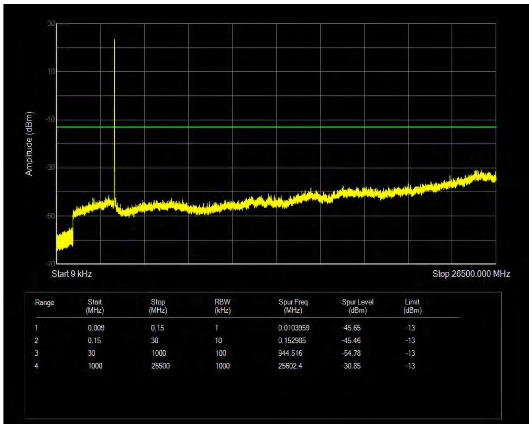
Band42 16QAM BW=5MHz Channel=42590 RB Size=1 Position=#0
