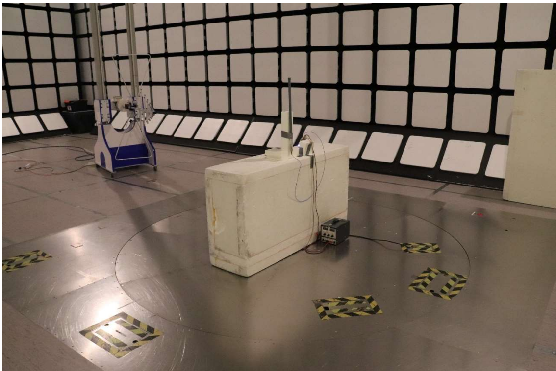
Photograph 3. Radiated Emissions 30 – 1000 MHz (whip antenna)
