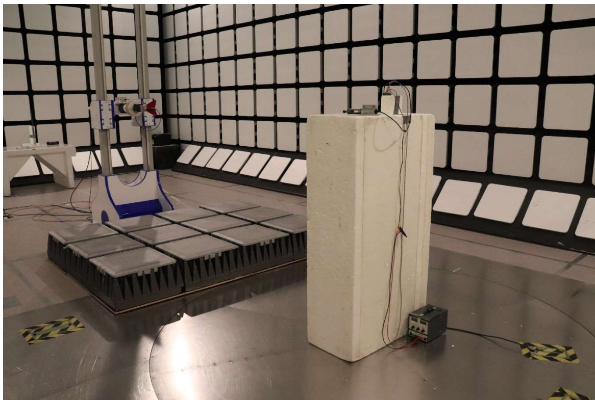
Photograph 7. Radiated Emissions 1 – 10 GHz (Yagi antenna)
