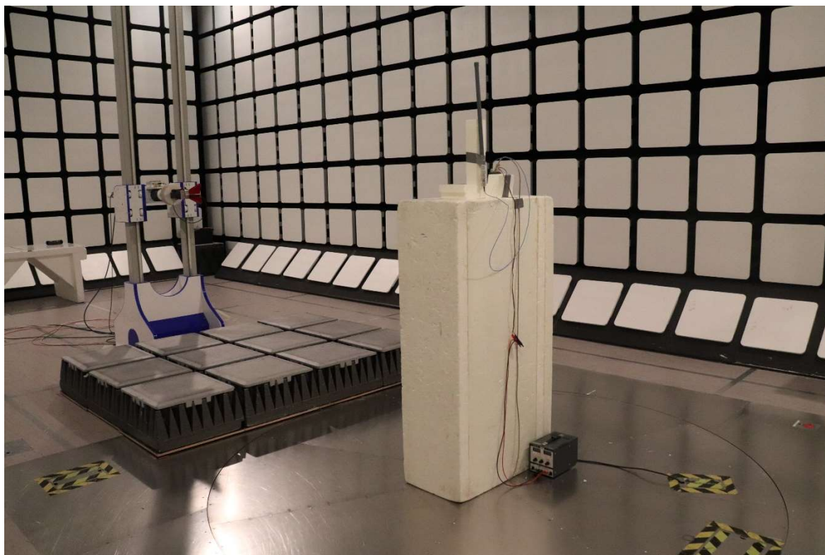
Photograph 4. Radiated Emissions 1 – 10 GHz (whip antenna)
