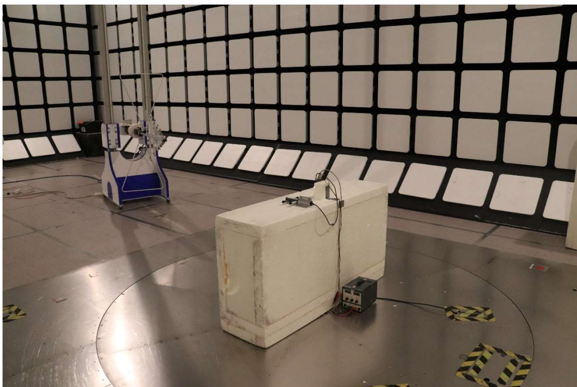
Photograph 6. Radiated Emissions 30 – 1000 MHz (Yagi antenna)
