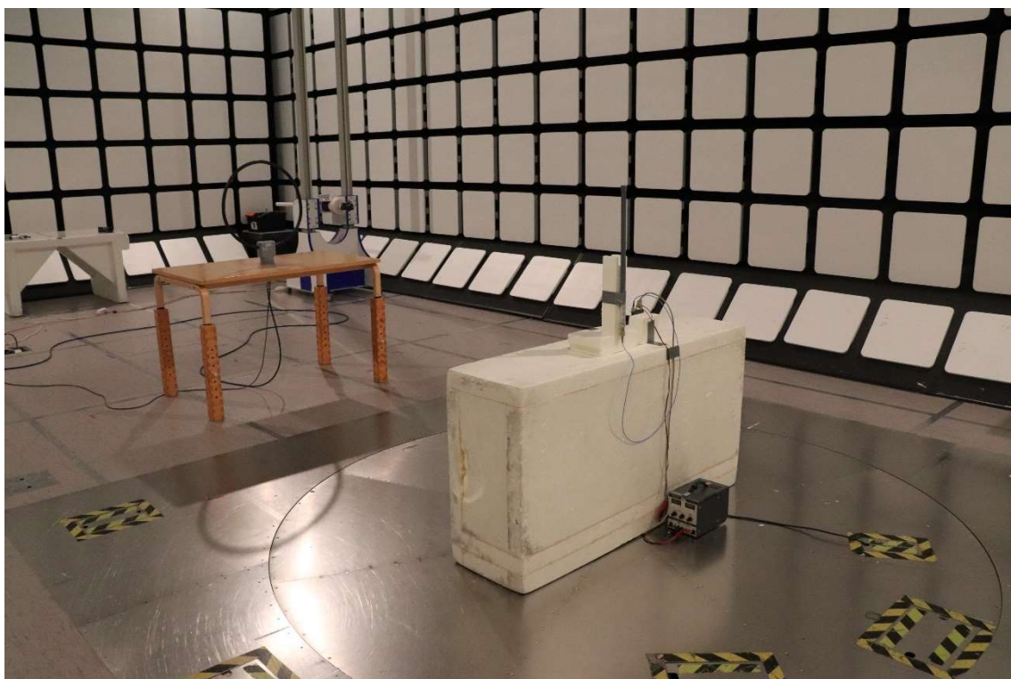
Photograph 2. Radiated Emissions 9 kHz – 30 MHz (whip antenna)
