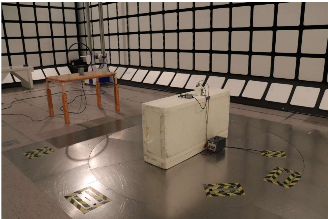
Photograph 5. Radiated Emissions 9 kHz – 30 MHz (Yagi antenna)
