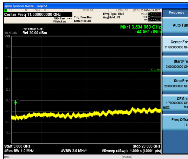
Band4_3MHz_16QAM_20385_1RB#0_3000~20000_3000~20000
