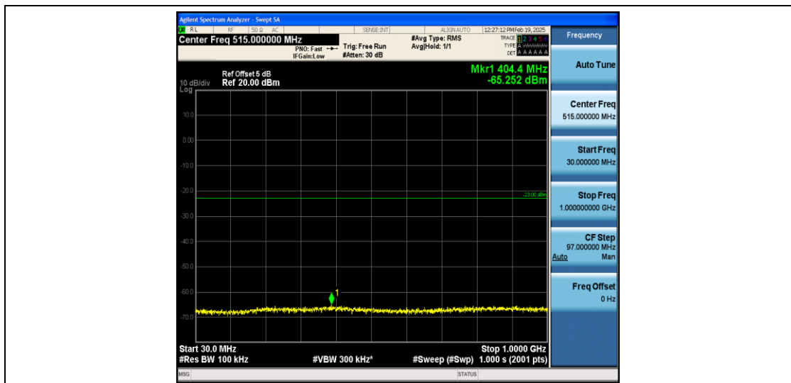
Band4_3MHz_16QAM_19965_1RB#0_30~1000_30~1000
