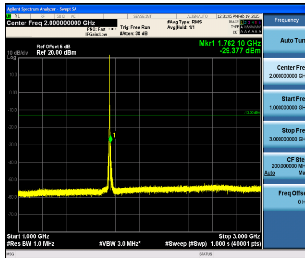
Band4_3MHz_16QAM_20385_1RB#0_1000~3000_1000~3000
