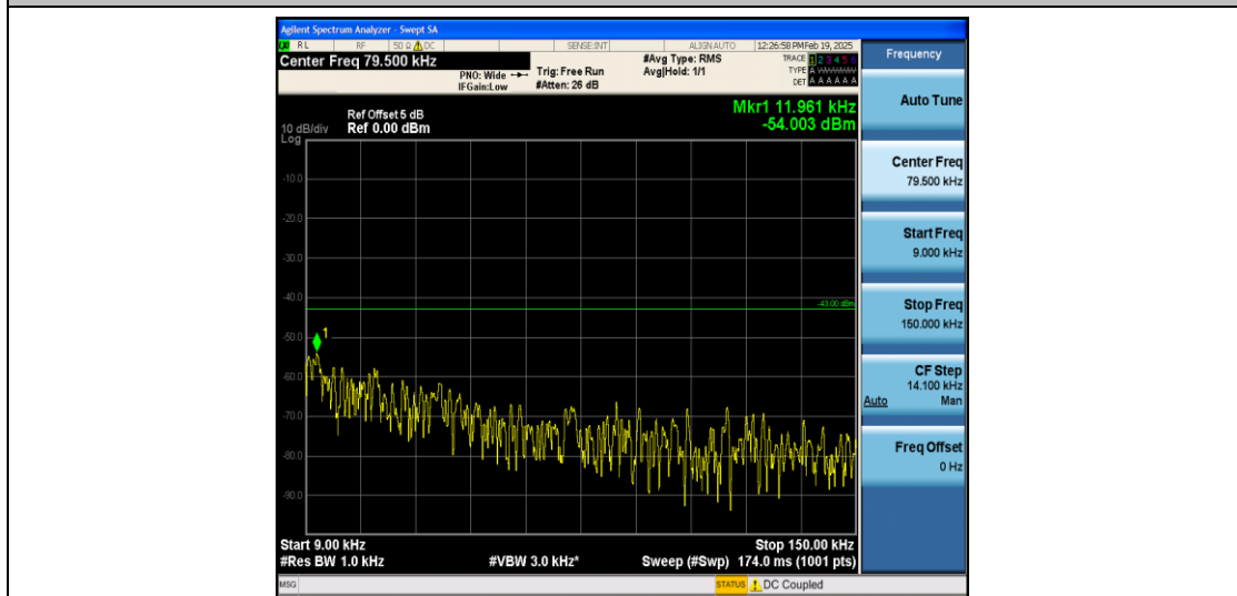
Band4_3MHz_16QAM_19965_1RB#0_0.009~0.15_0.009~0.15
