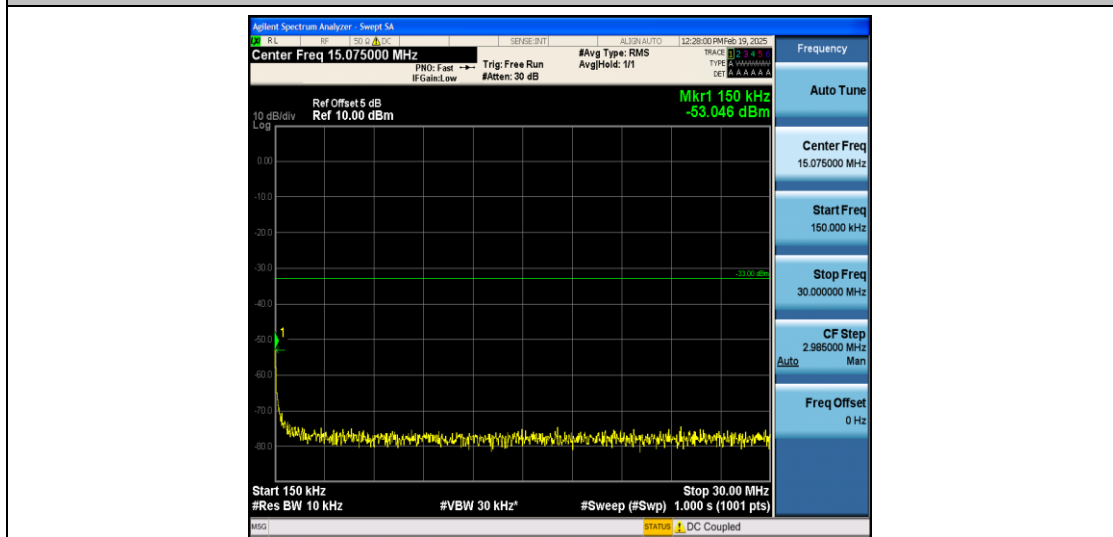
Band4_3MHz_QPSK_20175_1RB#0_0.15~30_0.15~30
