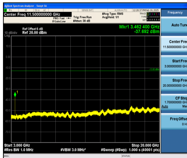
Band4_3MHz_QPSK_20175_1RB#0_3000~20000_3000~20000
