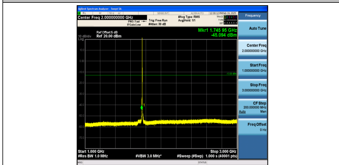
Band4_3MHz_QPSK_20385_1RB#0_1000~3000_1000~3000
