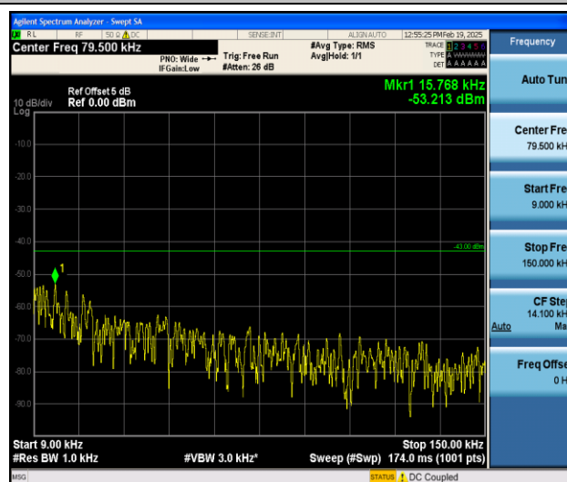
Band4_5MHz_QPSK_19975_1RB#0_0.009~0.15_0.009~0.15
