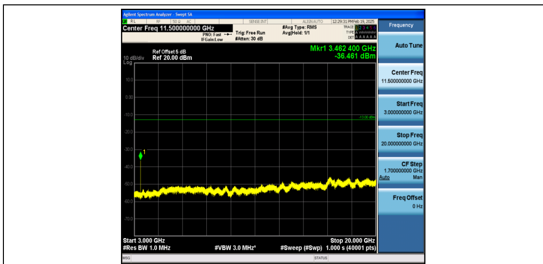
Band4_3MHz_16QAM_20175_1RB#0_3000~20000_3000~20000
