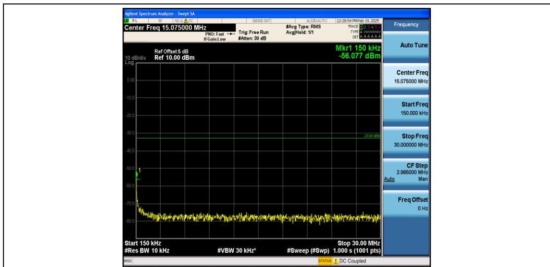
Band4_3MHz_16QAM_20175_1RB#0_0.15~30_0.15~30
