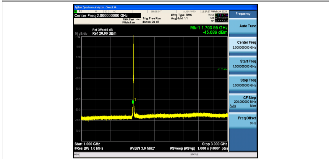
Band4_3MHz_16QAM_19965_1RB#0_1000~3000_1000~3000
