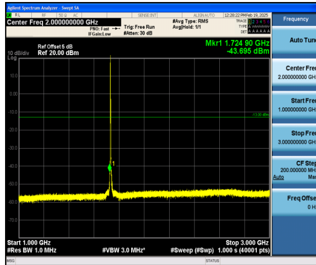
Band4_3MHz_QPSK_20175_1RB#0_1000~3000_1000~3000
