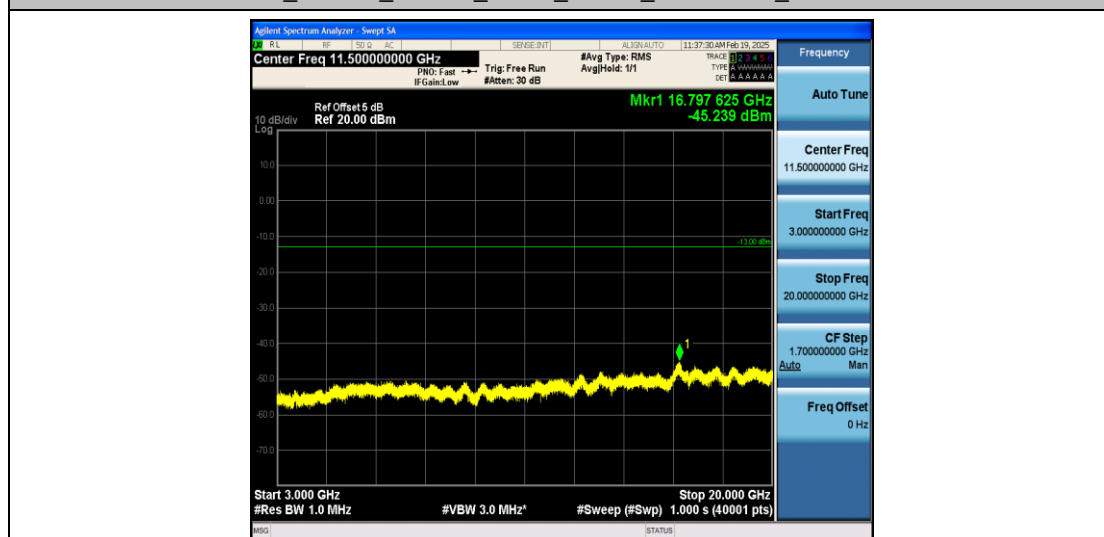
Band4_1.4MHz_16QAM_20393_1RB#0_3000~20000_3000~20000
