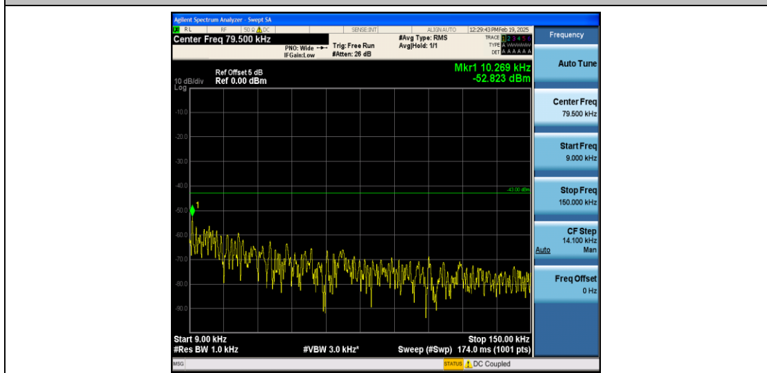
Band4_3MHz_QPSK_20385_1RB#0_0.009~0.15_0.009~0.15
