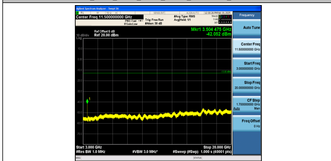
Band4_3MHz_QPSK_20385_1RB#0_3000~20000_3000~20000
