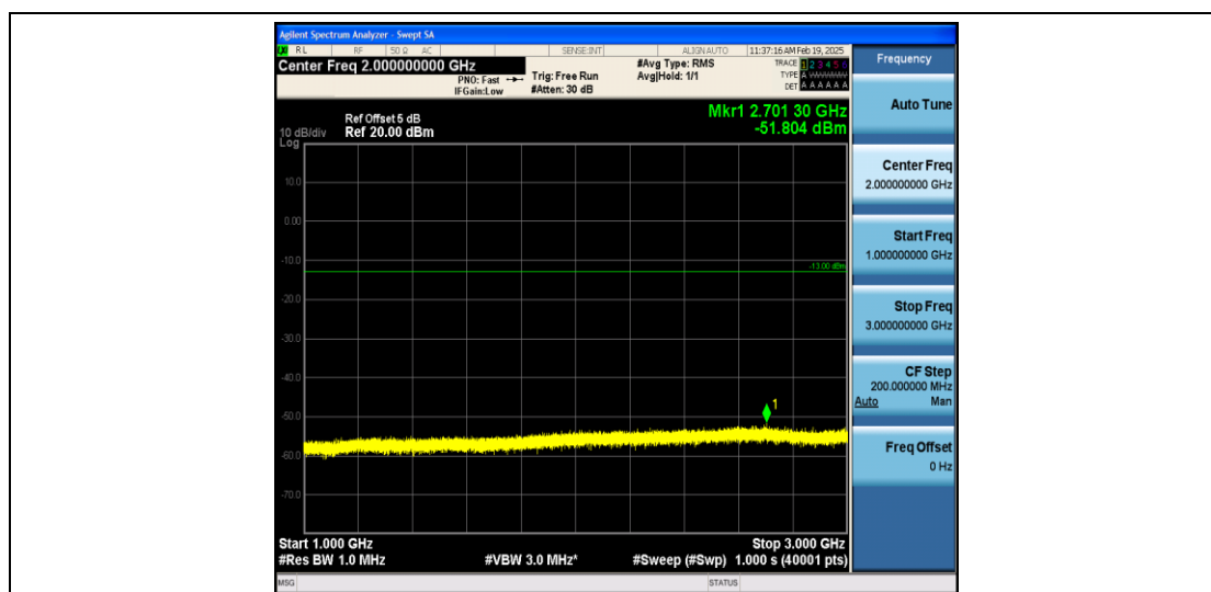
Band4_1.4MHz_16QAM_20393_1RB#0_1000~3000_1000~3000
