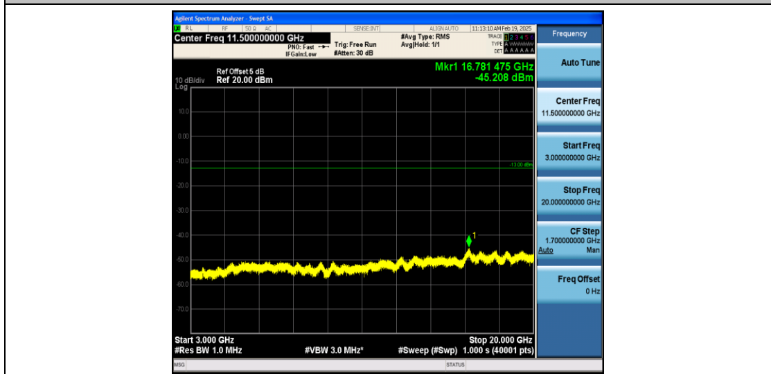
Band4_1.4MHz_QPSK_20175_1RB#0_3000~20000_3000~20000
