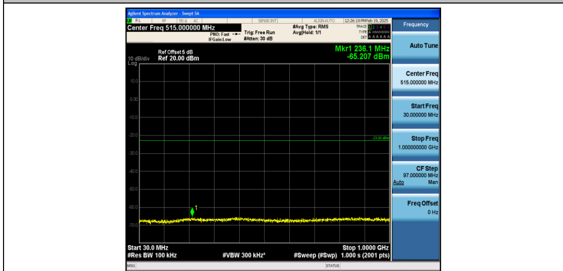
Band4_3MHz_QPSK_19965_1RB#0_30~1000_30~1000
