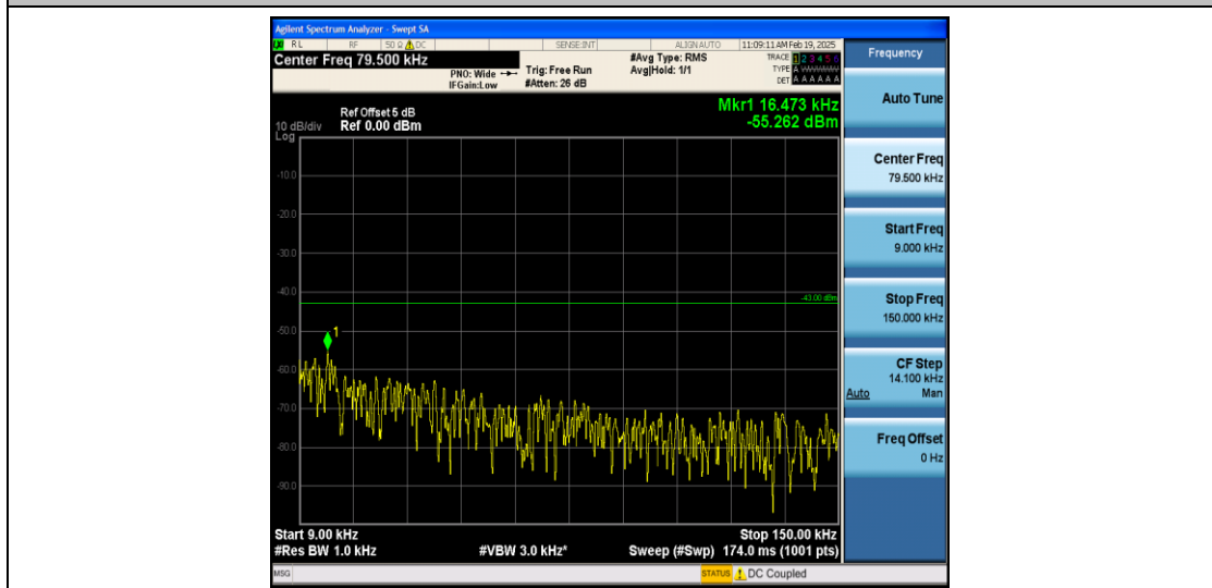
Band4_1.4MHz_16QAM_19957_1RB#0_0.009~0.15_0.009~0.15
