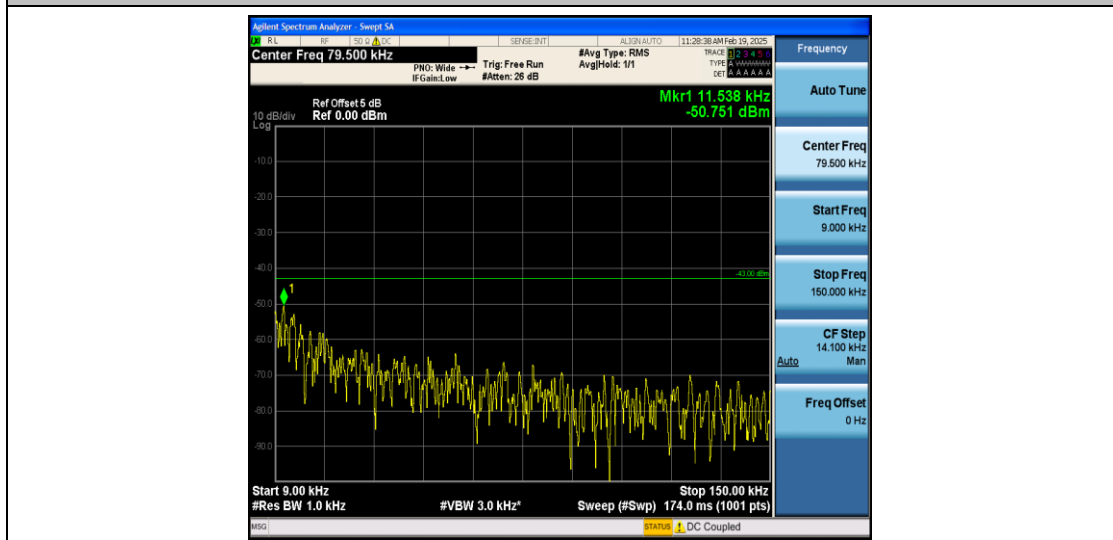
Band4_1.4MHz_QPSK_20393_1RB#0_0.009~0.15_0.009~0.15
