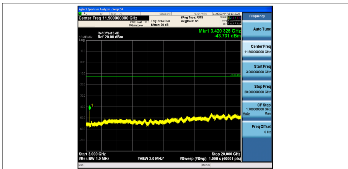
Band4_1.4MHz_QPSK_19957_1RB#0_3000~20000_3000~20000
