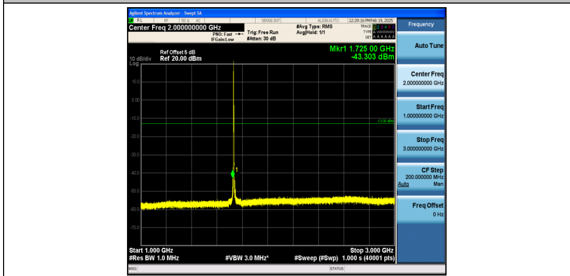
Band4_3MHz_16QAM_20175_1RB#0_1000~3000_1000~3000
