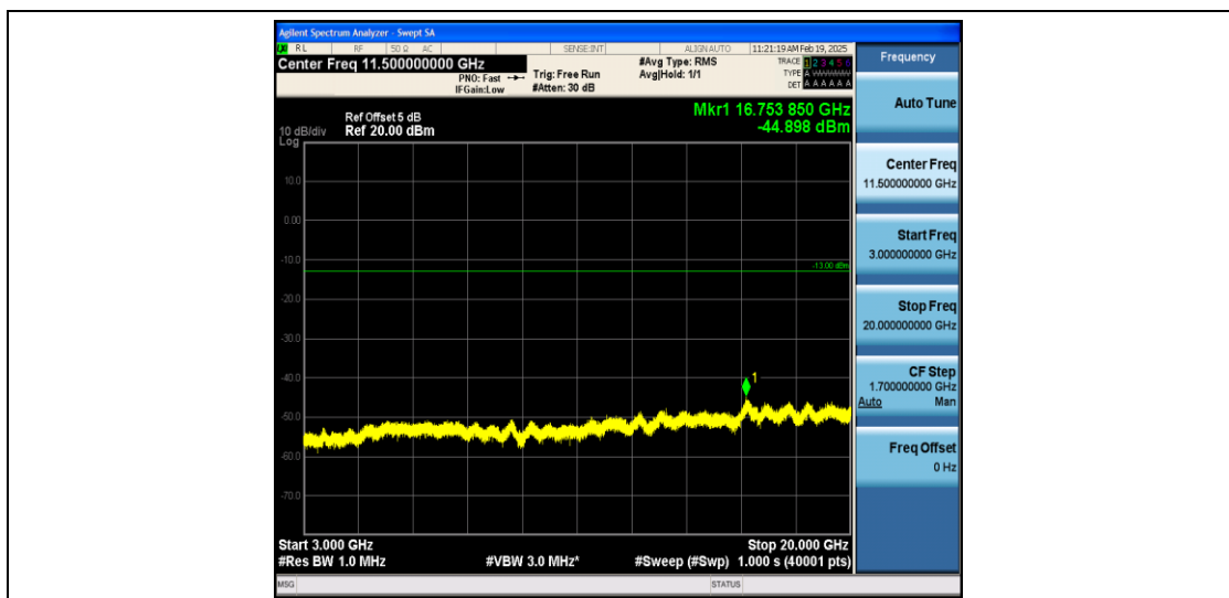
Band4_1.4MHz_16QAM_20175_1RB#0_3000~20000_3000~20000
