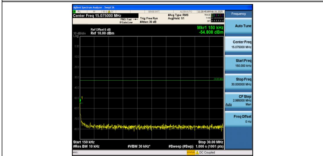
Band4_1.4MHz_QPSK_20393_1RB#0_0.15~30_0.15~30
