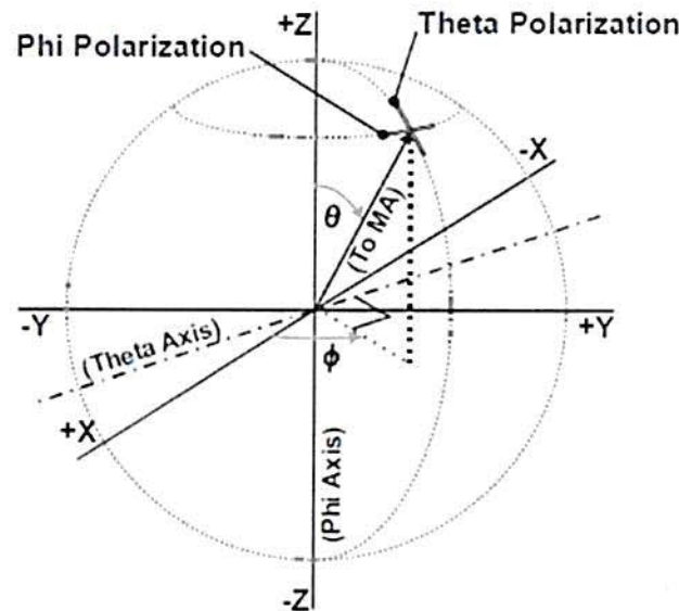
Figure 7-3: Theta/Phi coordinate system.
