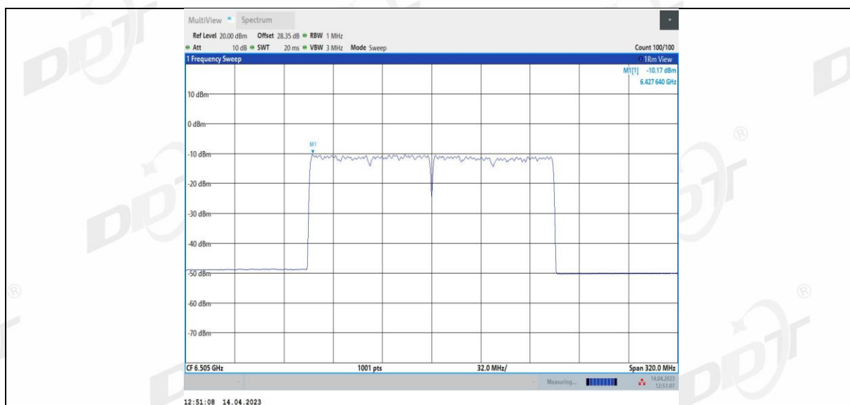
11AX160MIMO Ant3_6505
