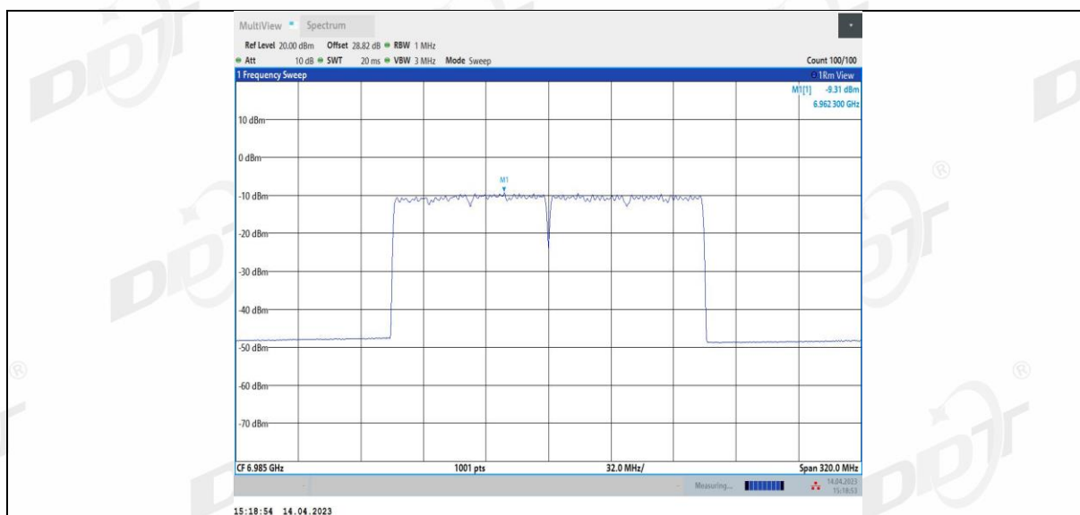
11AX160MIMO Ant3 6985
