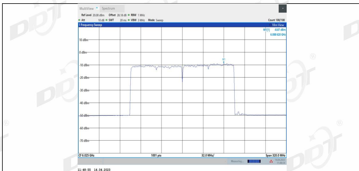
11AX160MIMO Ant3 6025
