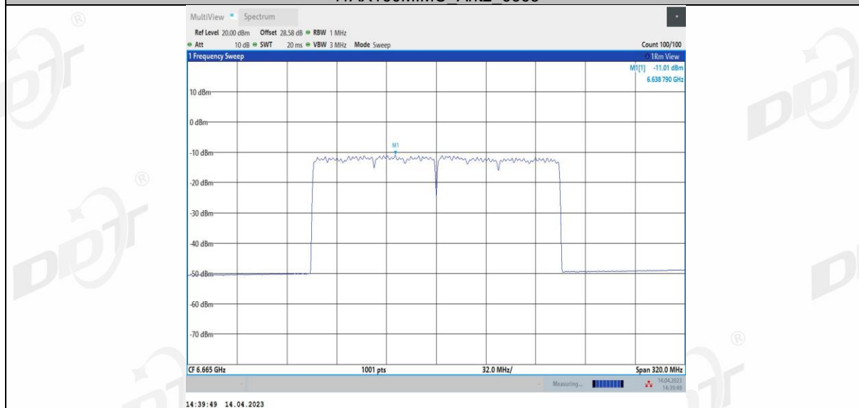
11AX160MIMO Ant3 6665
