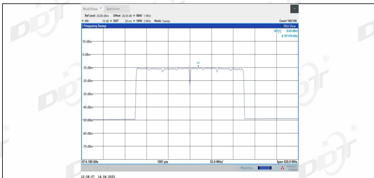
11AX160MIMO Ant2 6185
