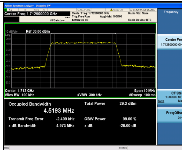
Band4-5MHz-QPSK-19975-25RB#0-PASS
