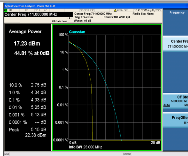
Band17-10MHz-QPSK-23800-1RB#0-PASS
