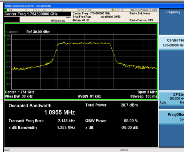
Band4-1.4MHz-QPSK-20393-6RB#0-PASS
