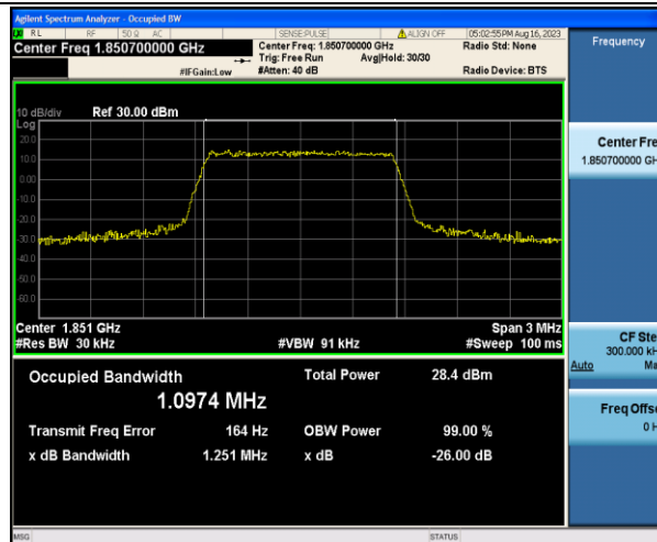
Band2-1.4MHz-QPSK-18607-6RB#0-PASS
