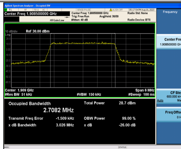
Band2-3MHz-QPSK-19185-15RB#0-PASS
