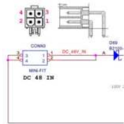
Figure 36: DC input
