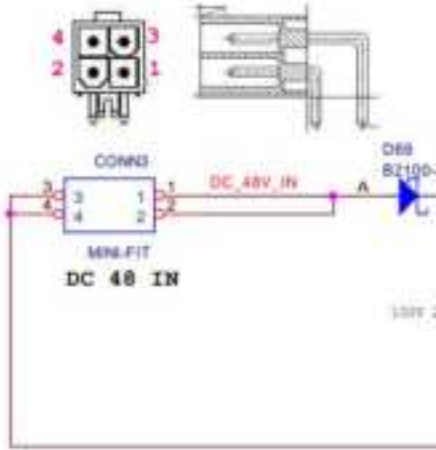
Figure 40: DC input
