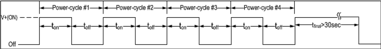
Figure 112: Power cycle timings
