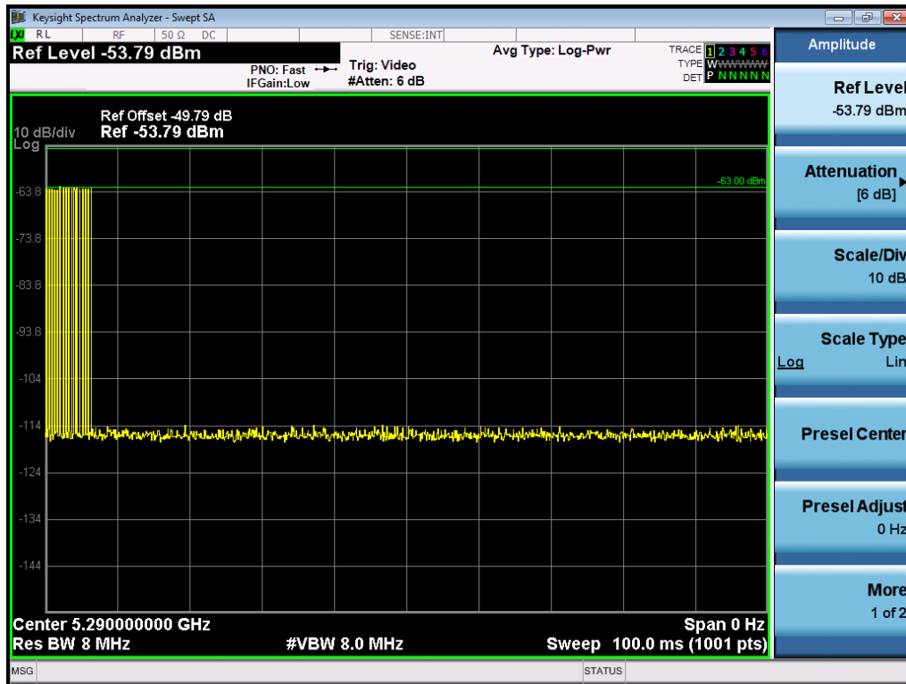
USA Bin 3 Radar Calibration BW160
