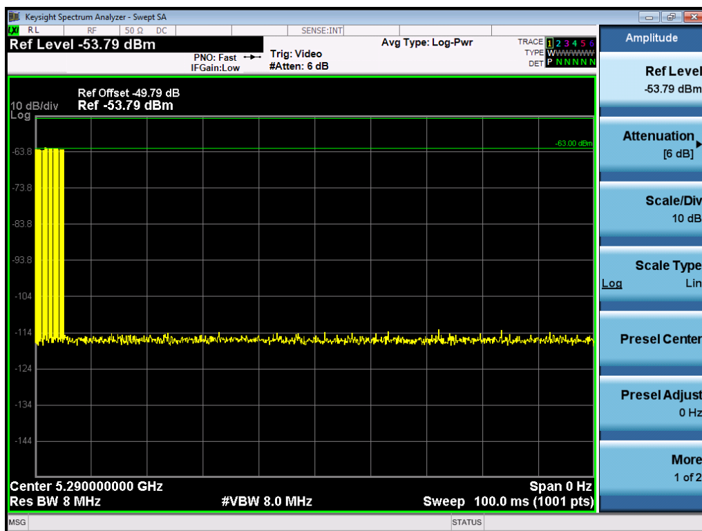
USA Bin 2 Radar Calibration BW160
