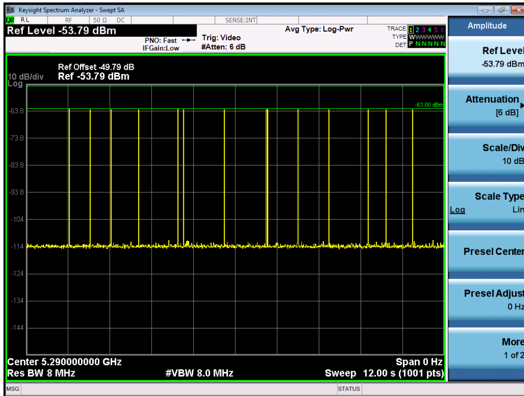
USA Bin 5 Radar Calibration BW160
