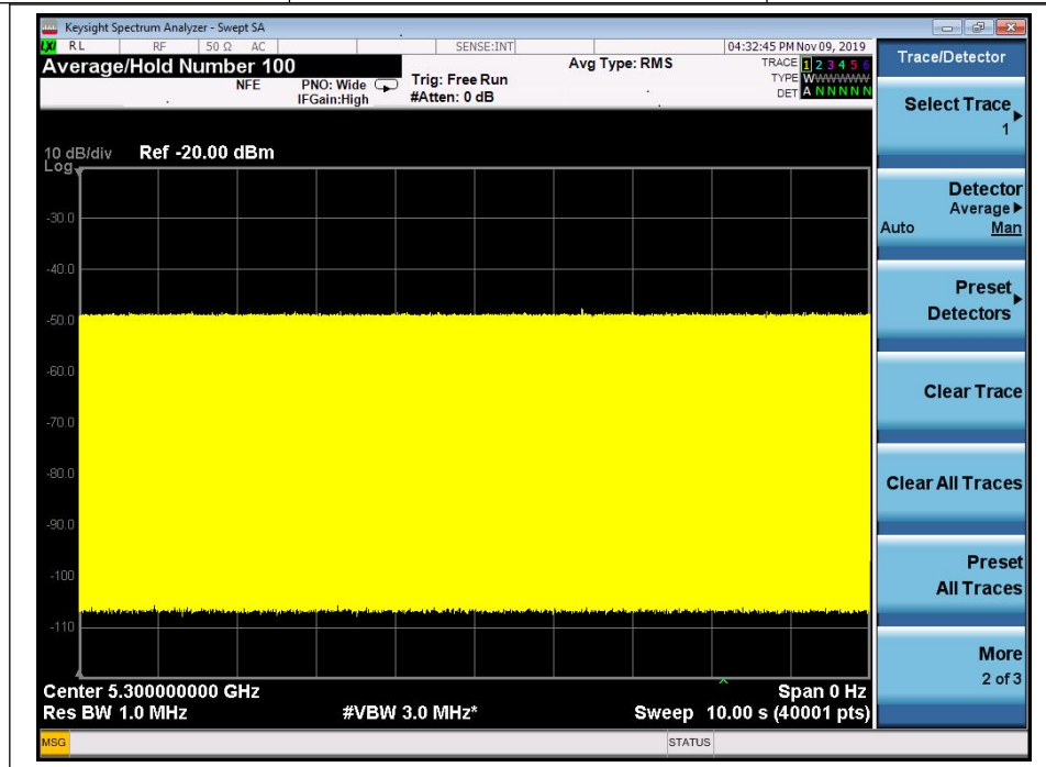
(Test sequence)
