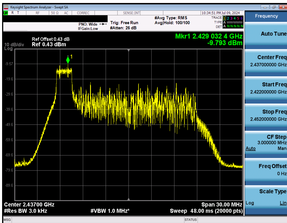
Plot 7-28. Power Spectral Density Plot Antenna WF8 (802.11ax OFDMA – RU26 Index 0 – Ch. 6)
