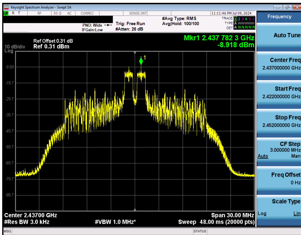
Plot 7-57. Power Spectral Density Plot Antenna WF8 (802.11ax OFDMA – RU26 Index 4 – Ch. 6)
