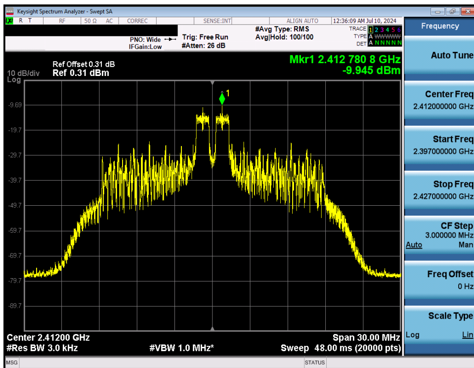
Plot 7-52. Power Spectral Density Plot Antenna WF7 (802.11ax OFDMA – RU26 Index 4 – Ch. 1)
