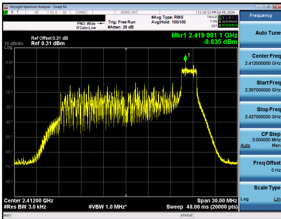
Plot 7-53. Power Spectral Density Plot Antenna WF8 (802.11ax OFDMA – RU26 Index 8 – Ch. 1)
