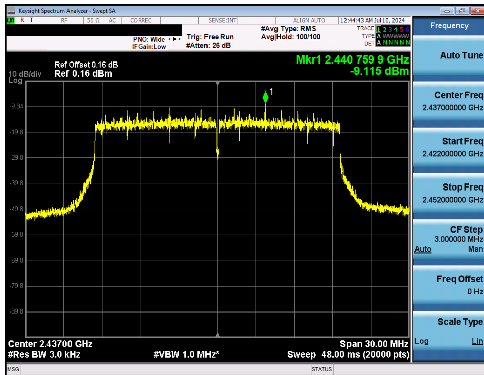
Plot 7-70. Power Spectral Density Plot Antenna WF7 (802.11ax OFDMA – RU242 – Ch. 6)
