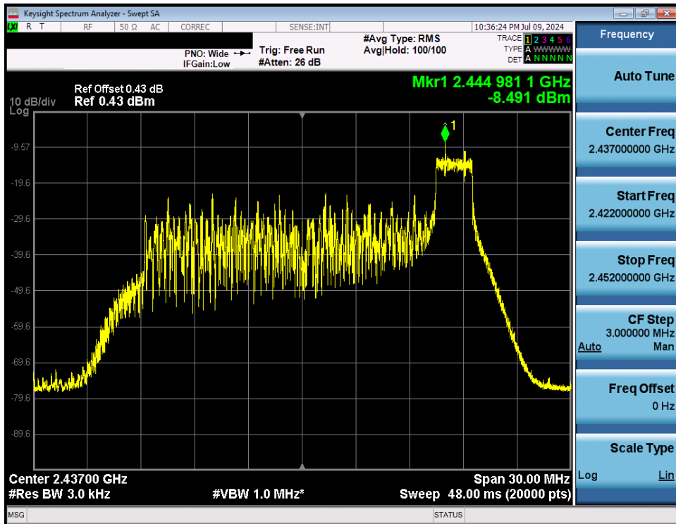
Plot 7-30. Power Spectral Density Plot Antenna WF8 (802.11ax OFDMA – RU26 Index 8 – Ch. 6)
