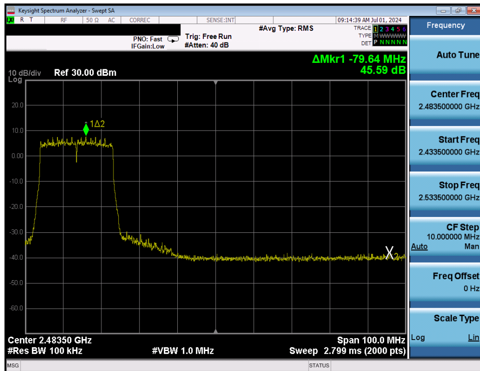
Plot 7-84. Band Edge Antenna WF8 (802.11ax OFDMA – RU242 – Ch. 8)
