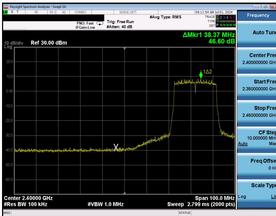
Plot 7-80. Band Edge Antenna WF8 (802.11ax OFDMA – RU242 – Ch. 5)
