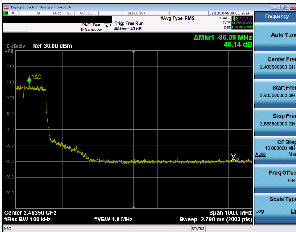
Plot 7-82. Band Edge Antenna WF8 (802.11ax OFDMA – RU242 – Ch. 6 High)
