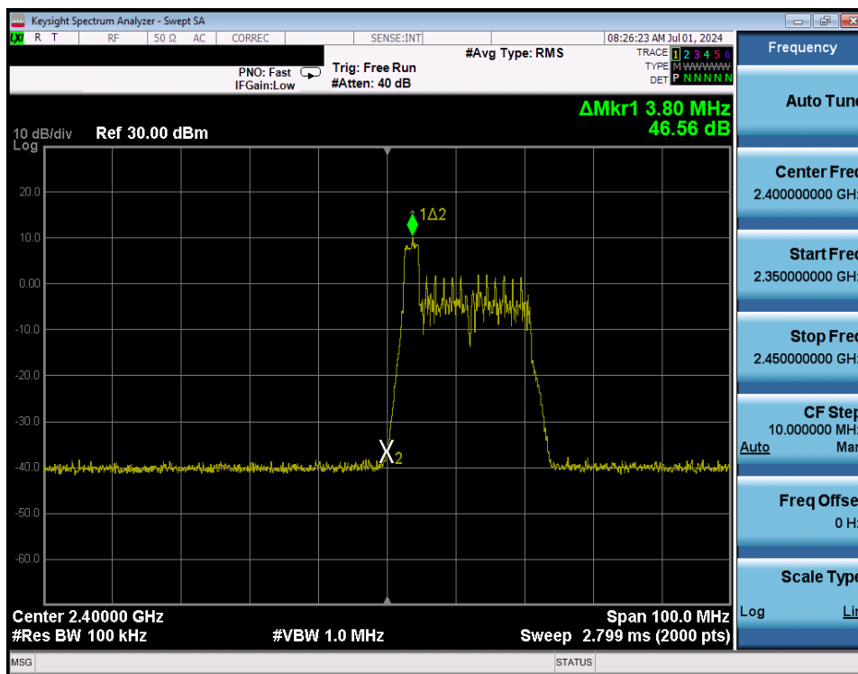
Plot 7-73. Band Edge Antenna WF8 (802.11ax OFDMA – RU26 Index 0 – Ch. 1)
