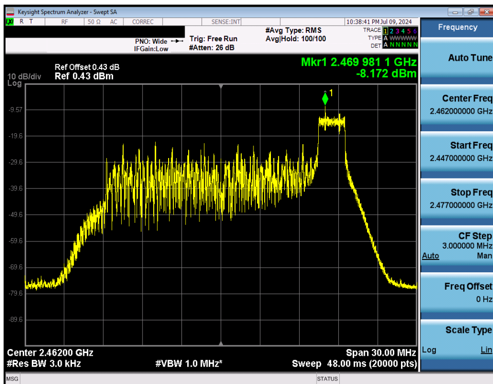
Plot 7-33. Power Spectral Density Plot Antenna WF8 (802.11ax OFDMA – RU26 Index 8 – Ch. 11)
