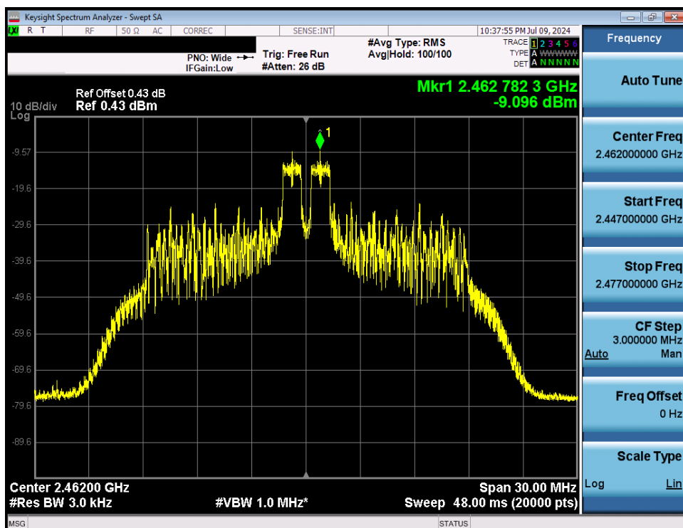
Plot 7-32. Power Spectral Density Plot Antenna WF8 (802.11ax OFDMA – RU26 Index 4 – Ch. 11)
