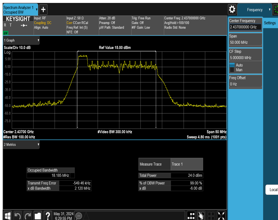
Plot 7-4. 6dB BW & 99% OBW Plot Antenna WF8 (802.11ax OFDMA – RU26 Index 0 – Ch. 6)
