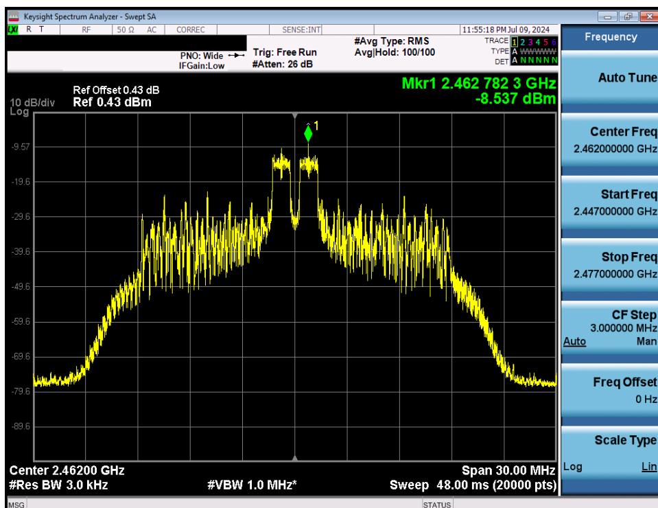
Plot 7-44. Power Spectral Density Plot Antenna WF7 (802.11ax OFDMA – RU26 Index 4 – Ch. 11)
