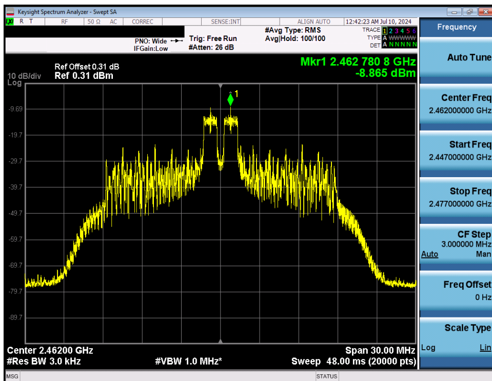
Plot 7-64. Power Spectral Density Plot Antenna WF7 (802.11ax OFDMA – RU26 Index 4 – Ch. 11)
