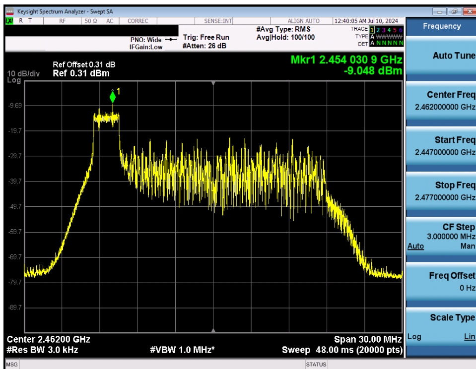
Plot 7-62. Power Spectral Density Plot Antenna WF7 (802.11ax OFDMA – RU26 Index 0 – Ch. 11)
