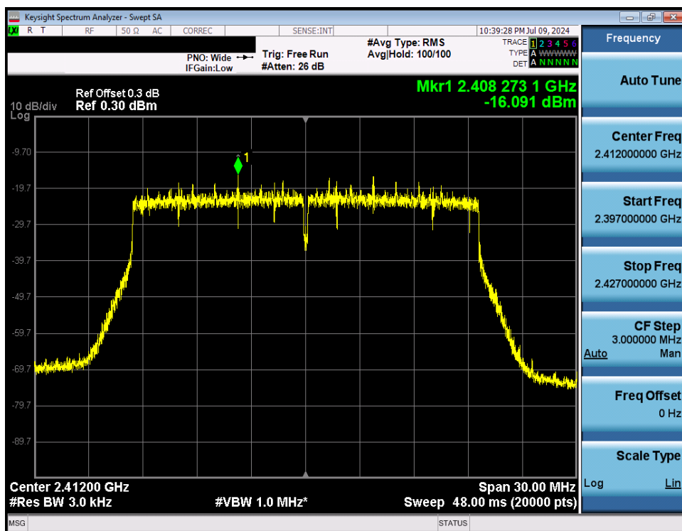
Plot 7-34. Power Spectral Density Plot Antenna WF8 (802.11ax OFDMA – RU242 – Ch. 1)
