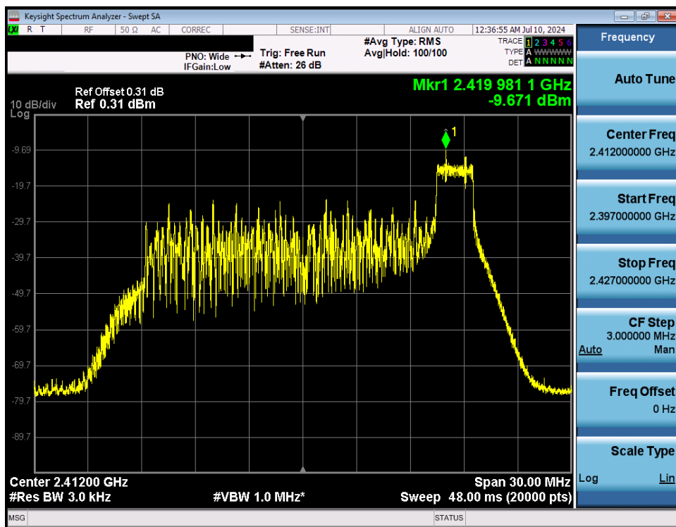
Plot 7-54. Power Spectral Density Plot Antenna WF7 (802.11ax OFDMA – RU26 Index 8 – Ch. 1)
