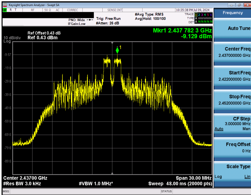
Plot 7-29. Power Spectral Density Plot Antenna WF8 (802.11ax OFDMA – RU26 Index 4 – Ch. 6)
