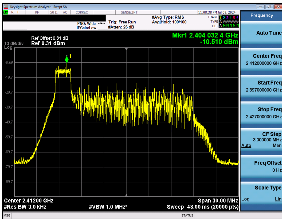
Plot 7-49. Power Spectral Density Plot Antenna WF8 (802.11ax OFDMA – RU26 Index 0 – Ch. 1)
