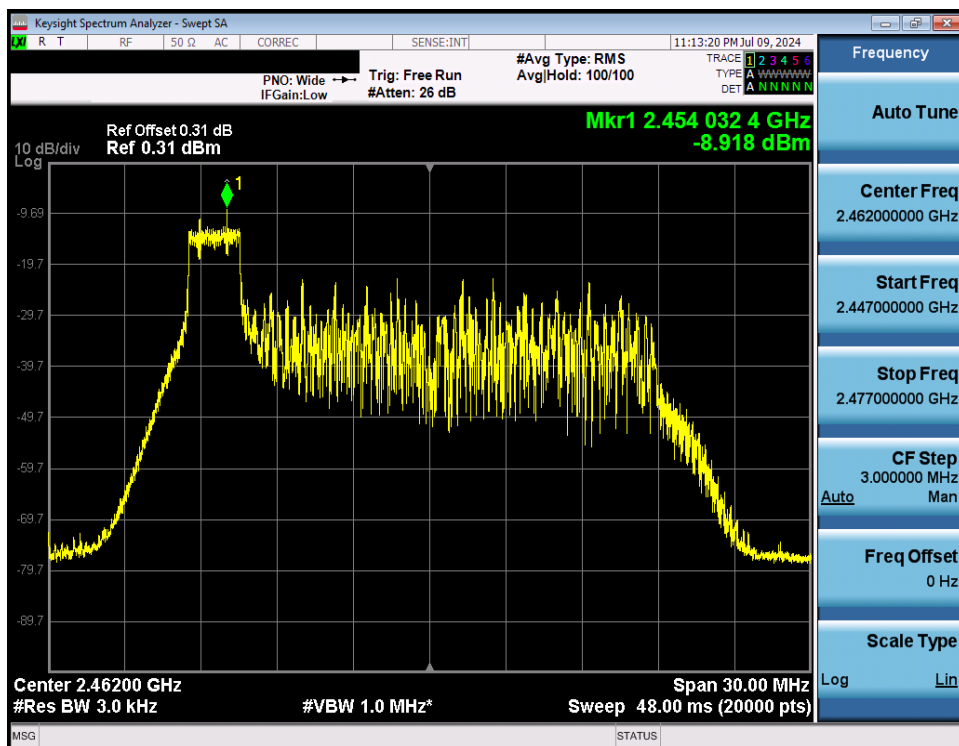
Plot 7-61. Power Spectral Density Plot Antenna WF8 (802.11ax OFDMA – RU26 Index 0 – Ch. 11)
