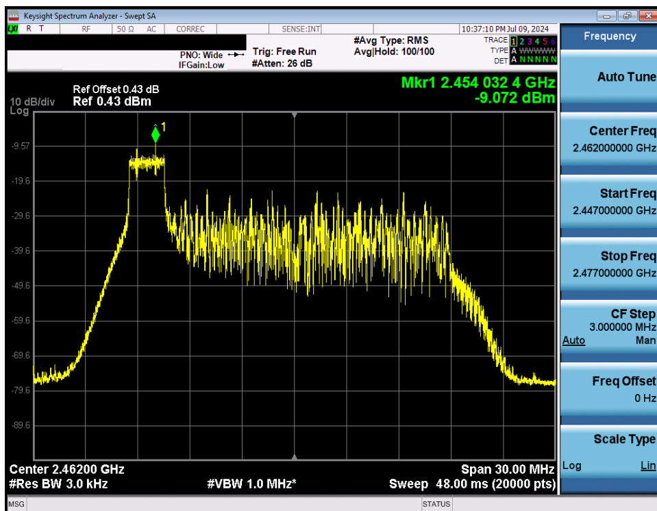
Plot 7-31. Power Spectral Density Plot Antenna WF8 (802.11ax OFDMA – RU26 Index 0 – Ch. 11)
