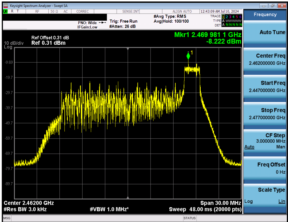
Plot 7-66. Power Spectral Density Plot Antenna WF7 (802.11ax OFDMA – RU26 Index 8 – Ch. 11)
