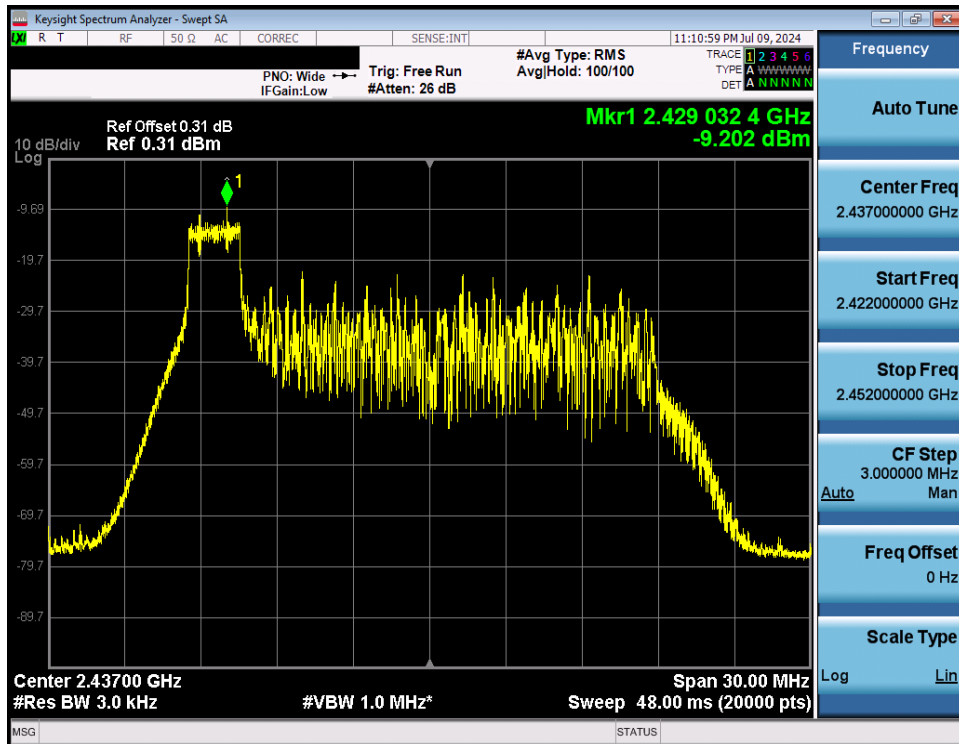
Plot 7-55. Power Spectral Density Plot Antenna WF8 (802.11ax OFDMA – RU26 Index 0 – Ch. 6)
