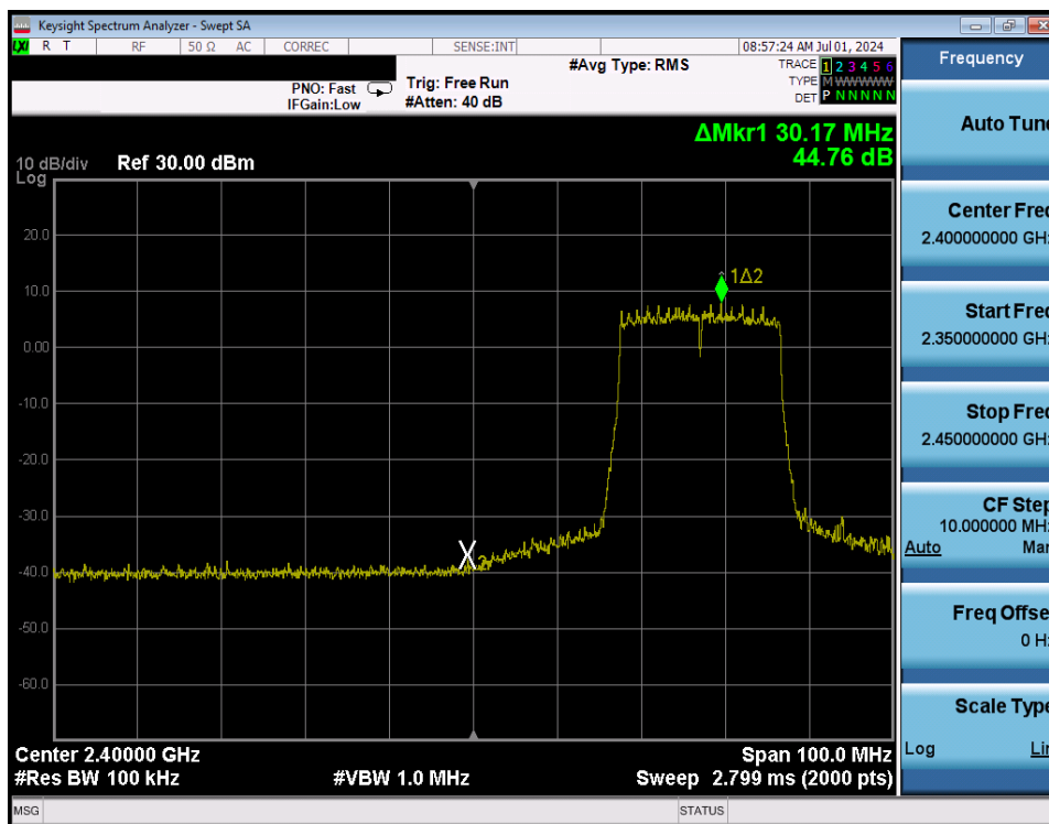
Plot 7-79. Band Edge Antenna WF8 (802.11ax OFDMA – RU242 – Ch. 4)
