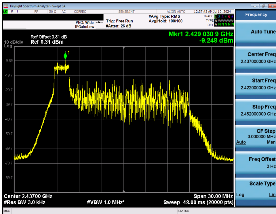
Plot 7-56. Power Spectral Density Plot Antenna WF7 (802.11ax OFDMA – RU26 Index 0 – Ch. 6)
