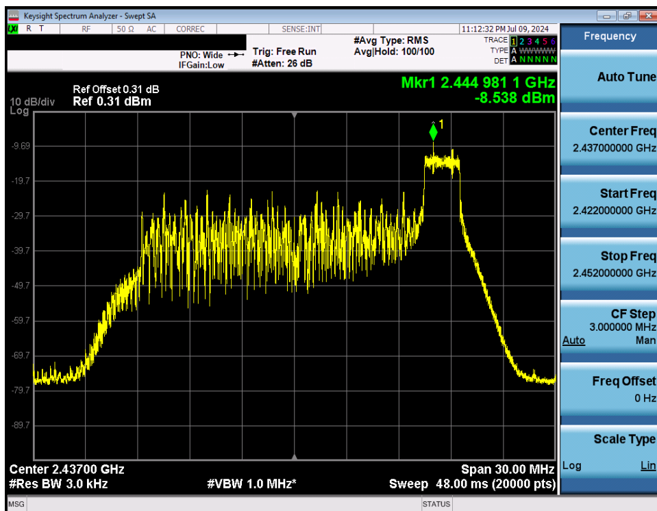
Plot 7-59. Power Spectral Density Plot Antenna WF8 (802.11ax OFDMA – RU26 Index 8 – Ch. 6)
