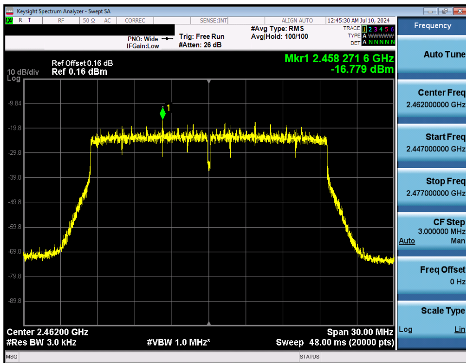
Plot 7-72. Power Spectral Density Plot Antenna WF7 (802.11ax OFDMA – RU242 – Ch. 11)
