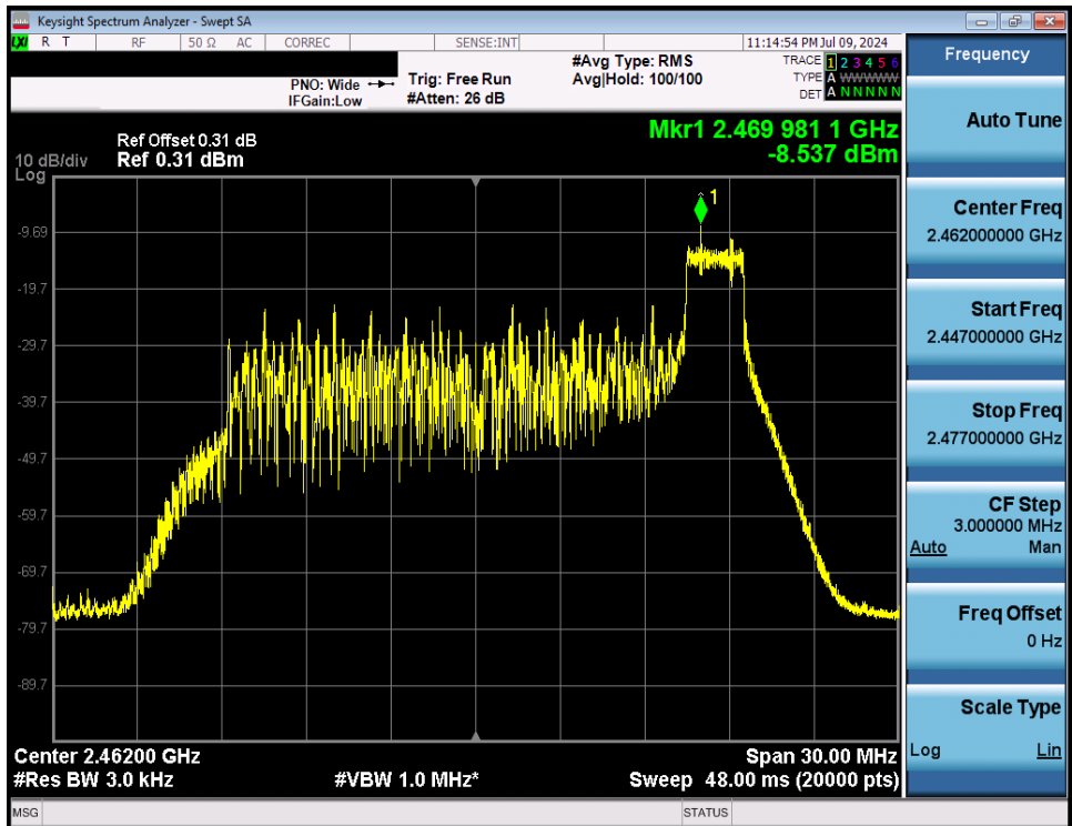
Plot 7-65. Power Spectral Density Plot Antenna WF8 (802.11ax OFDMA – RU26 Index 8 – Ch. 11)
