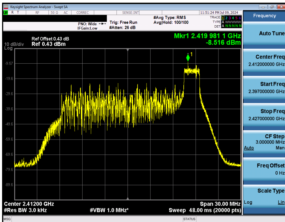
Plot 7-39. Power Spectral Density Plot Antenna WF7 (802.11ax OFDMA – RU26 Index 8 – Ch. 1)
