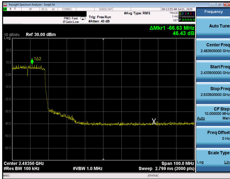
Plot 7-83. Band Edge Antenna WF8 (802.11ax OFDMA – RU242 – Ch. 7)
