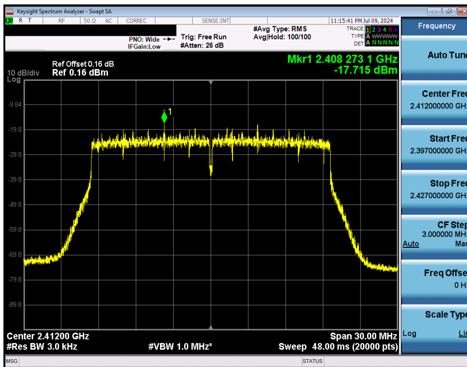
Plot 7-67. Power Spectral Density Plot Antenna WF8 (802.11ax OFDMA – RU242 – Ch. 1)
