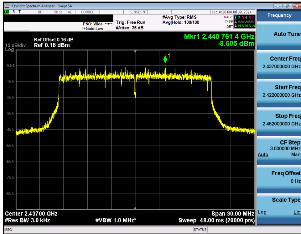
Plot 7-69. Power Spectral Density Plot Antenna WF8 (802.11ax OFDMA – RU242 – Ch. 6)
