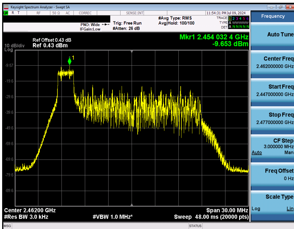
Plot 7-43. Power Spectral Density Plot Antenna WF7 (802.11ax OFDMA – RU26 Index 0 – Ch. 11)
