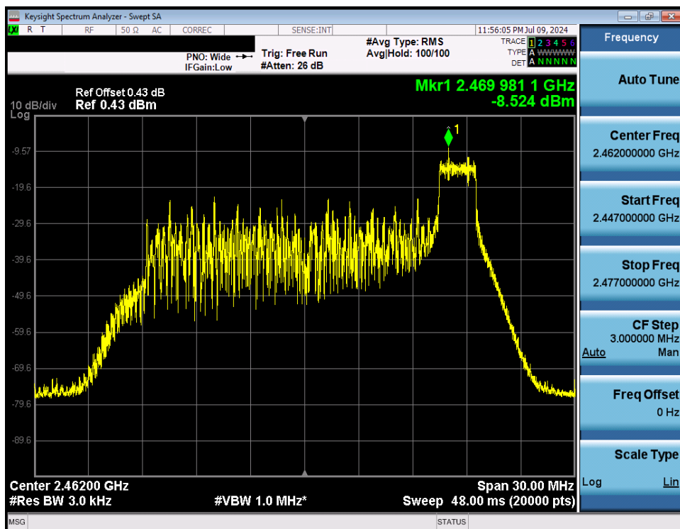
Plot 7-45. Power Spectral Density Plot Antenna WF7 (802.11ax OFDMA – RU26 Index 8 – Ch. 11)
