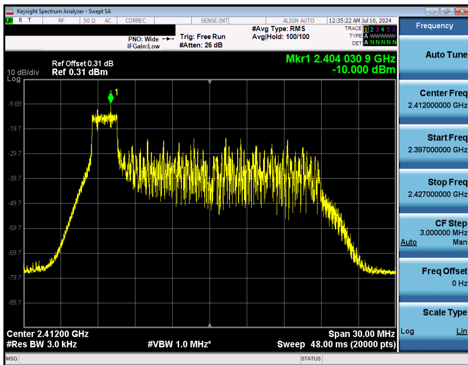
Plot 7-50. Power Spectral Density Plot Antenna WF7 (802.11ax OFDMA – RU26 Index 0 – Ch. 1)
