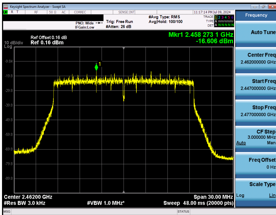
Plot 7-71. Power Spectral Density Plot Antenna WF8 (802.11ax OFDMA – RU242 – Ch. 11)
