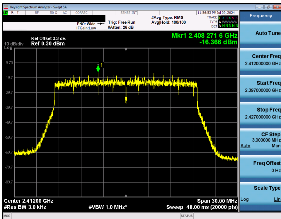
Plot 7-46. Power Spectral Density Plot Antenna WF7 (802.11ax OFDMA – RU242 – Ch. 1)
