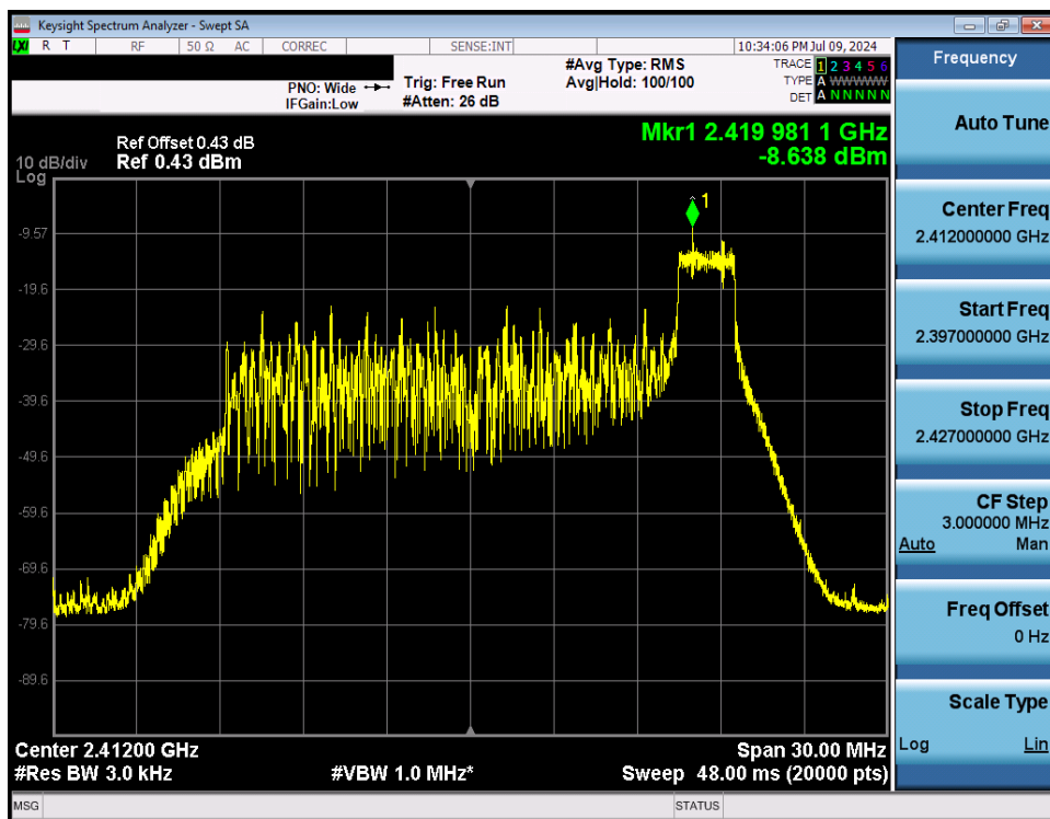
Plot 7-27. Power Spectral Density Plot Antenna WF8 (802.11ax OFDMA – RU26 Index 8 – Ch. 1)
