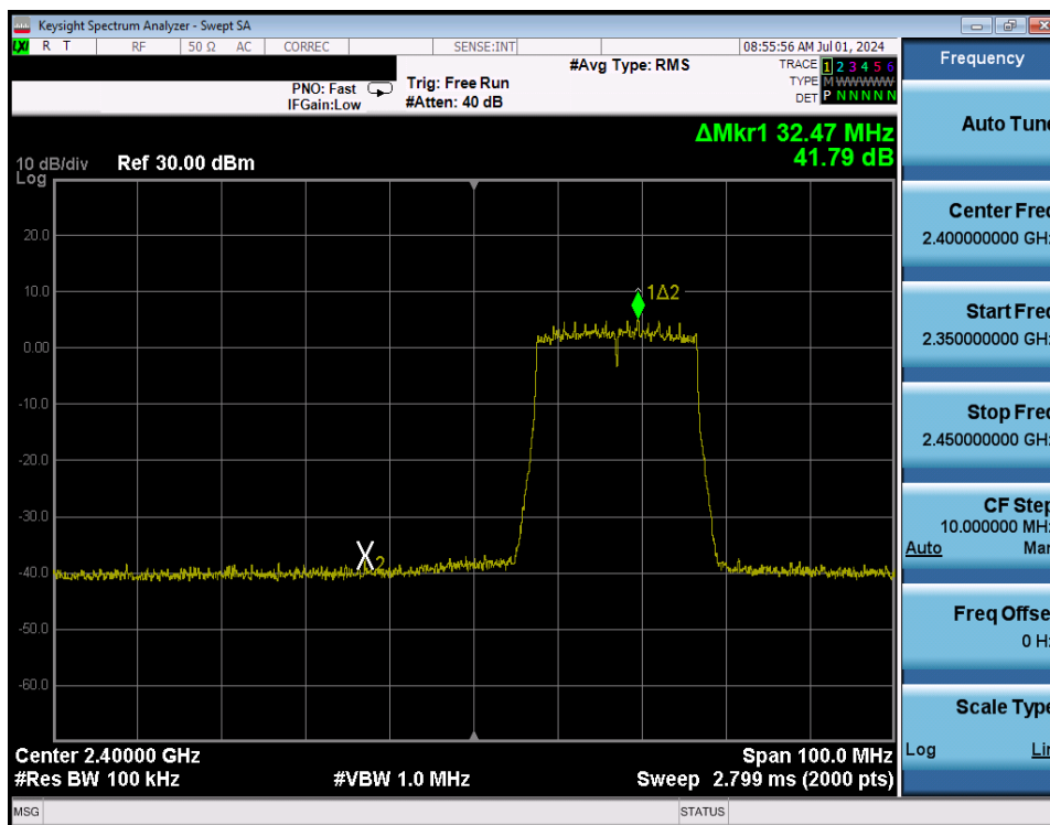
Plot 7-77. Band Edge Antenna WF8 (802.11ax OFDMA – RU242 – Ch. 2)
