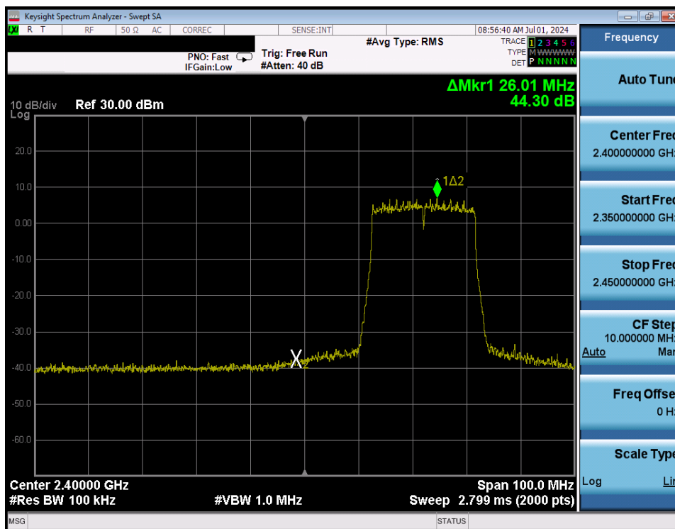
Plot 7-78. Band Edge Antenna WF8 (802.11ax OFDMA – RU242 – Ch. 3)
