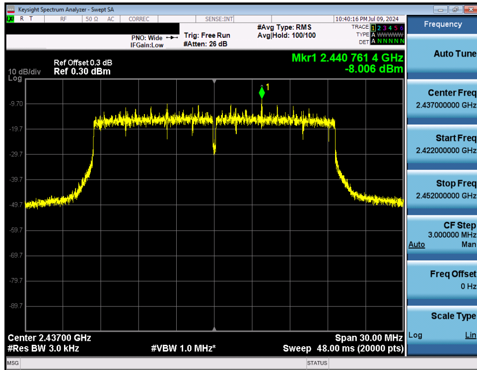
Plot 7-35. Power Spectral Density Plot Antenna WF8 (802.11ax OFDMA – RU242 – Ch. 6)
