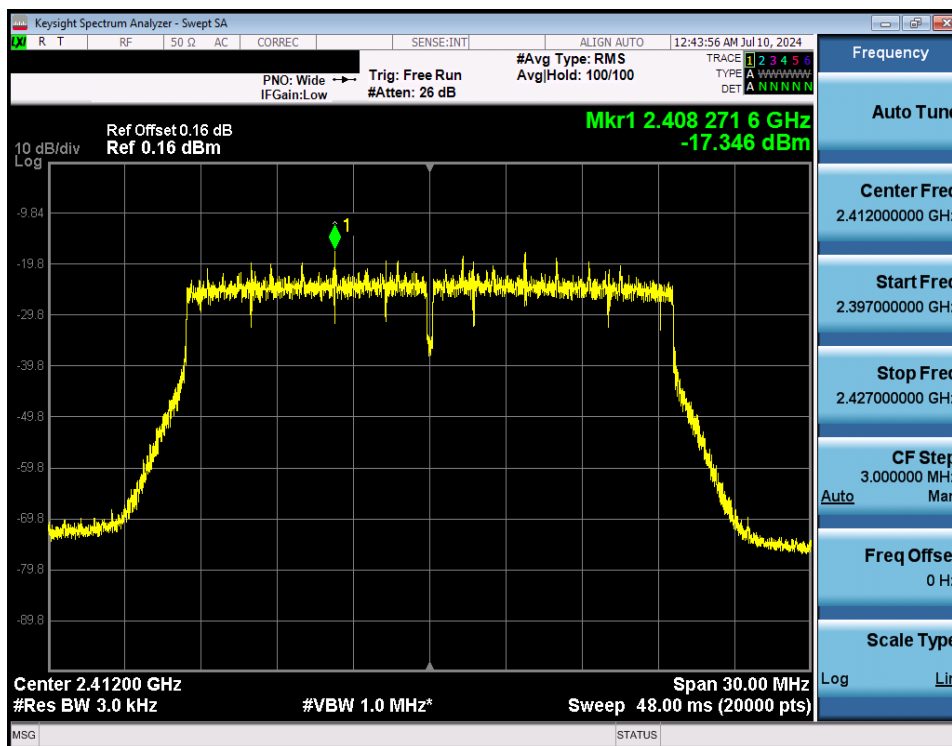
Plot 7-68. Power Spectral Density Plot Antenna WF7 (802.11ax OFDMA – RU242 – Ch. 1)
