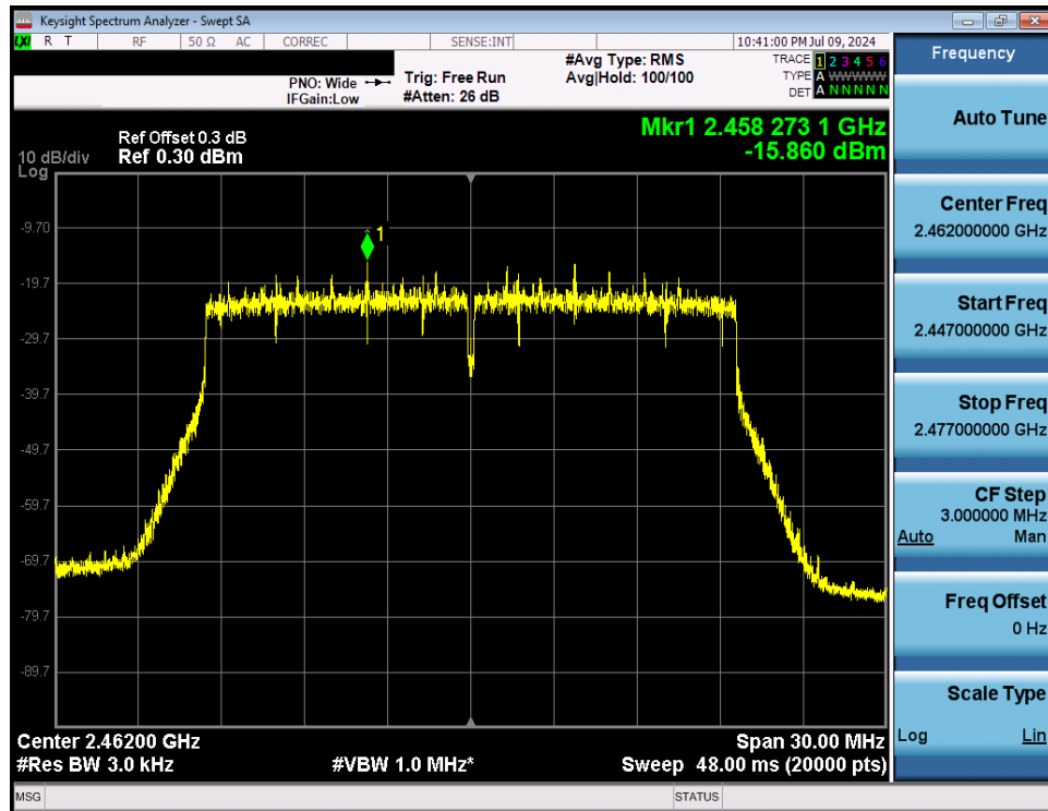
Plot 7-36. Power Spectral Density Plot Antenna WF8 (802.11ax OFDMA – RU242 – Ch. 11)
