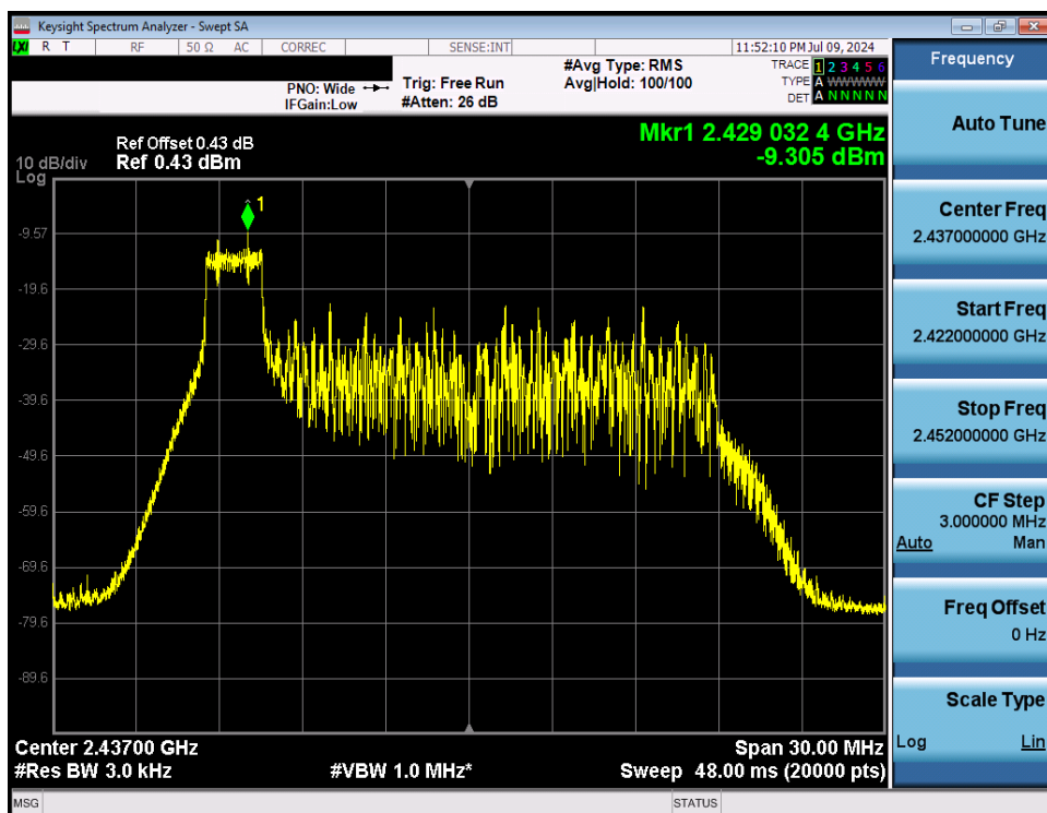
Plot 7-40. Power Spectral Density Plot Antenna WF7 (802.11ax OFDMA – RU26 Index 0 – Ch. 6)
