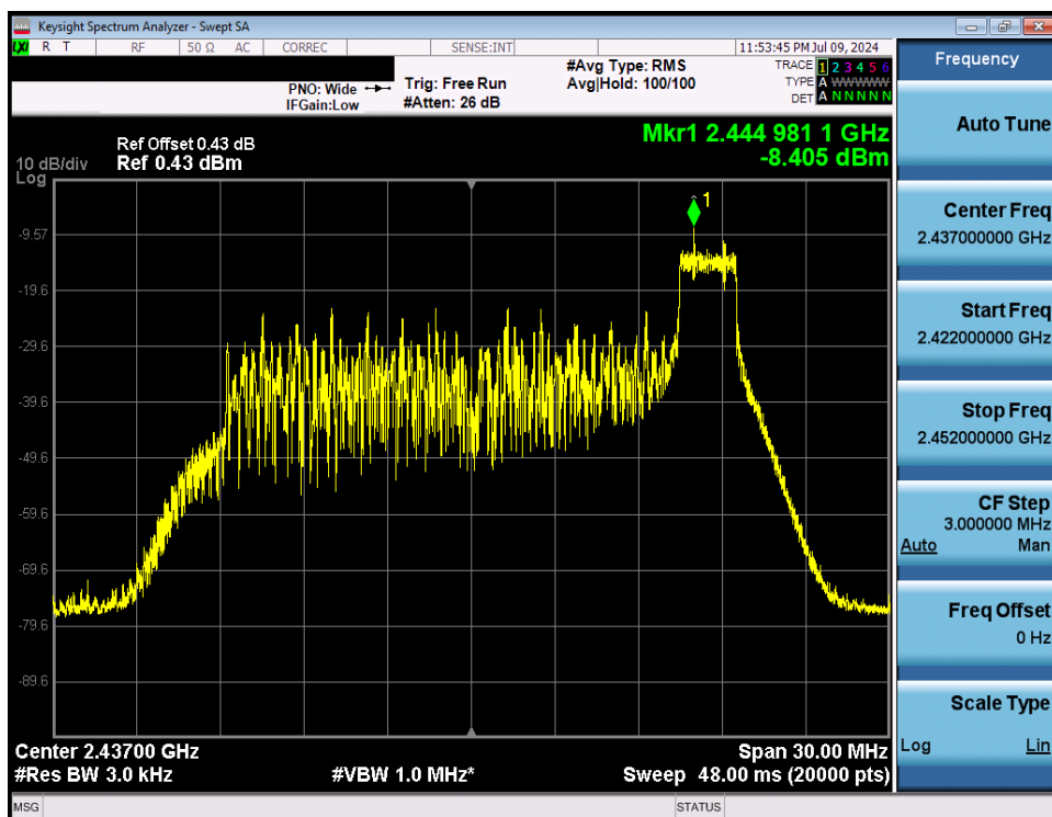
Plot 7-42. Power Spectral Density Plot Antenna WF7 (802.11ax OFDMA – RU26 Index 8 – Ch. 6)
