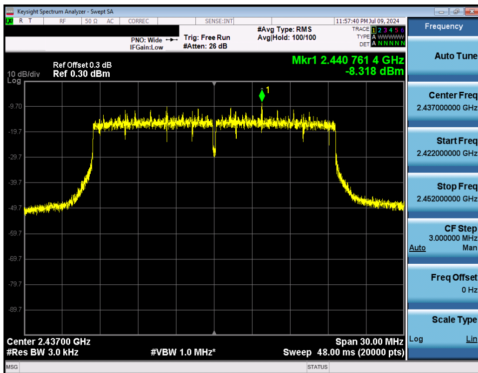
Plot 7-47. Power Spectral Density Plot Antenna WF7 (802.11ax OFDMA – RU242 – Ch. 6)
