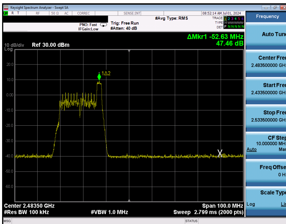
Plot 7-74. Band Edge Antenna WF8 (802.11ax OFDMA – RU26 Index 8 – Ch. 11)
