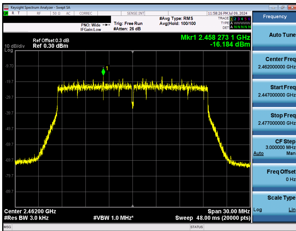
Plot 7-48. Power Spectral Density Plot Antenna WF7 (802.11ax OFDMA – RU242 – Ch. 11)
