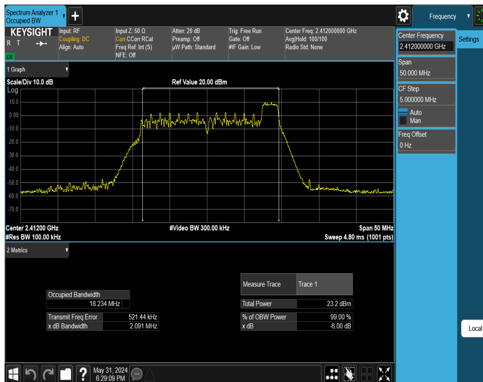
Plot 7-3. 6dB BW & 99% OBW Plot Antenna WF8 (802.11ax OFDMA – RU26 Index 8 – Ch. 1)
