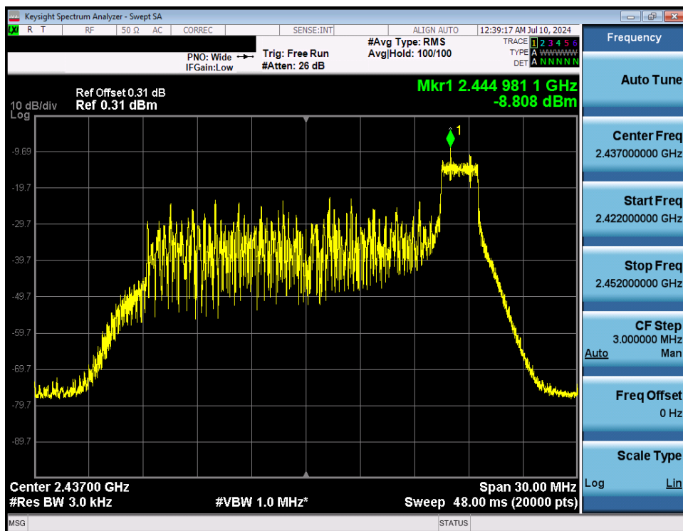
Plot 7-60. Power Spectral Density Plot Antenna WF7 (802.11ax OFDMA – RU26 Index 8 – Ch. 6)
