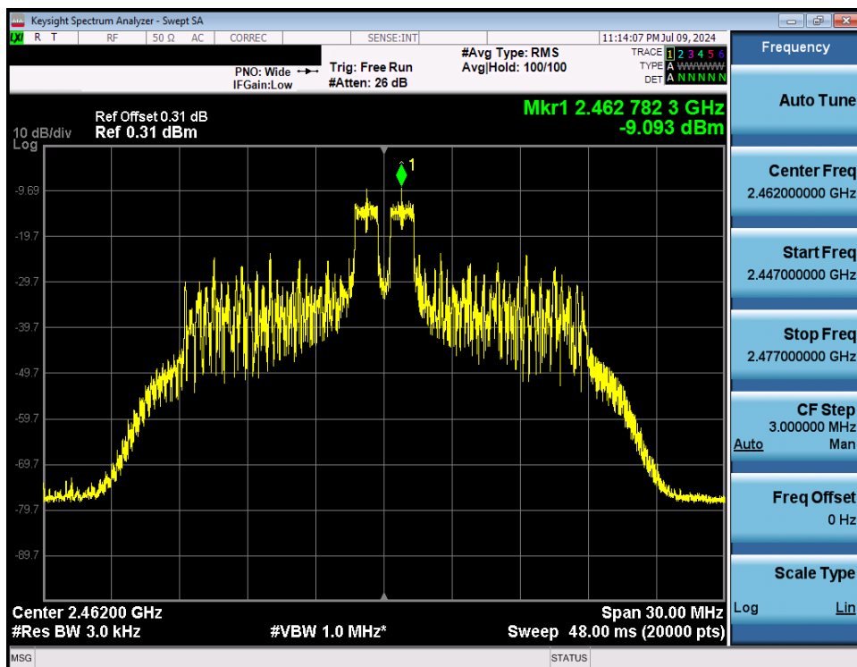
Plot 7-63. Power Spectral Density Plot Antenna WF8 (802.11ax OFDMA – RU26 Index 4 – Ch. 11)
