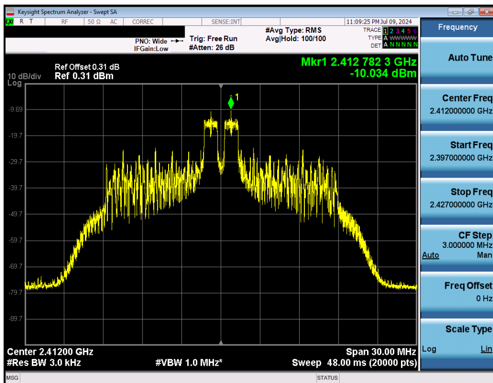
Plot 7-51. Power Spectral Density Plot Antenna WF8 (802.11ax OFDMA – RU26 Index 4 – Ch. 1)
