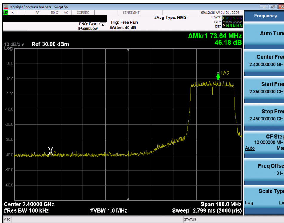
Plot 7-81. Band Edge Antenna WF8 (802.11ax OFDMA – RU242 – Ch. 6 Low)
