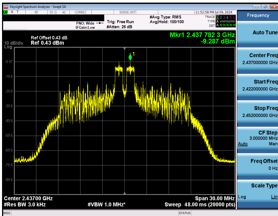
Plot 7-41. Power Spectral Density Plot Antenna WF7 (802.11ax OFDMA – RU26 Index 4 – Ch. 6)
