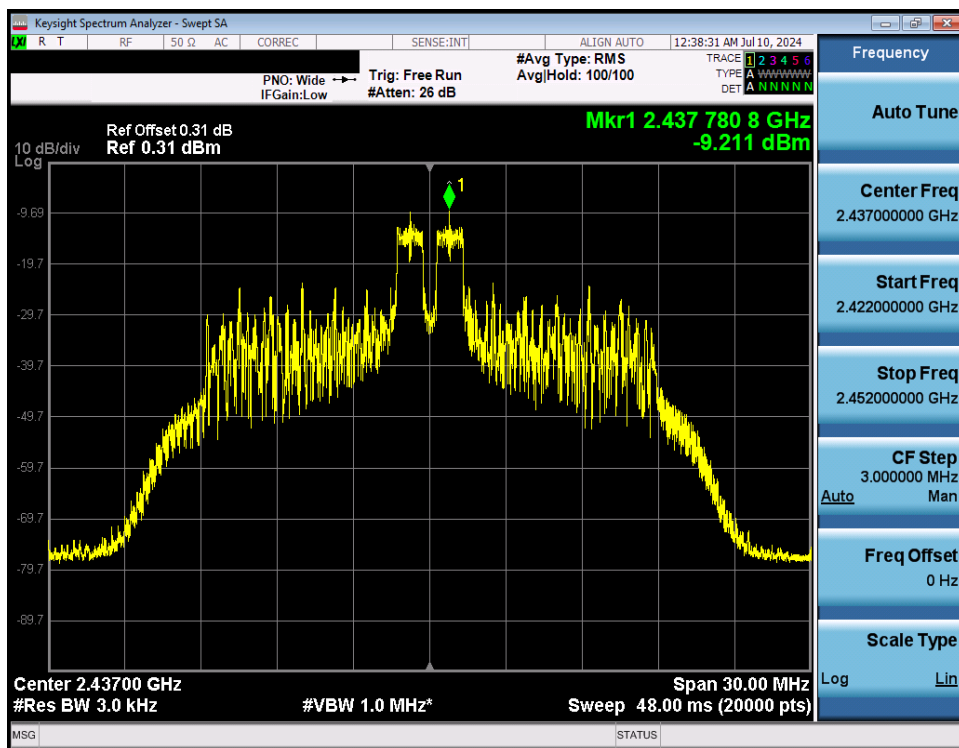
Plot 7-58. Power Spectral Density Plot Antenna WF7 (802.11ax OFDMA – RU26 Index 4 – Ch. 6)
