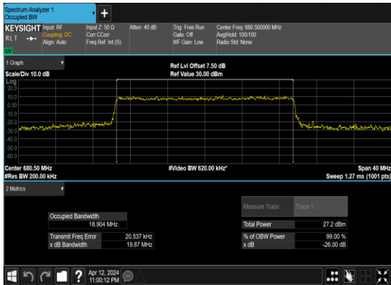
N71(20M)_CP-OFDM_16 QAM_Outer_Full_Mid_CH
