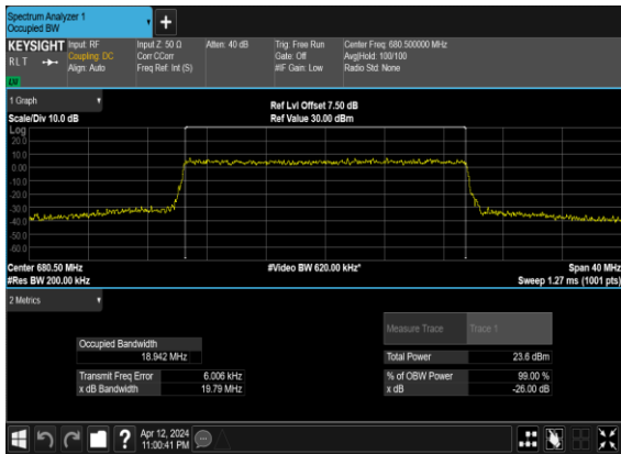
N71(20M)_CP-OFDM_256 QAM_Outer_Full_Mid_CH
