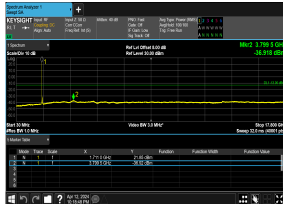
B5_N66(45M)_DFT-s- OFDM_QPSK_Edge_1RB_Left_Low_CH
