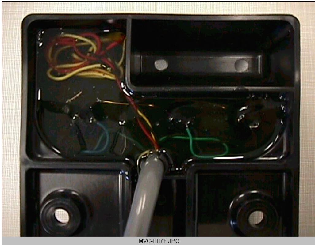
Strattec - Ignition Reader, Interconnect wiring
