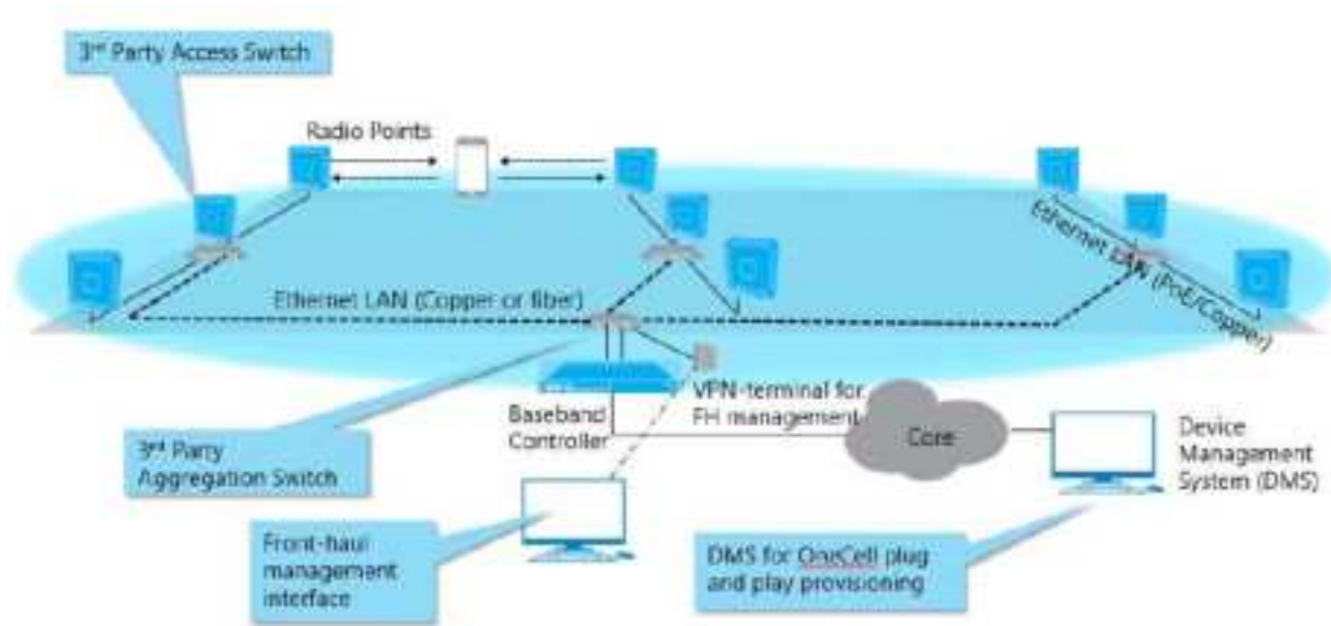
Figure 1-1. ONECELL solution
