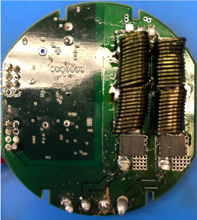
Amplifier PCB Back:
