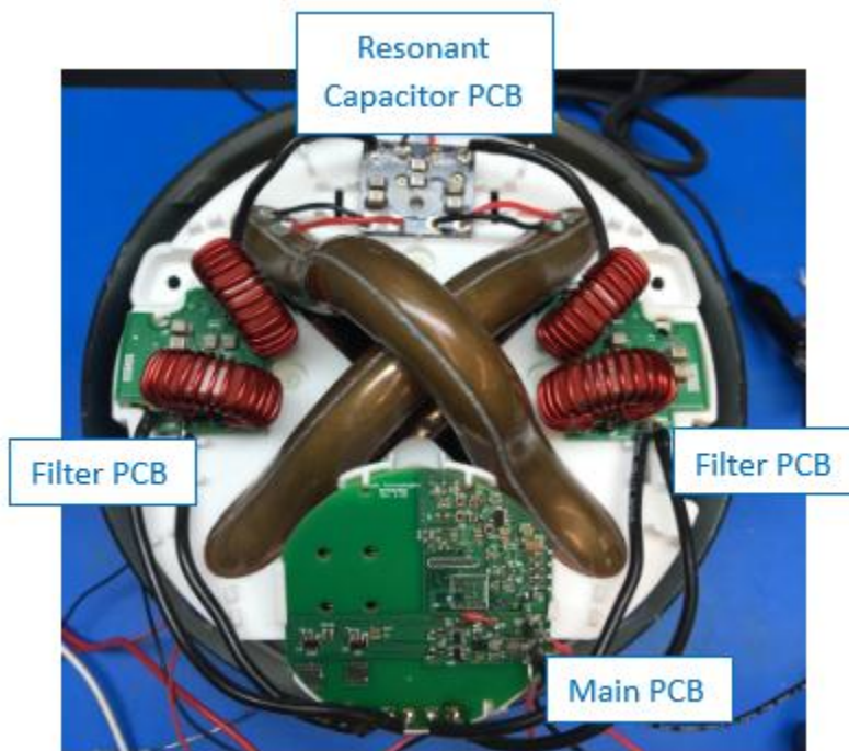
MotherBox Internal PCB Assembly Photo 2:
