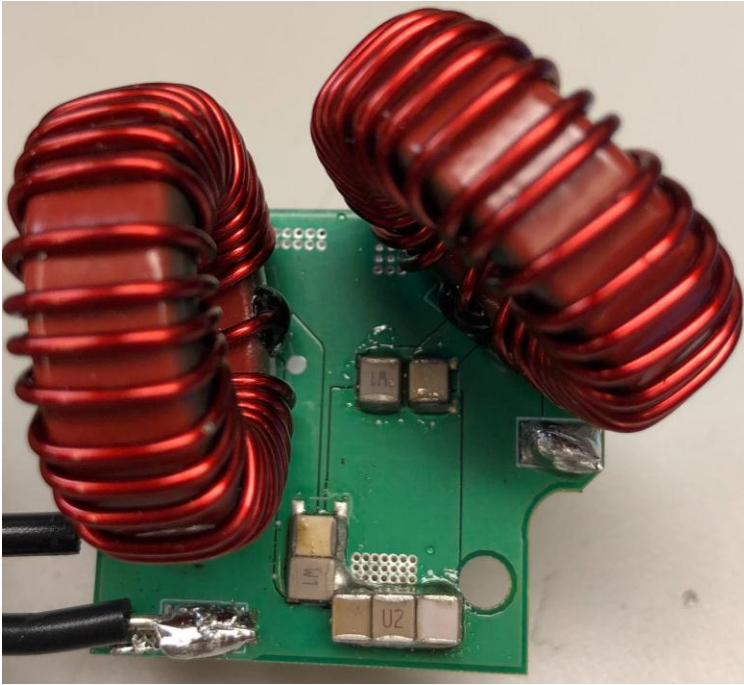
Second Filter Front:
