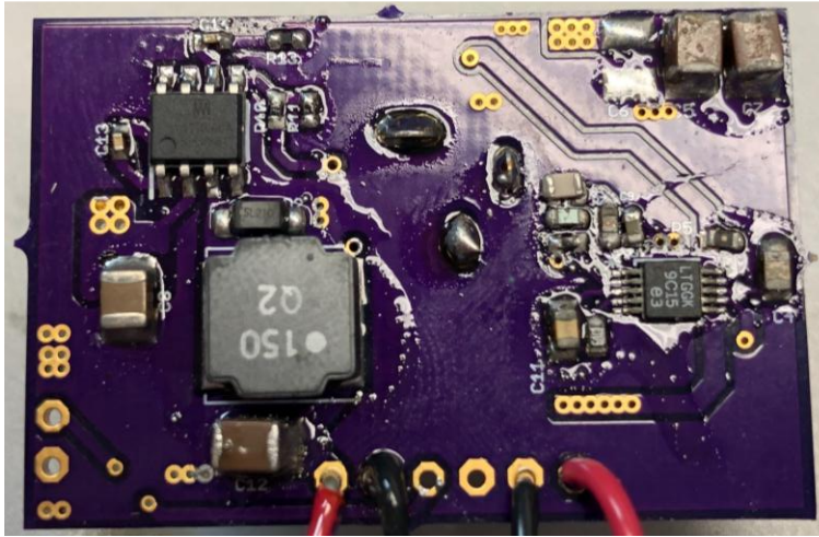
Back of Power PCB (DC input jack PCB):
